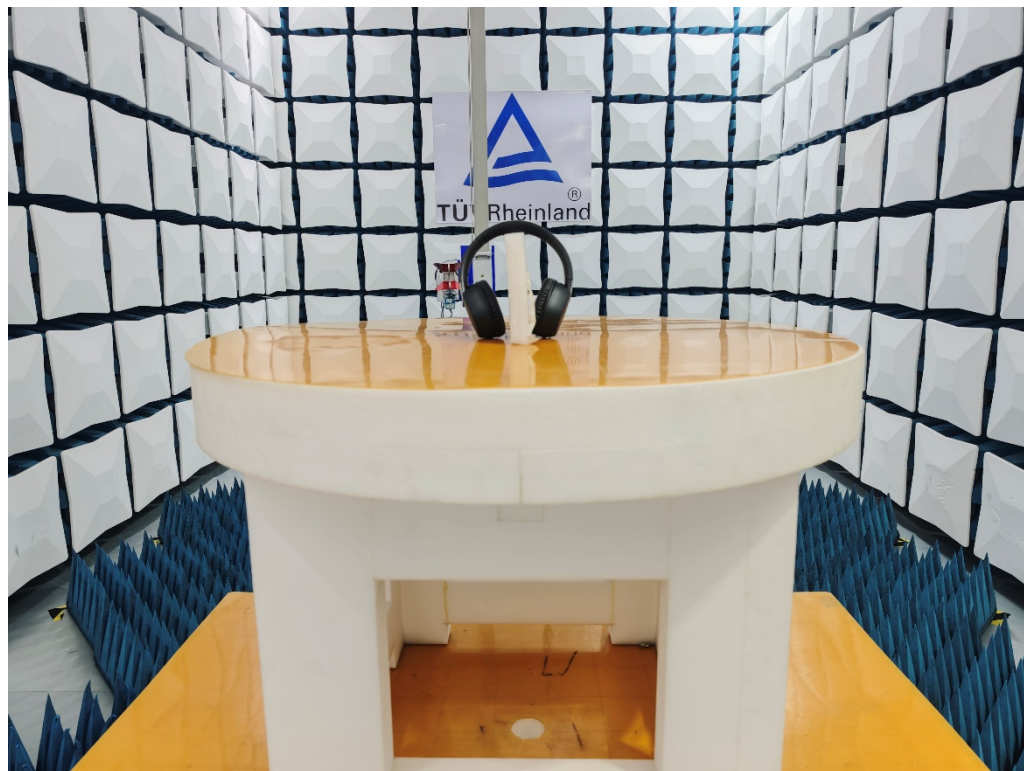
Photograph 2: Set-up photo for Radiated Spurious Emission, above 1G
