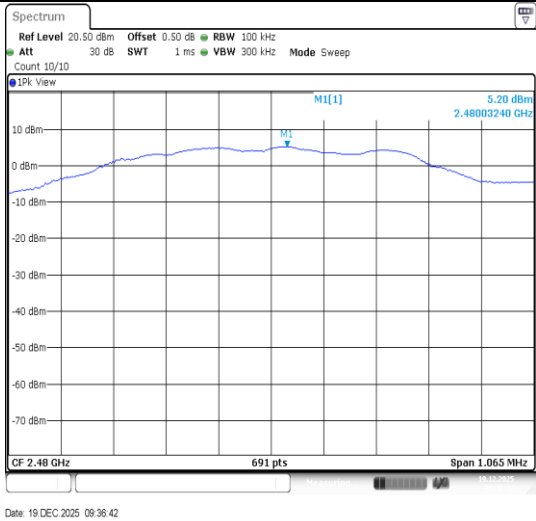
SRD-Ant1-2480-PASS
