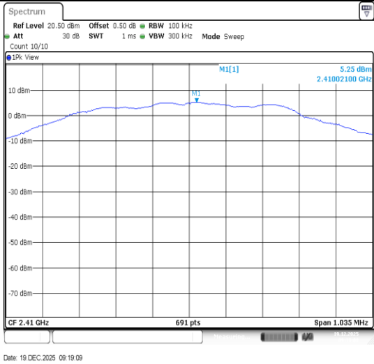
SRD-Ant1-2410-PASS
