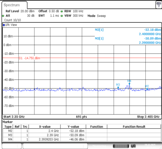
SRD-Ant1-2410-PASS
