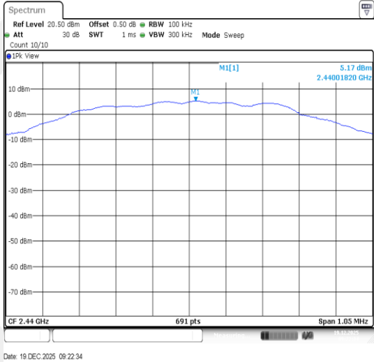
SRD-Ant1-2440-PASS
