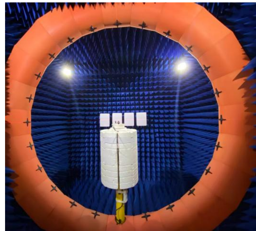
Testing 3D microwave darkroom(3m*3m*3m)
