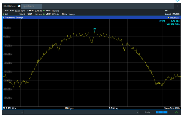
802.11b on Channel 11
