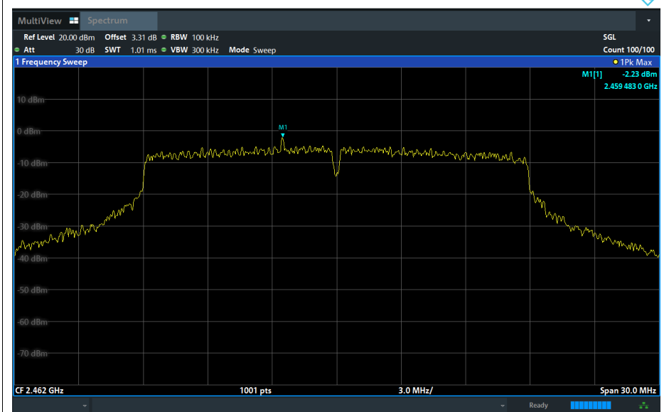
Band Edge NVNT n20 2462MHz Ant1 Emission
