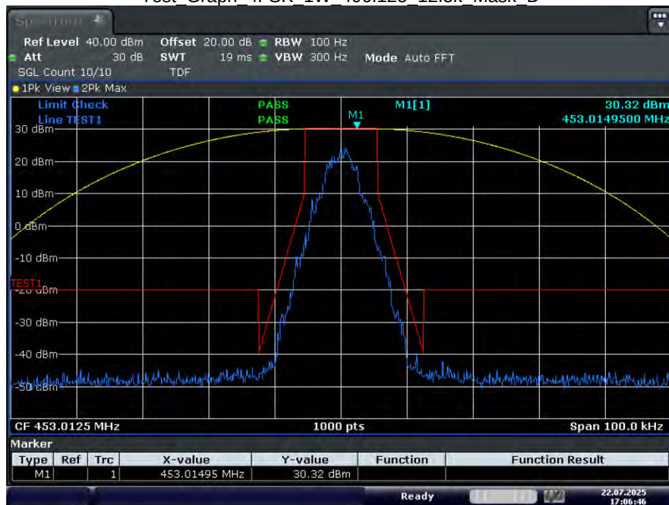
Test_Graph_4FSK_1W_453.0125_12.5k_Mask_D
