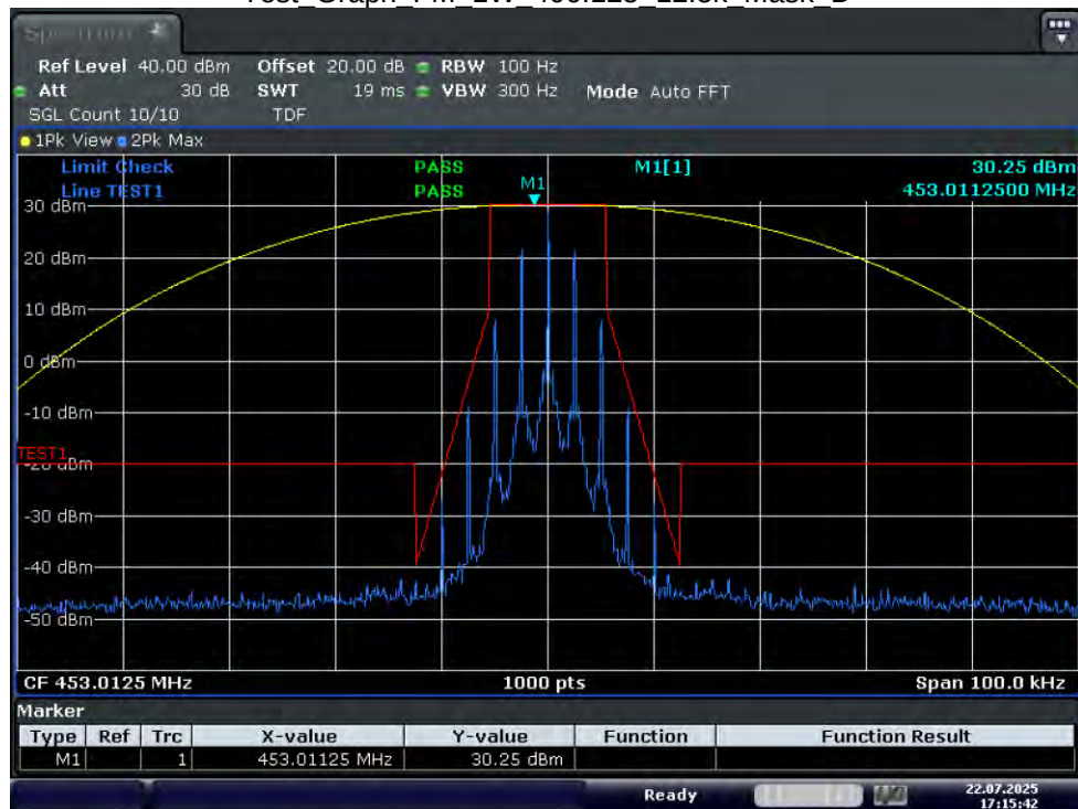
Test_Graph_FM_1W_453.0125_12.5k_Mask_D
