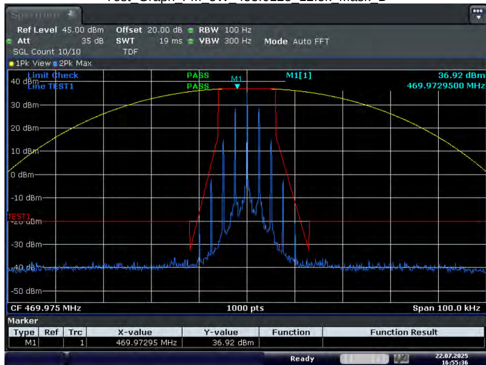
Test_Graph_FM_5W_469.975_12.5k_Mask_D
