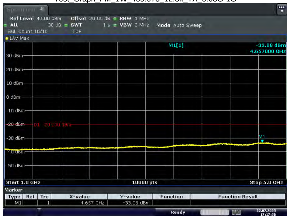
Test_Graph_FM_1W_469.975_12.5k_TX_1G-5G
