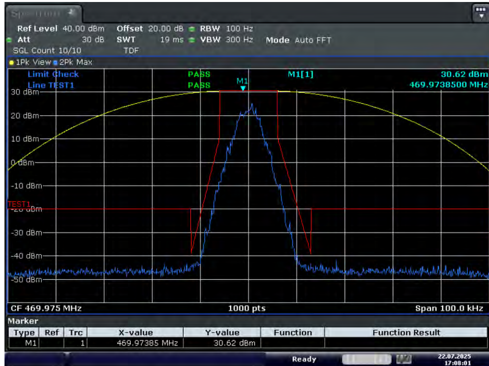
Test Graph 4FSK 1W 469.975 12.5k Mask D
