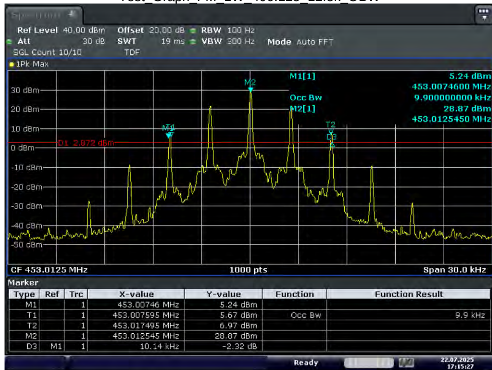
Test_Graph_FM_1W_453.0125_12.5k_OBW
