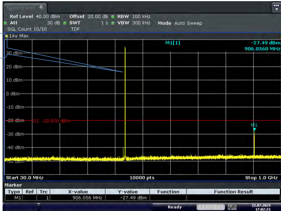
Test Graph 4FSK 5W 453.0125 12.5k TX 0.03G-1G
