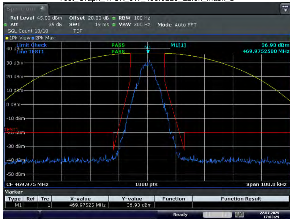
Test_Graph_4FSK_5W_469.975_12.5k_Mask_D
