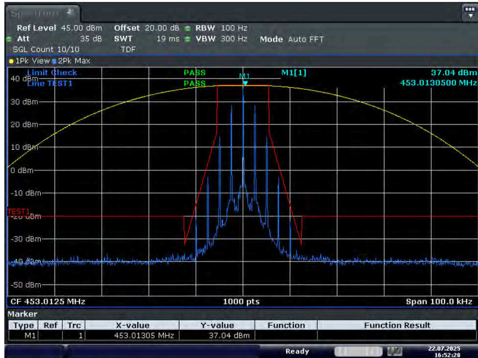
Test Graph FM 5W 453.0125 12.5k Mask D
