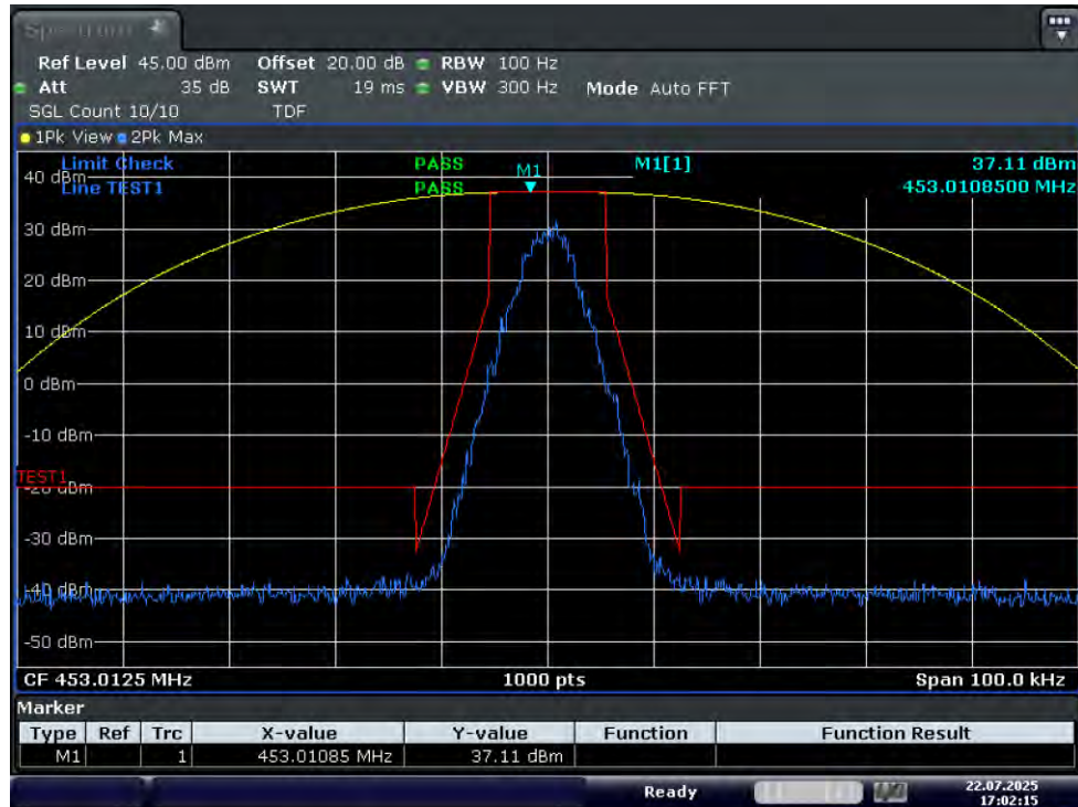
Test Graph 4FSK 5W 453.0125 12.5k Mask D
