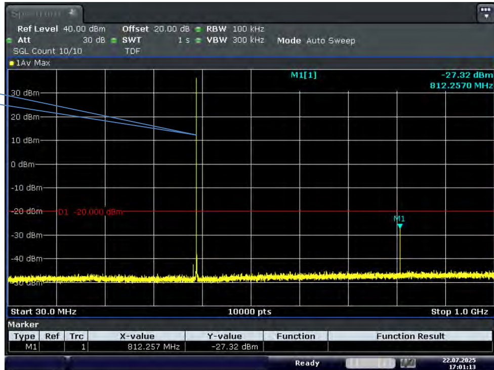
Test Graph 4FSK 5W 406.125 12.5k TX 0.03G-1G
