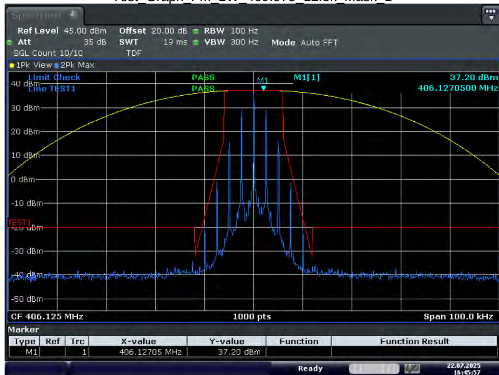
Test_Graph_FM_5W_406.125_12.5k_Mask_D
