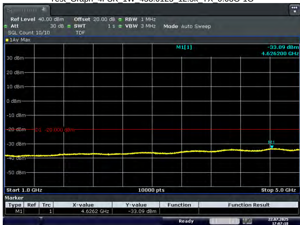
Test_Graph_4FSK_1W_453.0125_12.5k_TX_1G-5G
