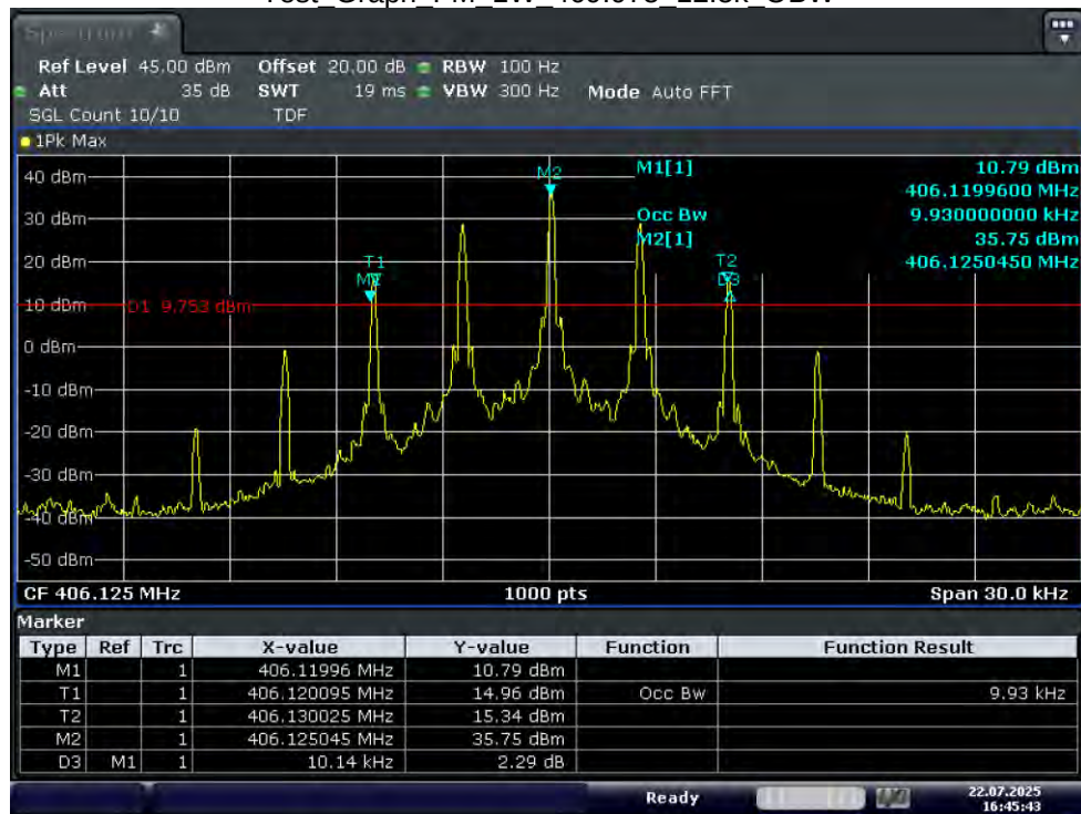
Test_Graph_FM_5W_406.125_12.5k_OBW
