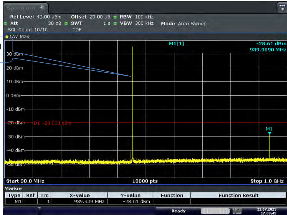
Test Graph 4FSK 5W 469.975 12.5k TX 0.03G-1G
