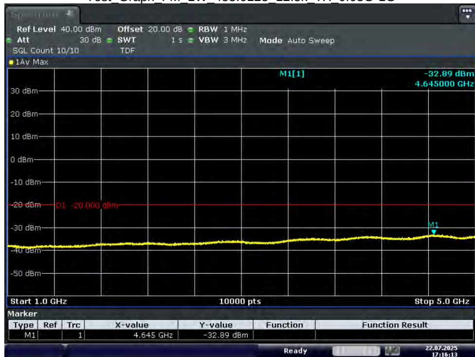
Test_Graph_FM_1W_453.0125_12.5k_TX_1G-5G
