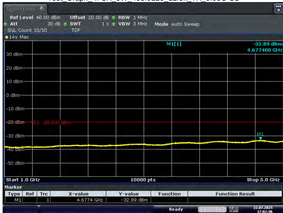
Test_Graph_4FSK_5W_453.0125_12.5k_TX_1G-5G
