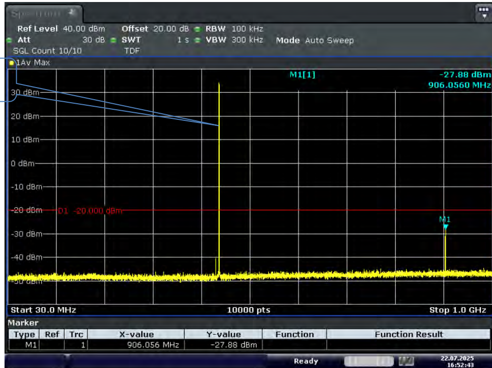
Test Graph FM 5W 453.0125 12.5k TX 0.03G-1G
