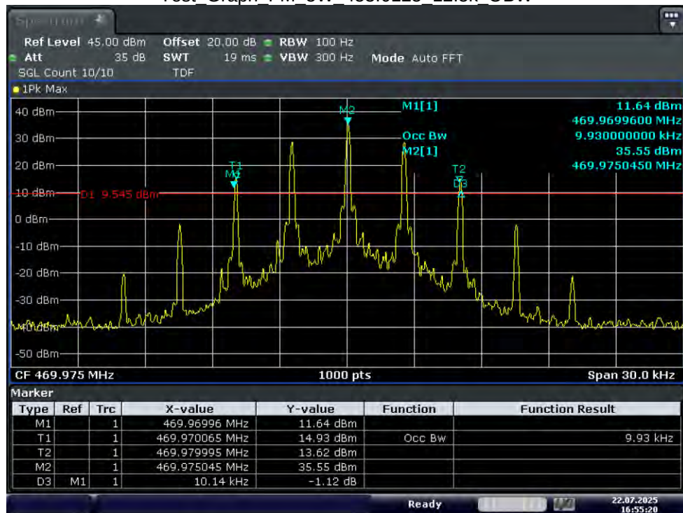
Test_Graph_FM_5W_469.975_12.5k_OBW
