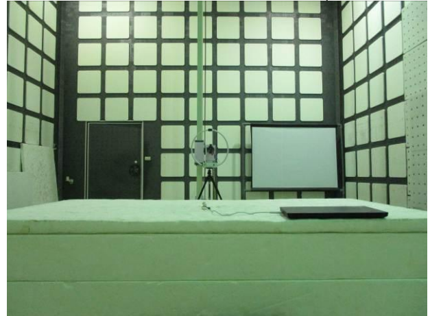
FCC_15_247_BLE_Radiated_L_Setup
