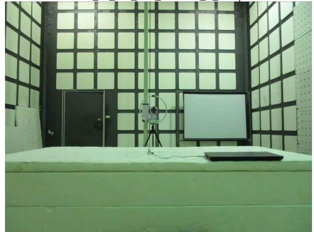
FCC_15_247_BLE_Radiated_R_Setup
