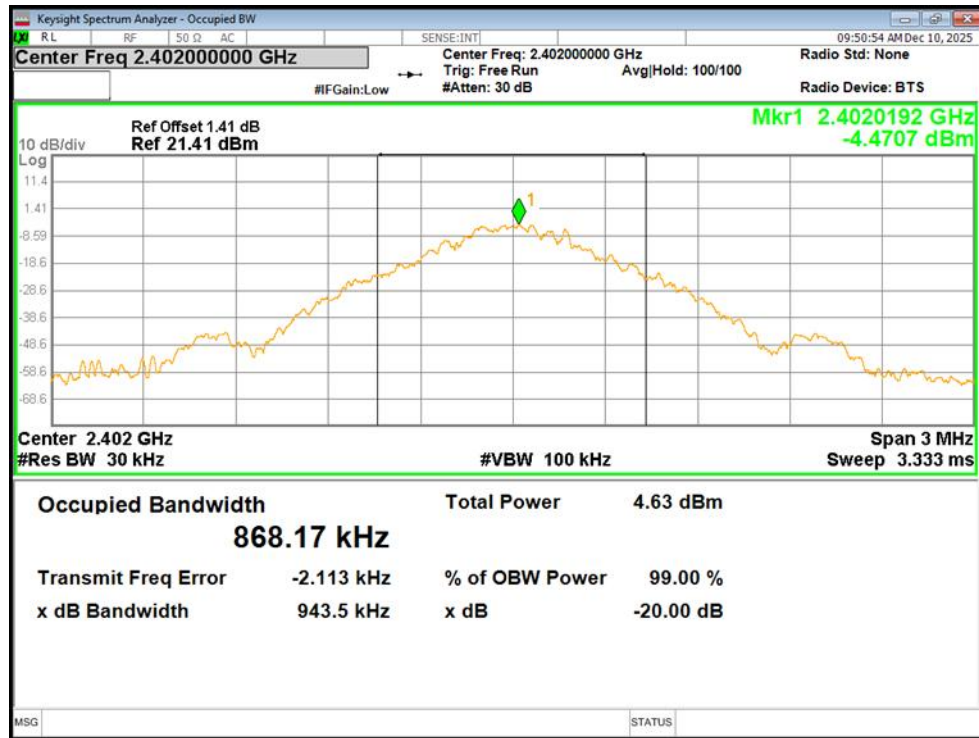
99%_Occupied_Bandwidth_NVNT_ANT1_1-DH5_2402_00
