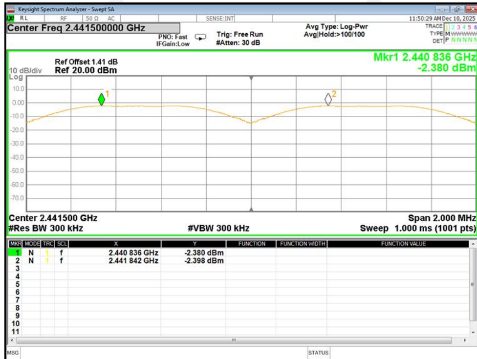
Carrier_Frequencies_Separation_(Hopping)_NVNT_ANT5_1-DH5_Hopping
