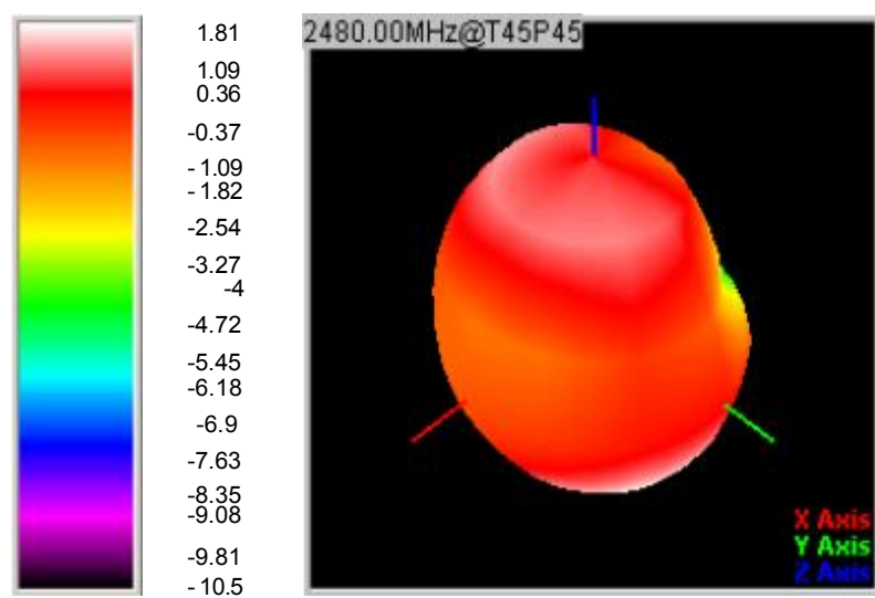
◎ 3D Gain Pattern (2480 MHz)
