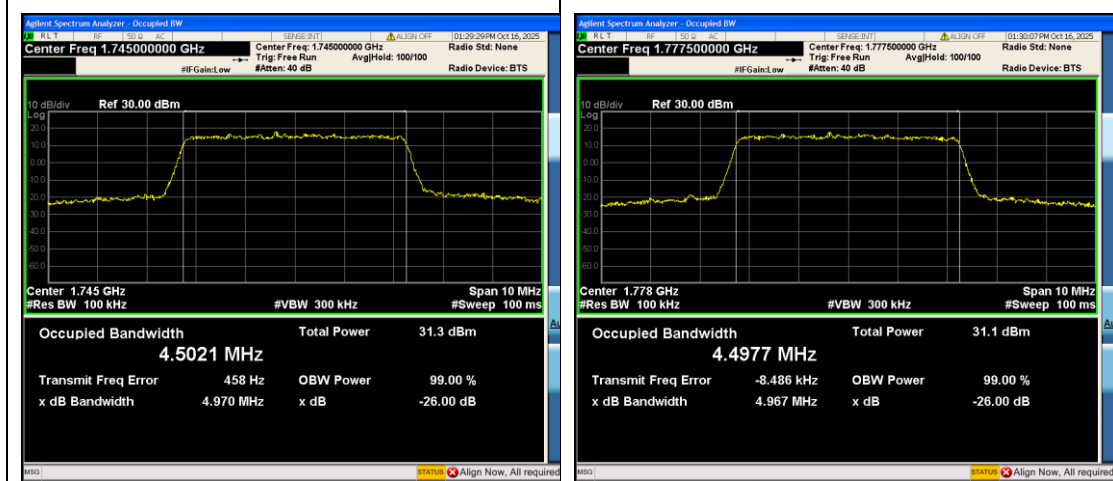
Band66-5MHz-16QAM-132322-25RB#0-PASS
