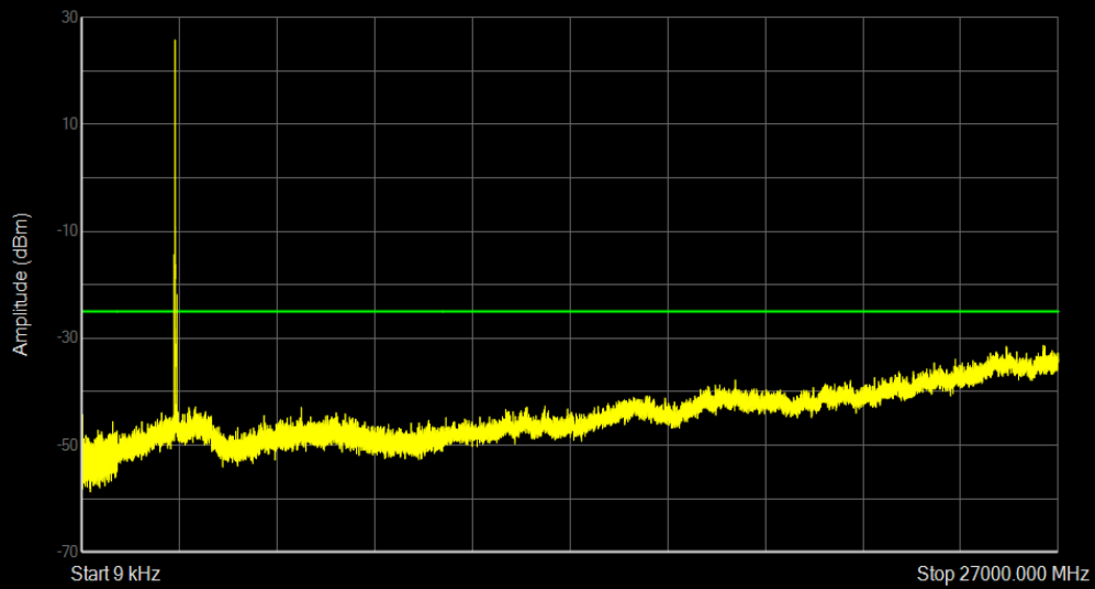
Band41(2535-2655) QPSK BW=5MHz Channel=40640 RB Size=1 Position=#0
