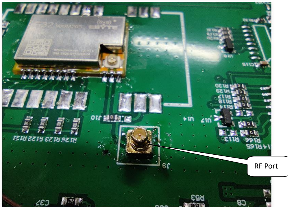
ANTENNA VIEW OF EUT (FIGURE 1)
