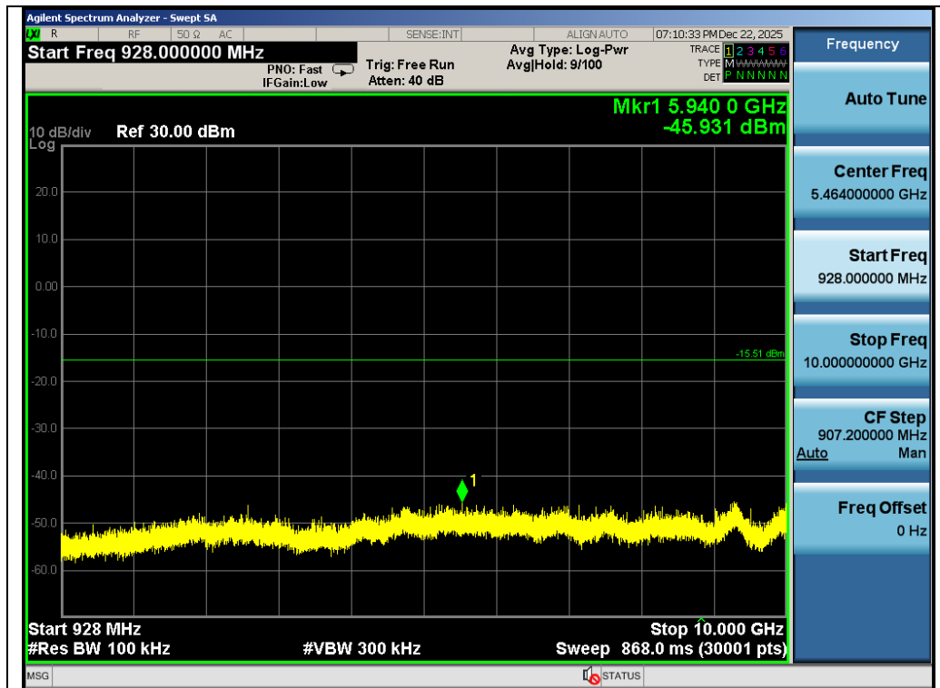
Test_Graph_LoRa_903.00MHz_Frequency Band 2
