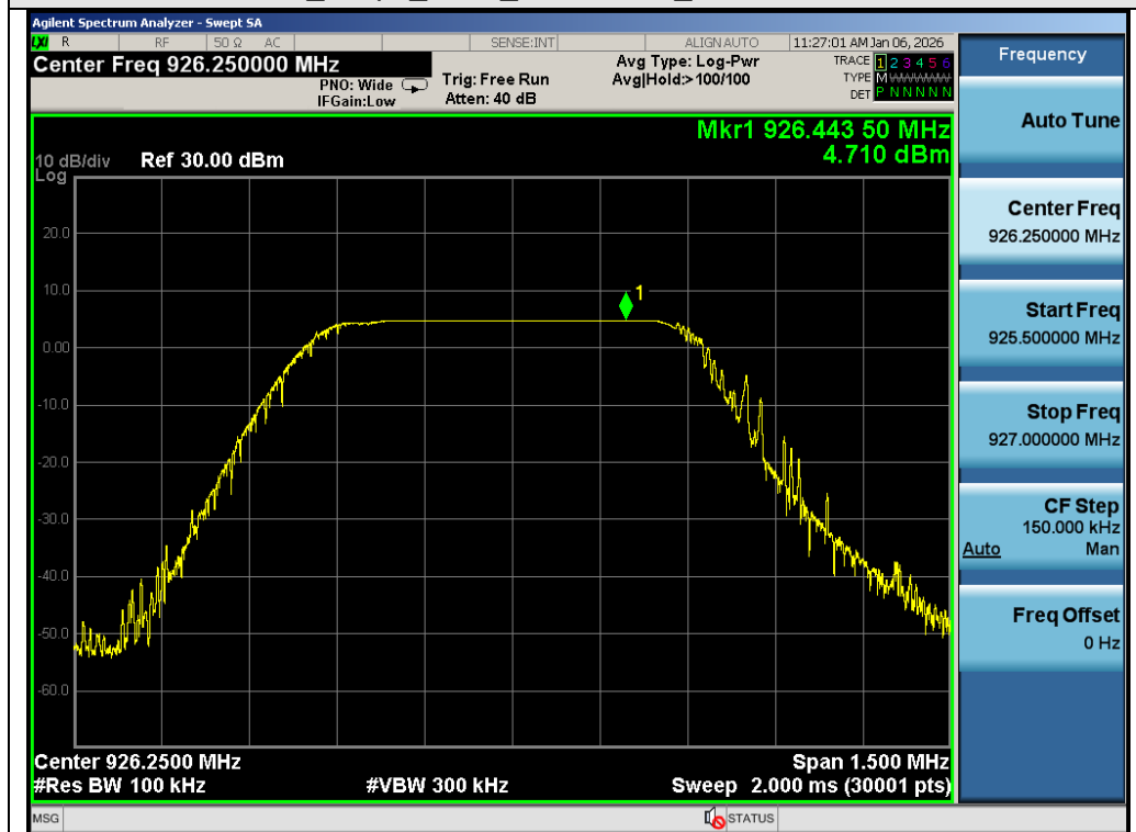
Test_Graph_LoRa_926.25MHz_Frequency Band 1
