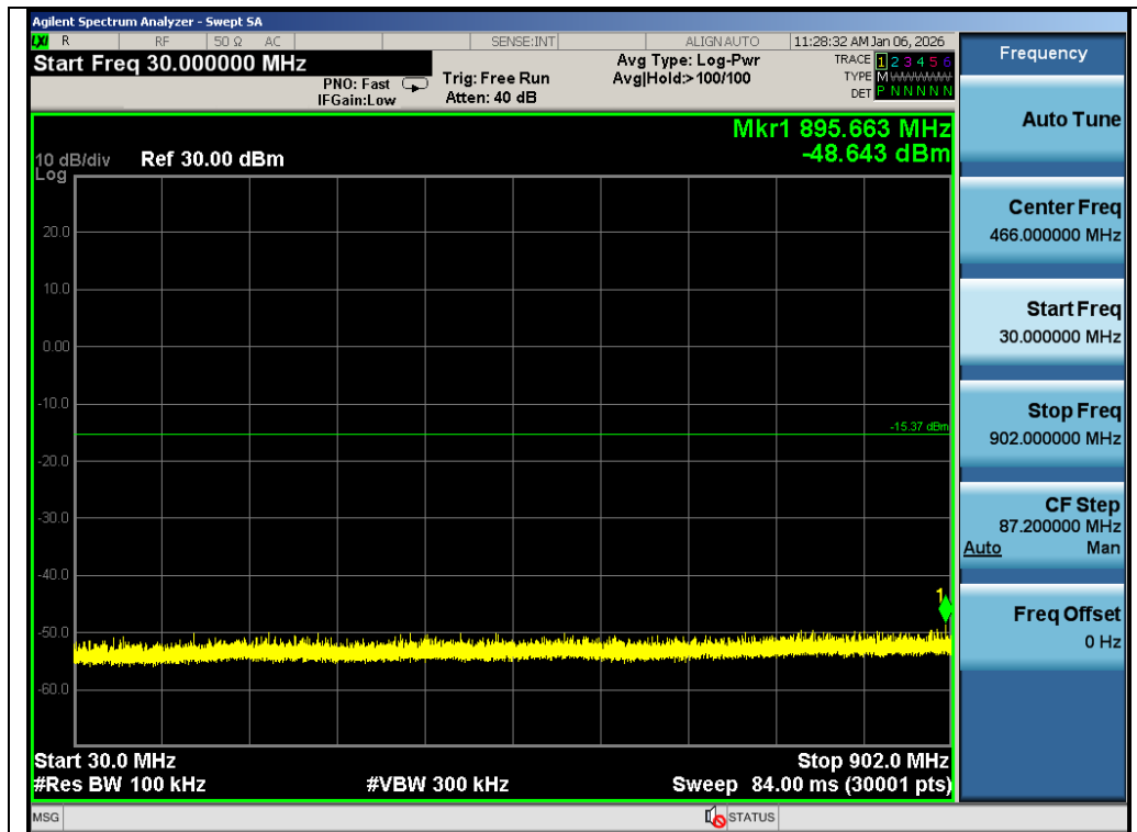
Test_Graph_LoRa_915.00MHz_Frequency Band 1
