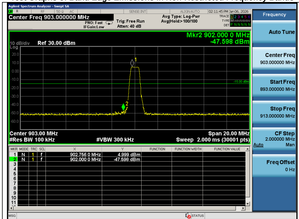
Test_Graph_LoRa_903.00MHz_Lower Band Edge Emissions
