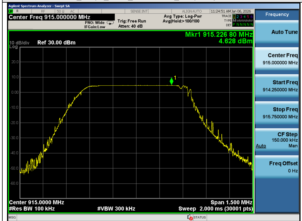
Test_Graph_LoRa_915.00MHz_Reference level
