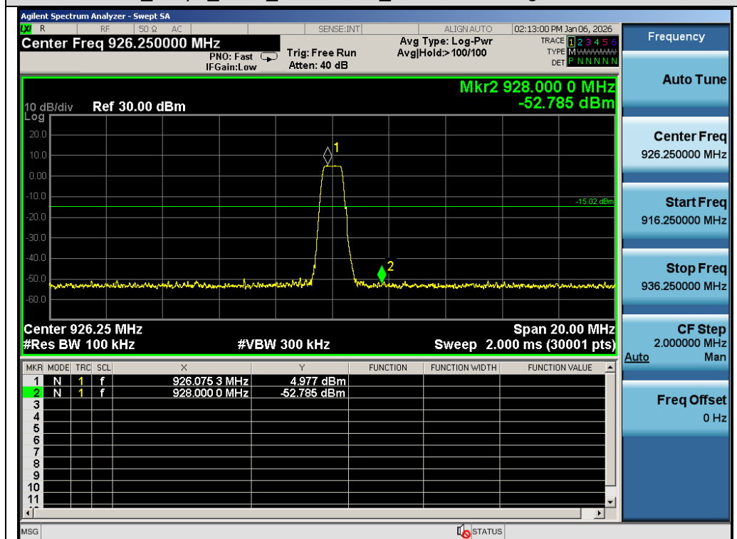
Test_Graph_LoRa_926.25MHz_Higher Band Edge Emissions
