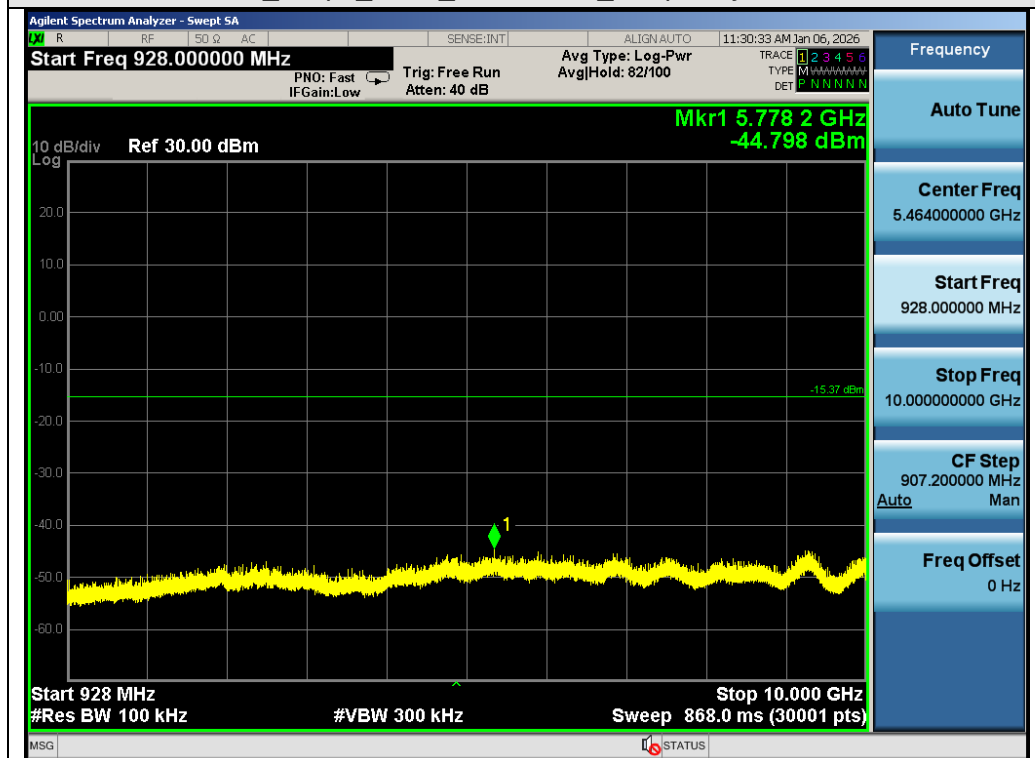
Test_Graph_LoRa_915.00MHz_Frequency Band 2
