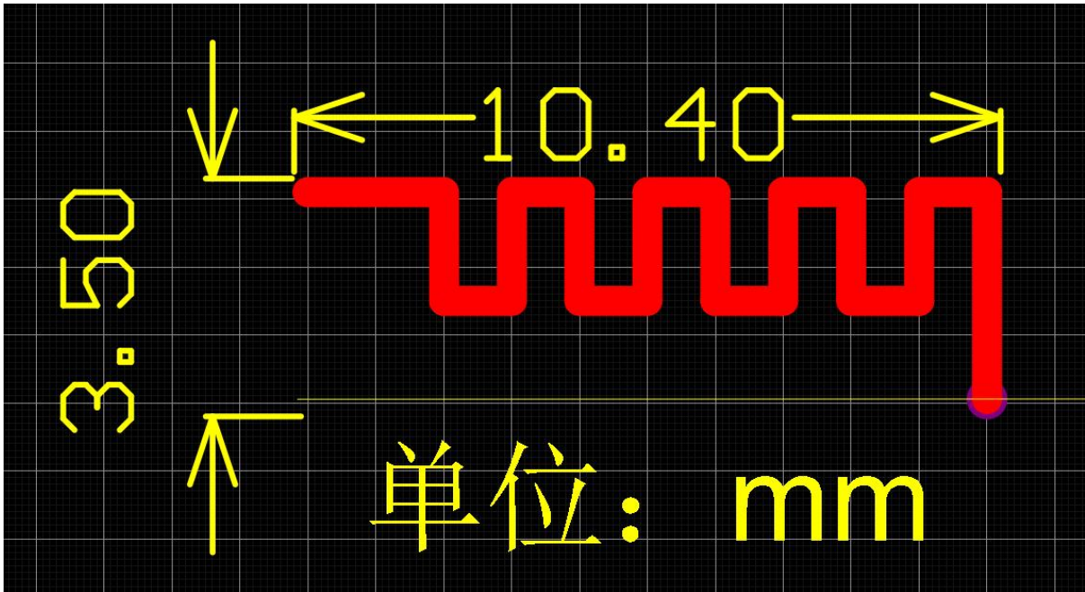
Antenna Photo & Length (mm)
