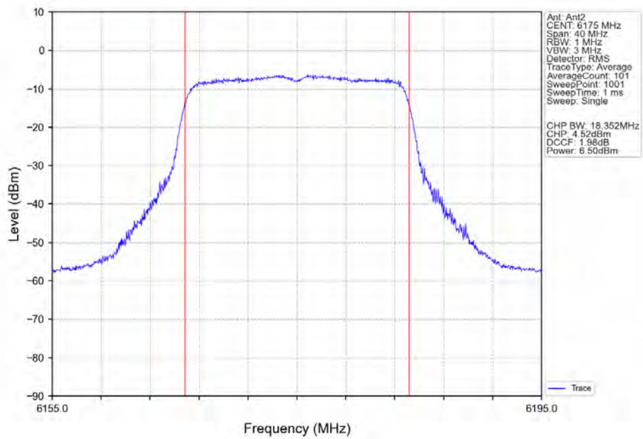
802.11ac(VHT20) MCH 6175MHz Ant2 NTN
