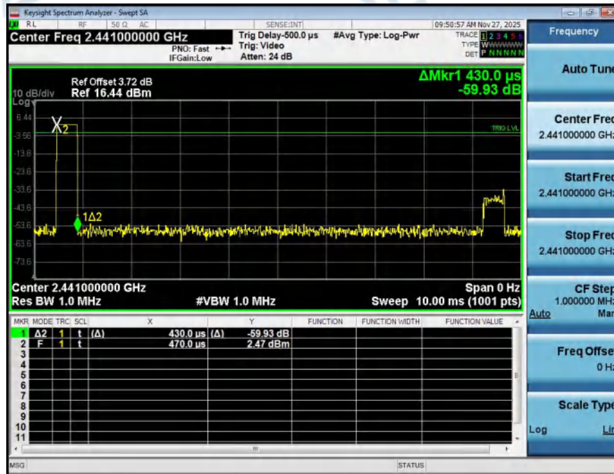
Dwell_Time_(Hopping)_NVNT_ANT1_1-DH1_2441_00_One_Burst_Time
