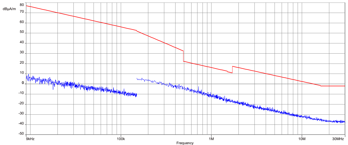
Plot 4: 9 kHz to 30 MHz, 913.6 MHz, ISED
