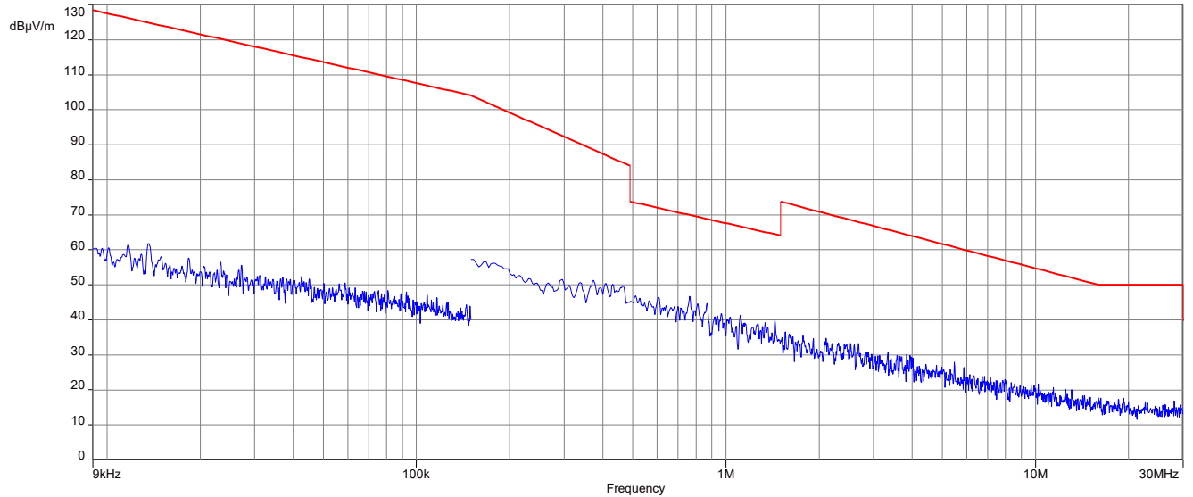
Plot 5: 9 kHz to 30 MHz, 926.0 MHz, FCC
