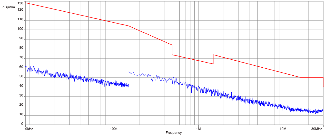
Plot 3: 9 kHz to 30 MHz, 913.6 MHz, FCC
