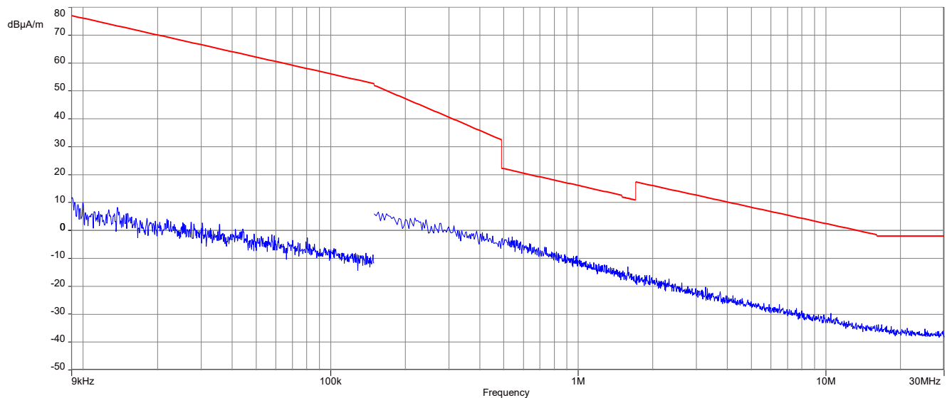
Plot 6: 9 kHz to 30 MHz, 926.0 MHz, ISSED
