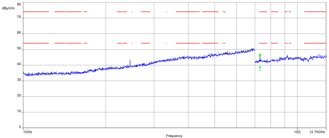
Plot 2: 1 GHz to 12.75 GHz, vertical & horizontal polarization, 913.6 MHz
