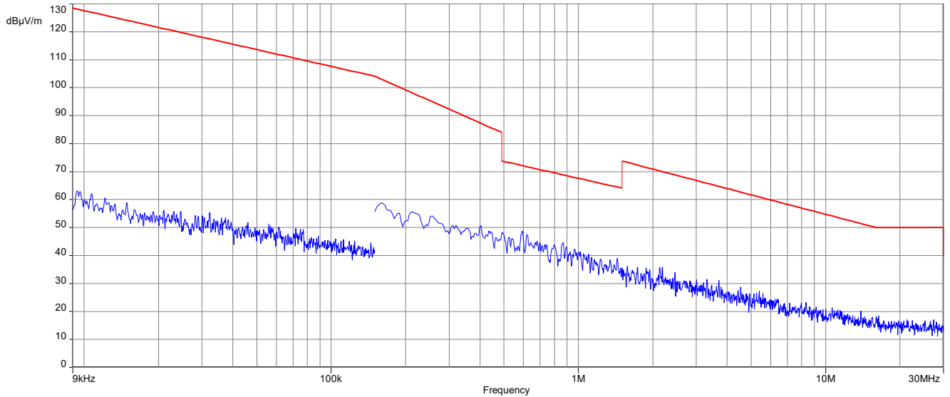
Plot 1: 9 kHz to 30 MHz, 905.5 MHz FCC
