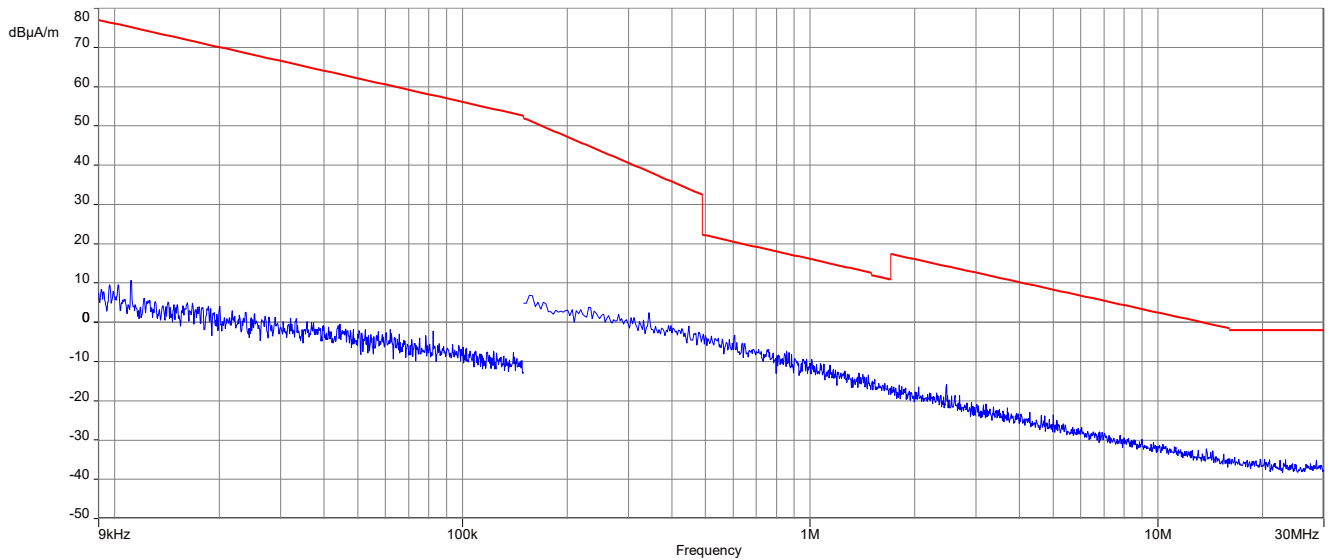
Plot 2: 9 kHz to 30 MHz, 905.5 MHz ISED
