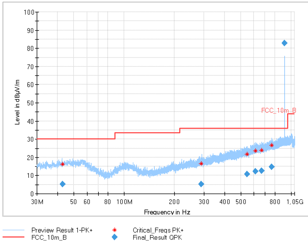
Plot 2: 30 MHz to 1 GHz, vertical & horizontal polarization, 913.6 MHz
