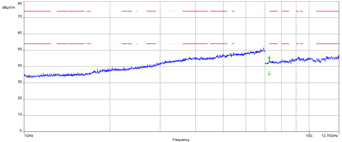
Plot 1: 1 GHz to 12.75 GHz, vertical & horizontal polarization, 905.5 MHz
