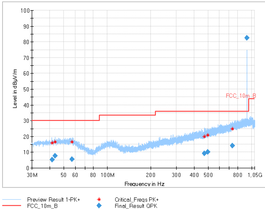
Plot 3: 30 MHz to 1 GHz, vertical & horizontal polarization, 926.0 MHz
