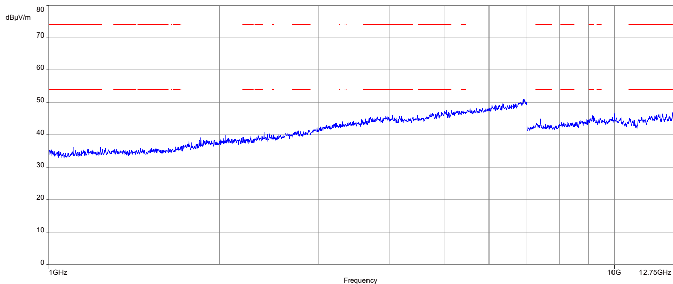
Plot 3: 1 GHz to 12.75 GHz, vertical & horizontal polarization, 926.0 MHz
