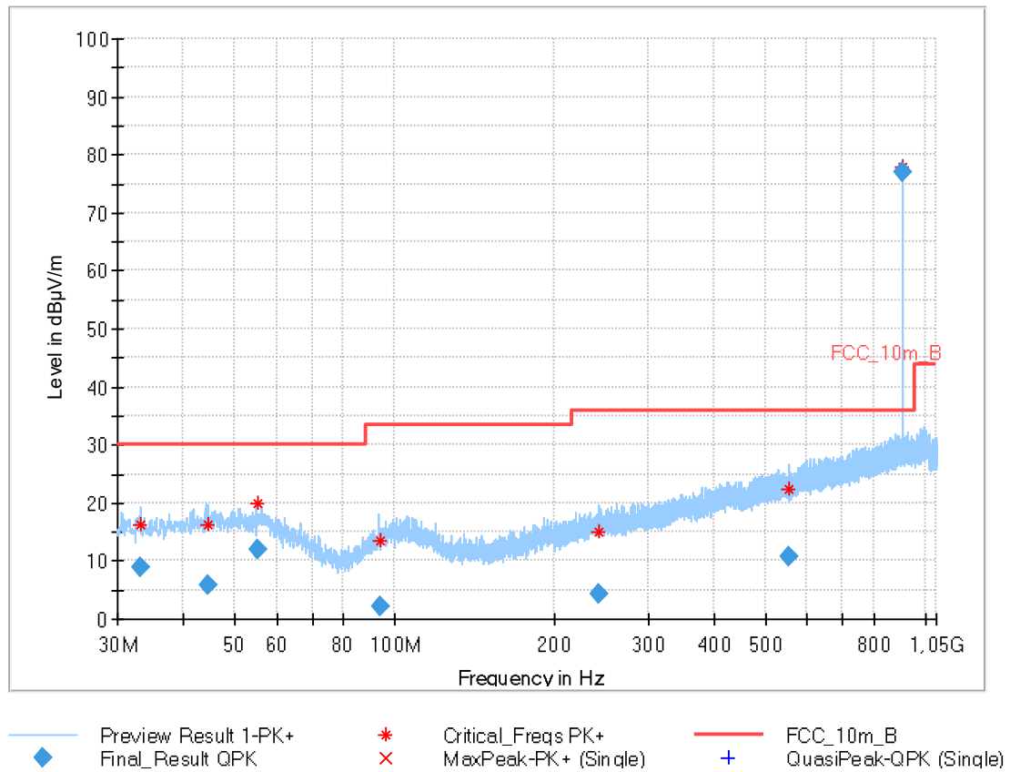
Plot 1: 30 MHz to 1 GHz, vertical & horizontal polarization, 905.5 MHz
