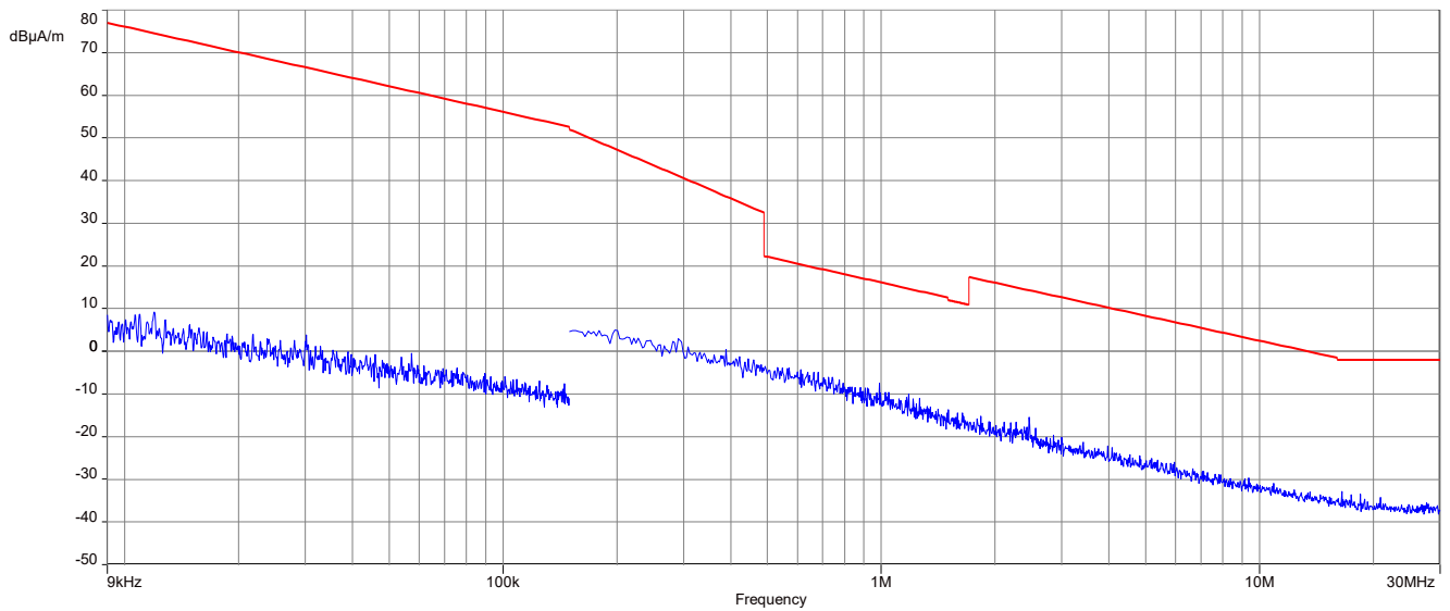
Plot 2: 9 kHz to 30 MHz, 905.5 MHz ISSED
