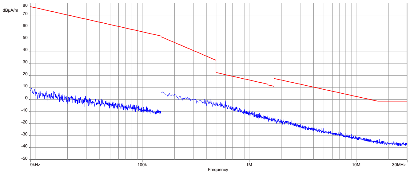
Plot 4: 9 kHz to 30 MHz, 913.6 MHz, ISSED
