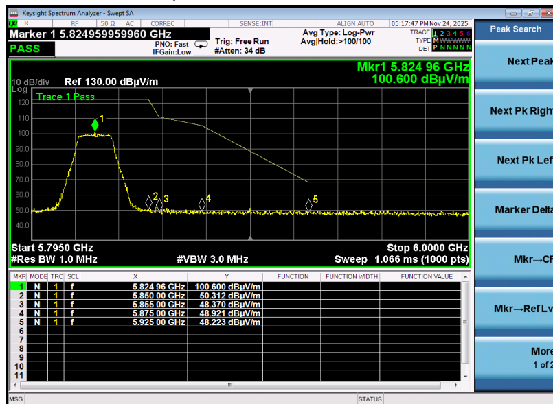
Test Graph for Peak Measurement- Vertical
