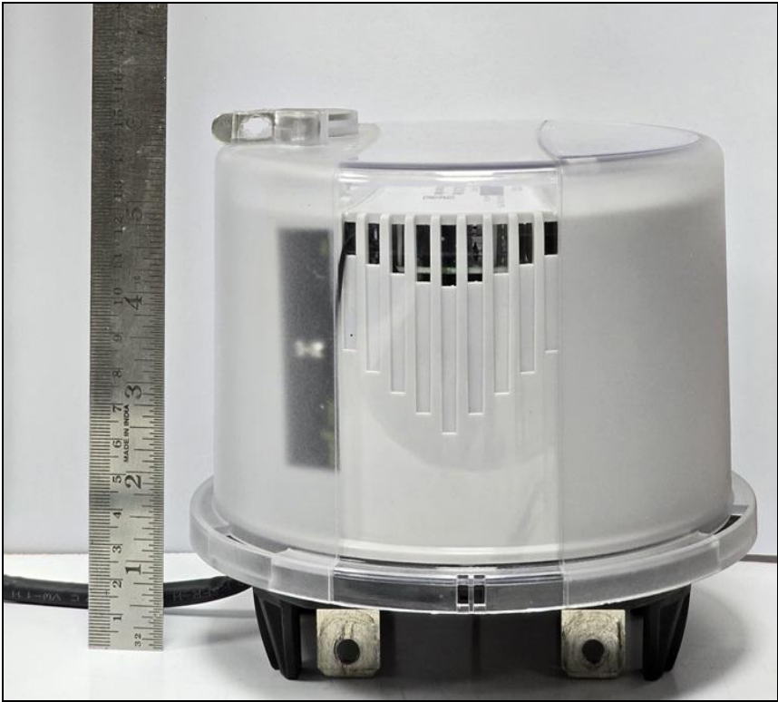
Photo 3: EUT With Dimension
