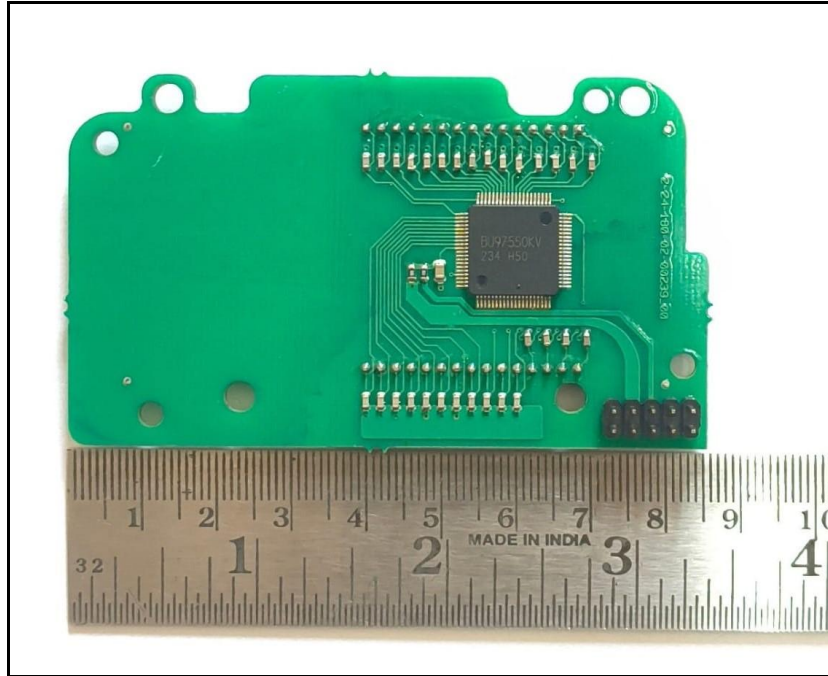
Photo 9: Display card with Dimension with rare view
