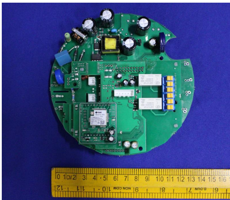
Photo 5: ANSI EM CPU with LORA MOD KYZ CARD Dimension View
