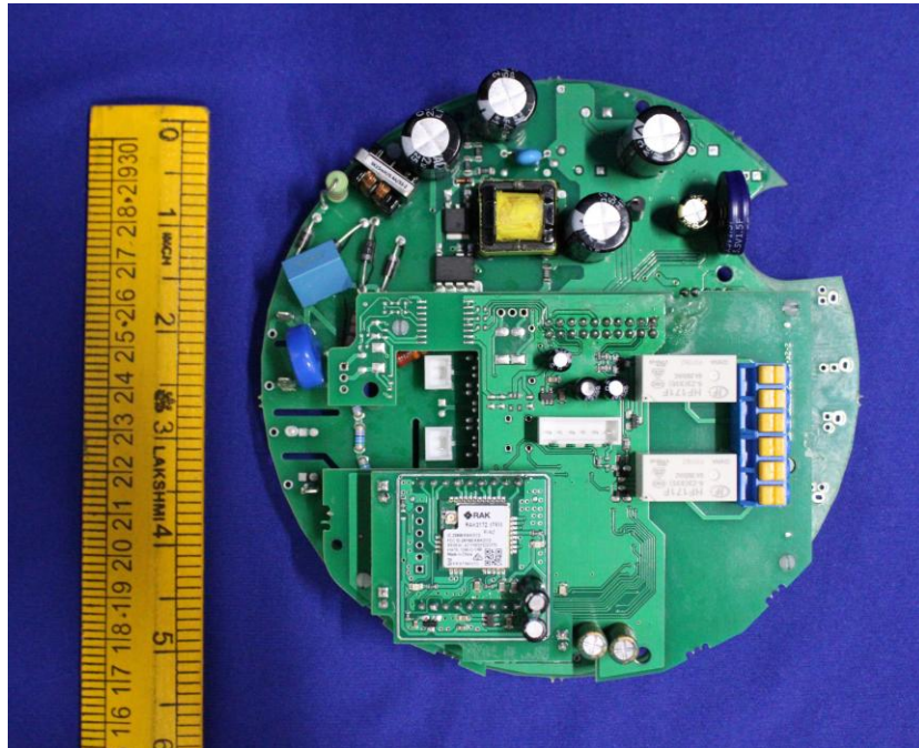
Photo 3: ANSI EM CPU with LORA MOD KYZ CARD Dimension View
