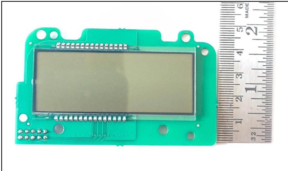
Photo 8: Display card with Dimension with front view
