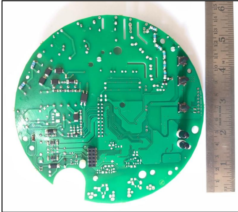
Photo 13: ANSI EM CPU Card rare view
