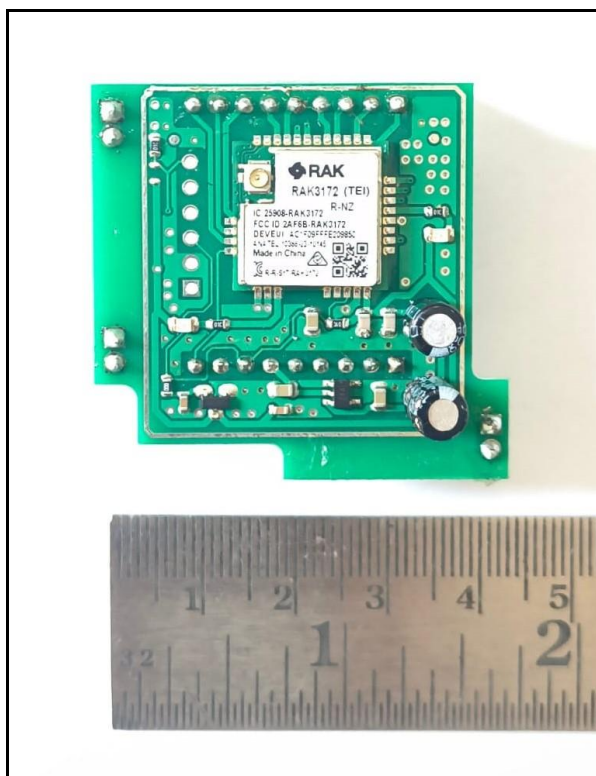
Photo 6: Module With Dimensions
