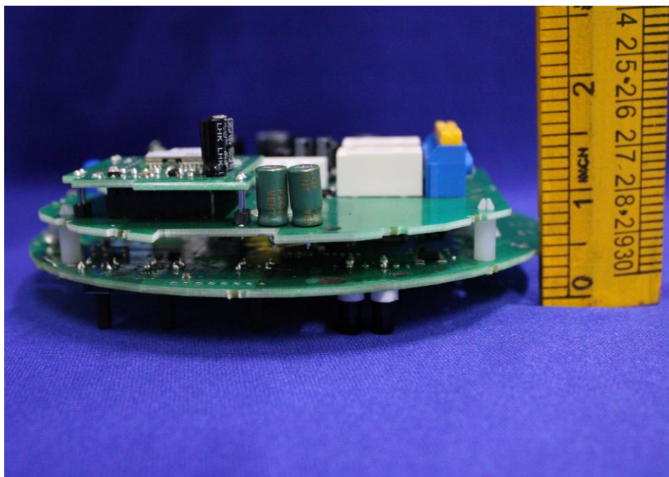
Photo 4: ANSI EM CPU with LORA MOD KYZ CARD Dimension View
