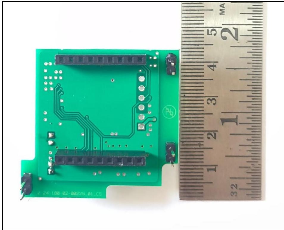
Photo 7: Module With Dimensions
