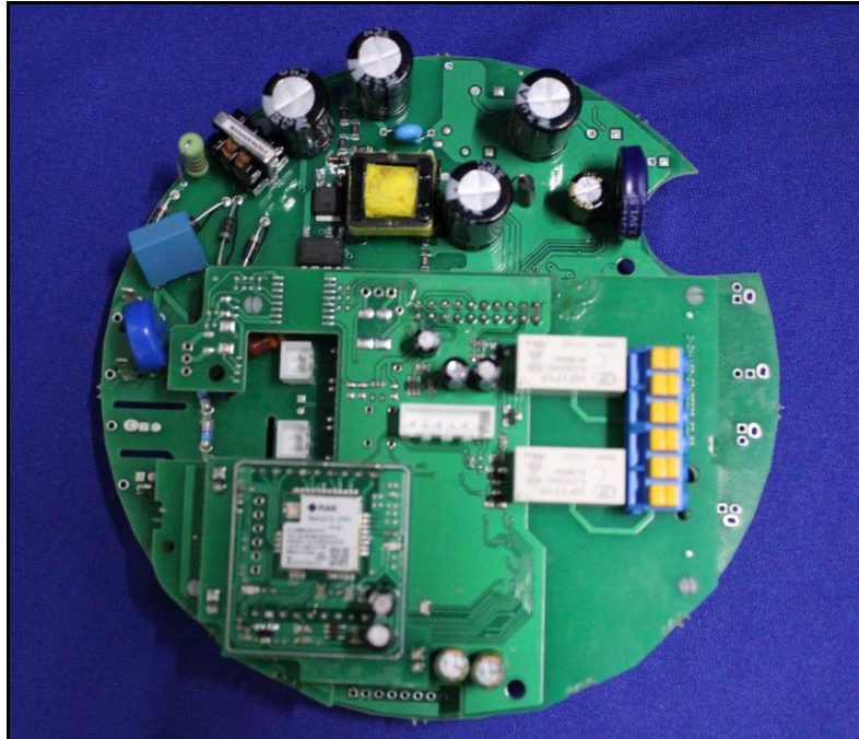
Photo 1: ANSI EM CPU with LORA MOD KYZ CARD Top View
