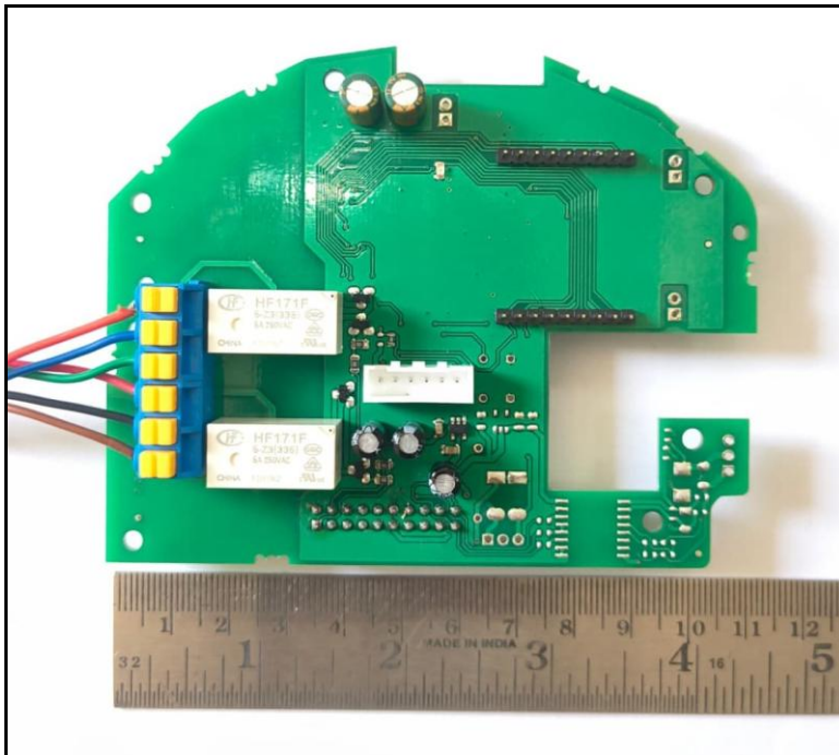
Photo 14: ANSI EM Addon LoRa Mod KYZ card front view
