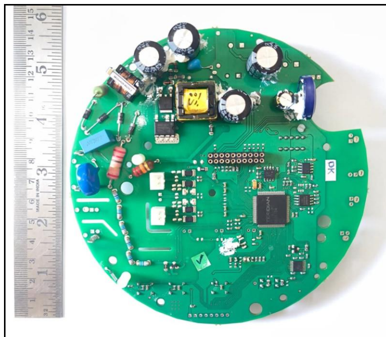
Photo 12: ANSI EM CPU Card Front view
