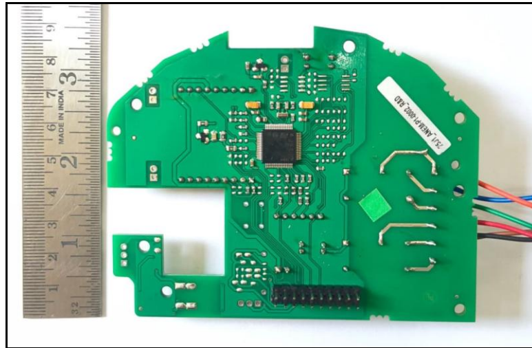
Photo 15: ANSI EM Addon LoRa Mod KYZ card rare view
