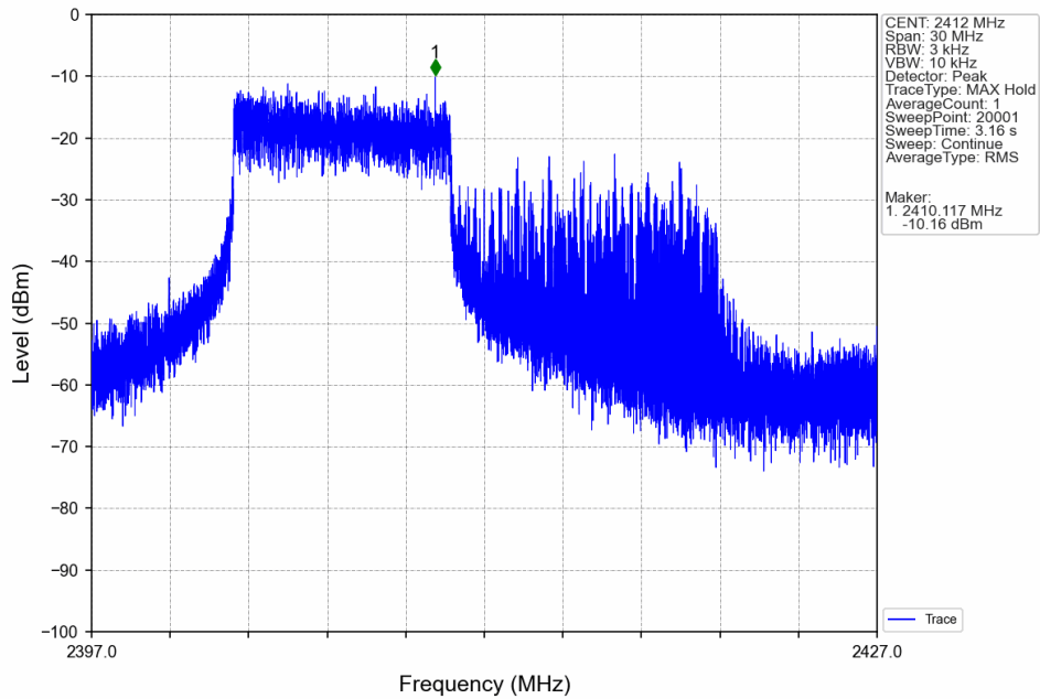
802.11ax(HEW20) LCH 2412MHz RU106 Left Ant7 (MIMO) NTN
