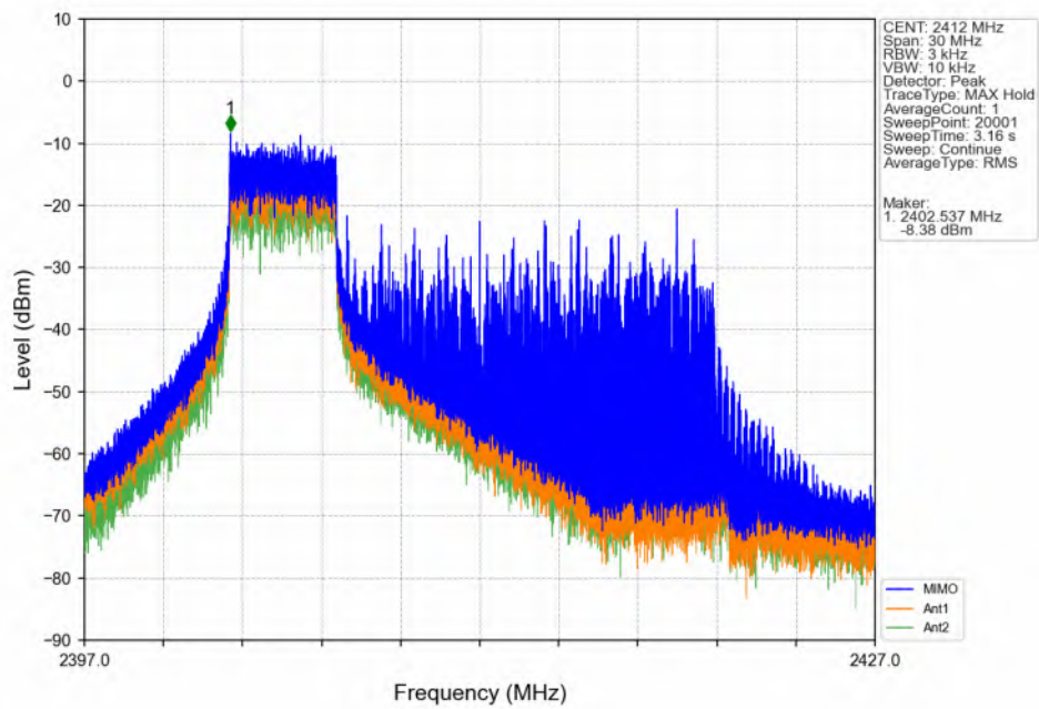
802.11ax(HEW20)_LCH_2412MHz_RU52_Left MIMO_NTNV
