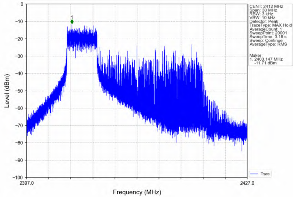
802.11ax(HEW20)_LCH_2412MHz_RU52_Left MIMO_NTNV
