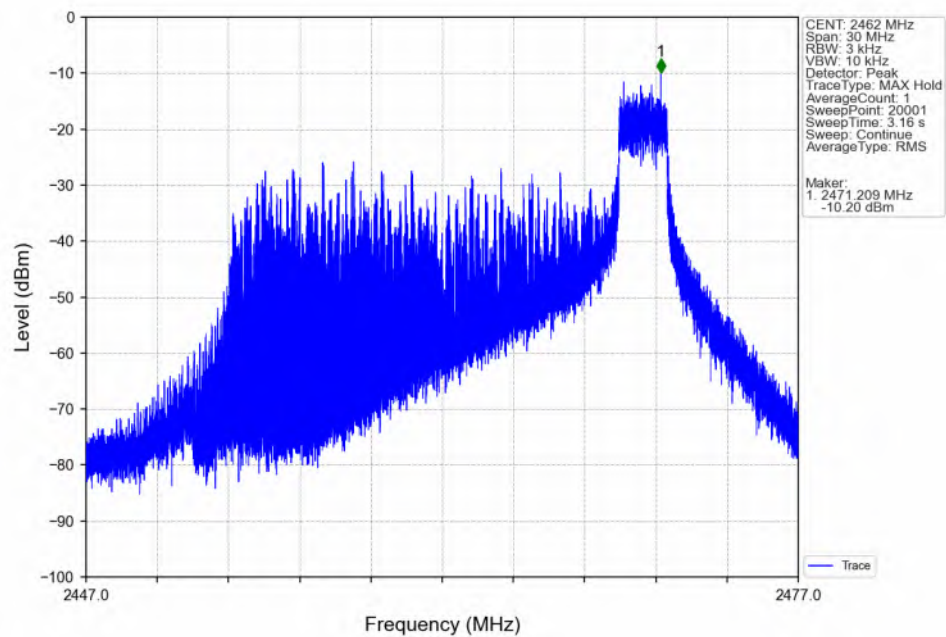
802.11ax(HEW20) HCH 2462MHz RU26 Right Ant7 (MIMO) NTN
