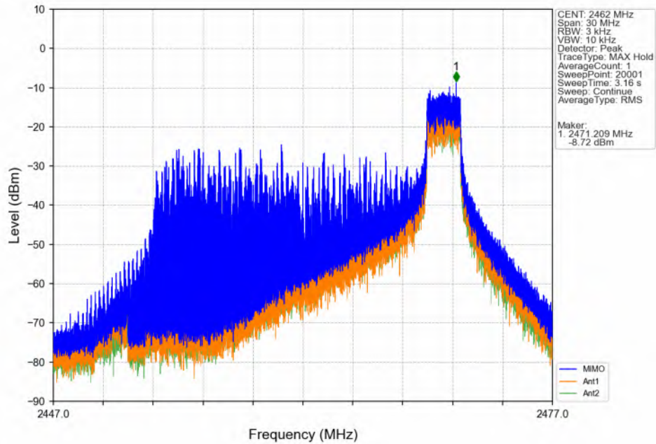
802.11ax(HEW20) HCH 2462MHz RU52 Right Ant6 (MIMO) NTN
