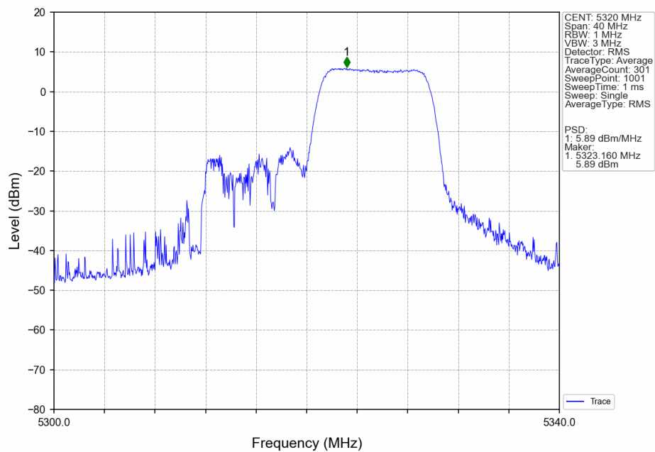
802.11ax(HEW20) HCH 5320MHz RU106 Right Ant6 NTN
