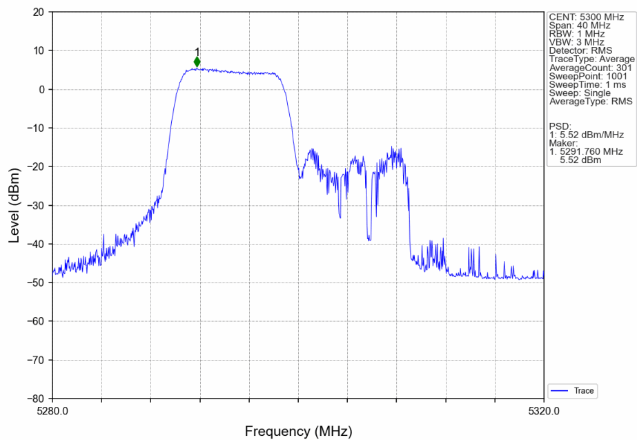
802.11ax(HEW20)_MCH_5300MHz_RU106_Left_Ant6_NTNV
