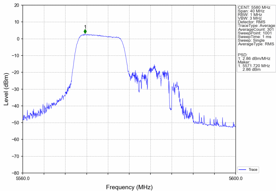
802.11ax(HEW20)_MCH_5580MHz_RU106_Left_Ant6_NTNV
