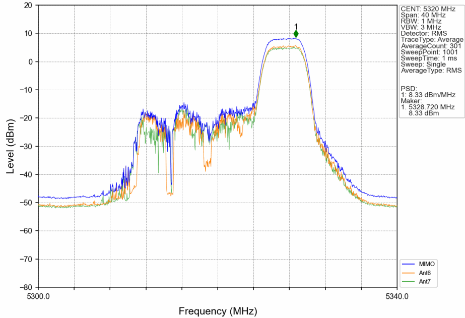
802.11ax(HEW20) HCH 5320MHz RU106 Right Ant6 NTN
