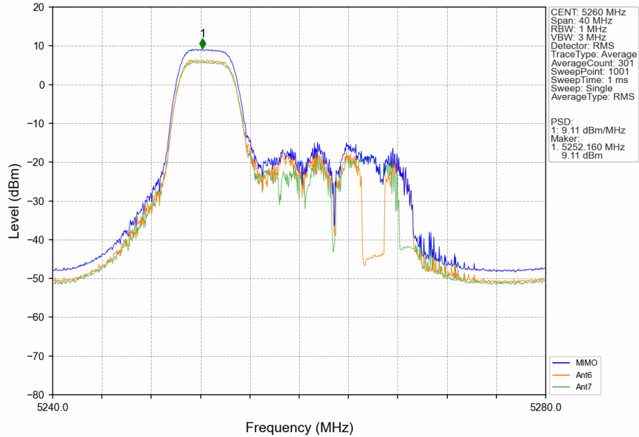
802.11ax(HEW20) LCH_5260MHz RU106 Left Ant6 NTN
