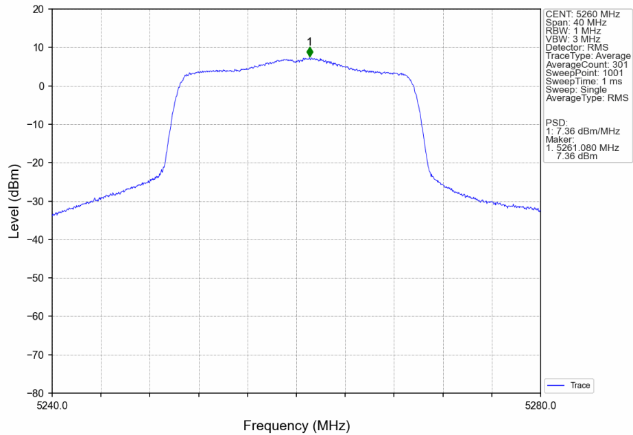
802.11ax(HEW20) LCH_5260MHz_SU / Ant7_NTNV
