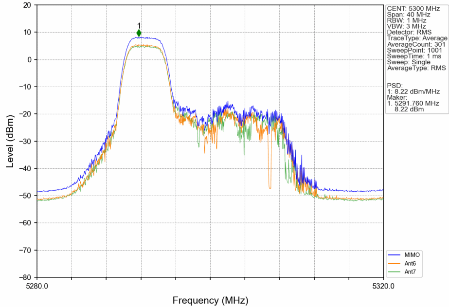
802.11ax(HEW20)_MCH_5300MHz_RU106_Left_Ant6_NTNV
