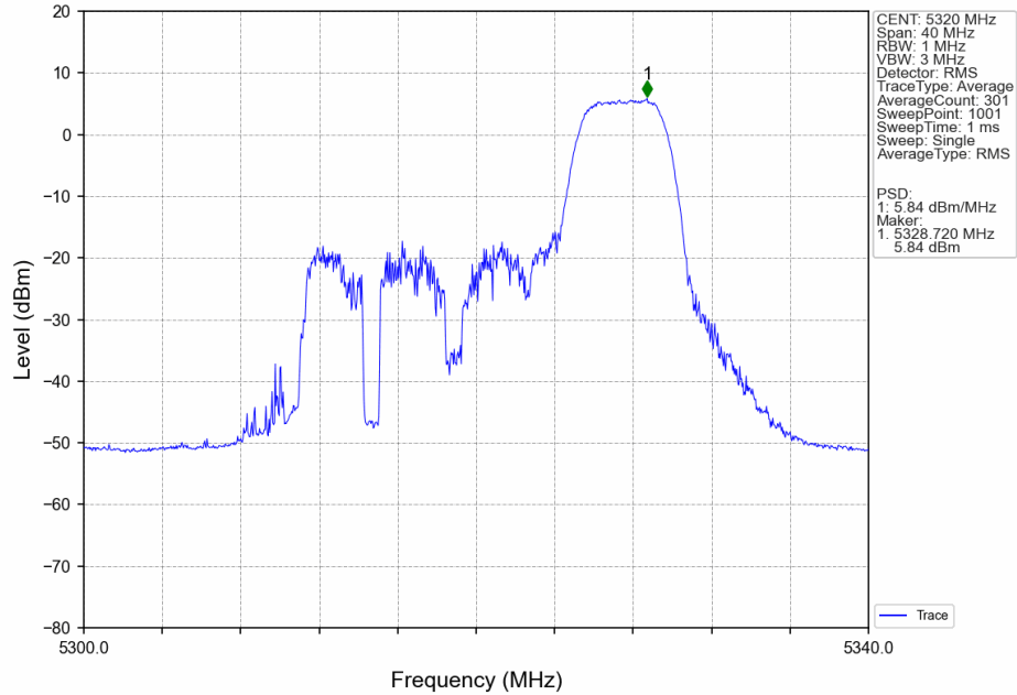
802.11ax(HEW20) HCH_5320MHz RU52 Right_Ant7 NTN
