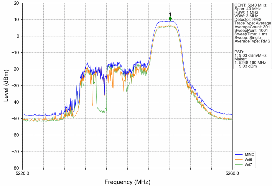
802.11ax(HEW20) HCH 5240MHz RU106 Right Ant6 NTN
