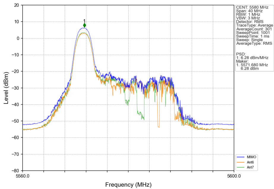
802.11ax(HEW20)_MCH_5580MHz_RU26_Left_MIMO_NTNV
