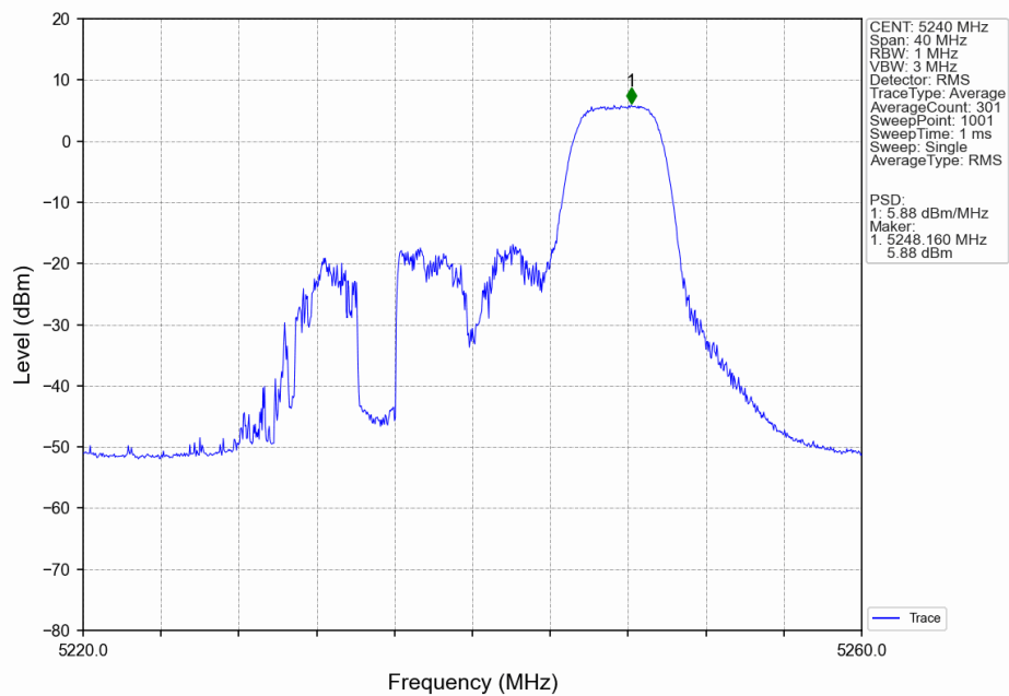
802.11ax(HEW20) HCH_5240MHz RU52_Right_Ant7_NTNV
