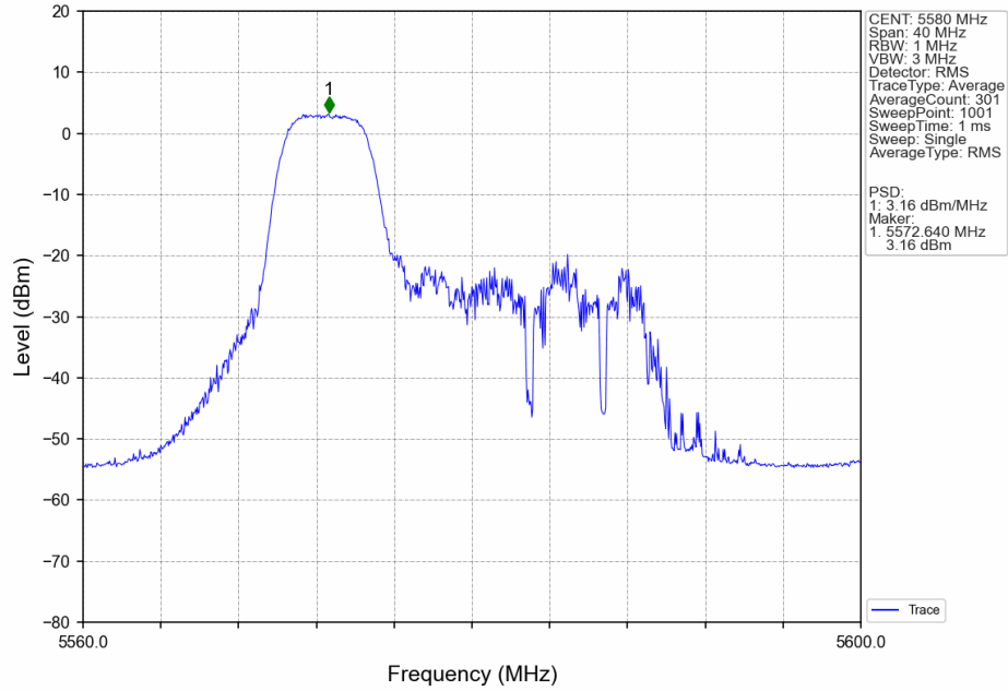
802.11ax(HEW20) MCH 5580MHz RU52 Left Ant7_NTNV
