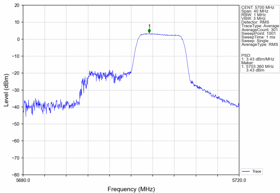
802.11ax(HEW20) HCH 5700MHz RU106 Right Ant6 NTN
