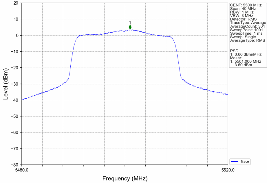
802.11ax(HEW20)_LCH_5500MHz_SU_ / Ant7_NTNV
