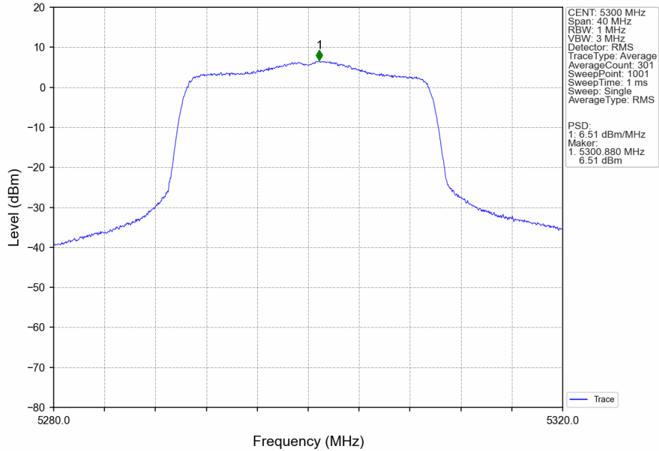
802.11ax(HEW20)_MCH_5300MHz_SU / Ant7 NTN
