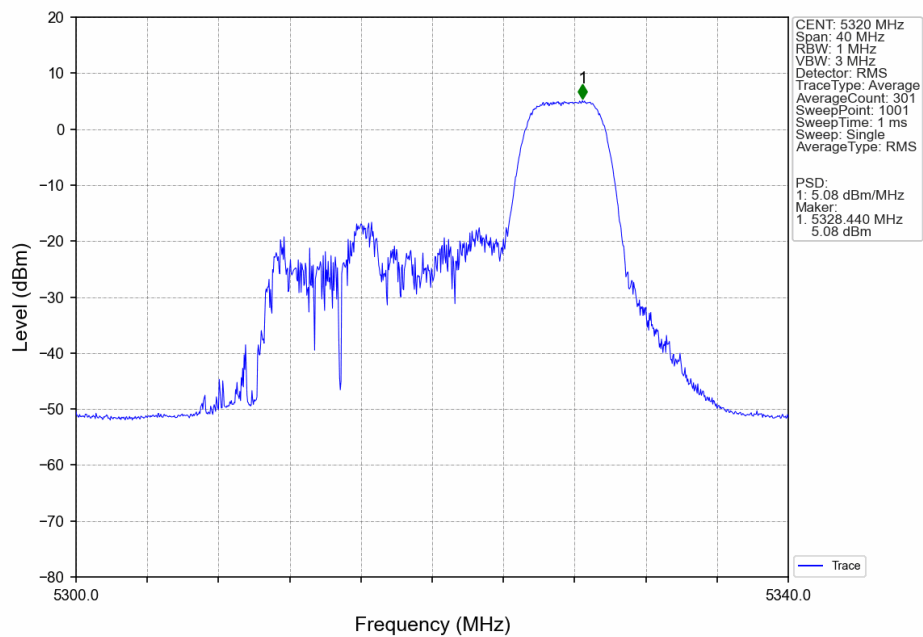
802.11ax(HEW20) HCH_5320MHz RU52 Right_Ant7 NTN
