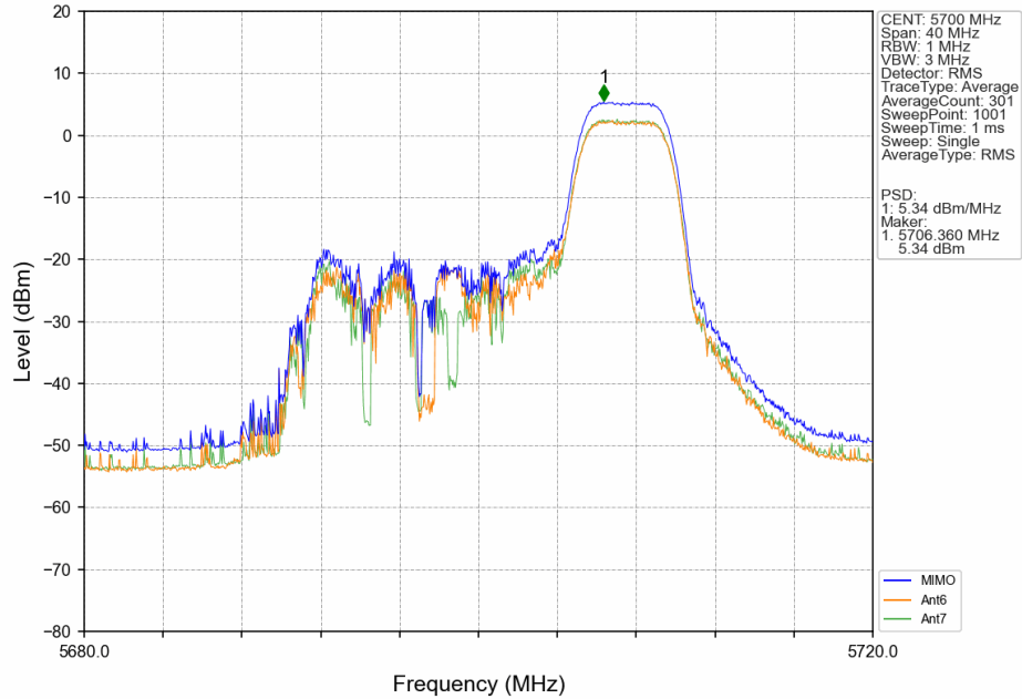
802.11ax(HEW20) HCH 5700MHz RU106 Right Ant6 NTN
