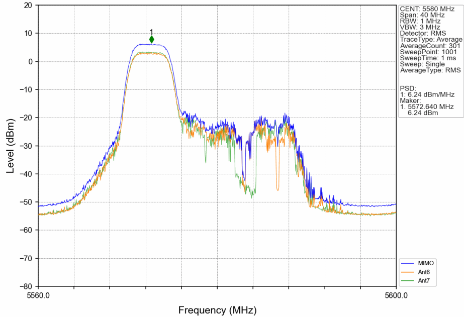
802.11ax(HEW20)_MCH_5580MHz_RU106_Left_Ant6_NTNV
