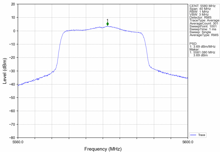
802.11ax(HEW20)_MCH_5580MHz_SU / Ant7 NTN
