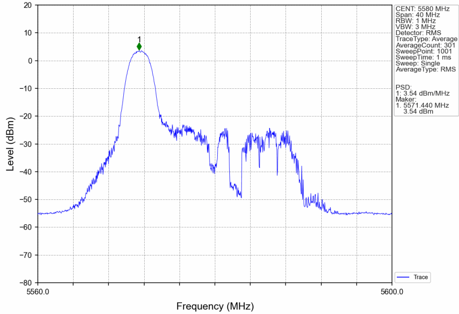
802.11ax(HEW20)_MCH_5580MHz_RU26_Left_MIMO_NTNV
