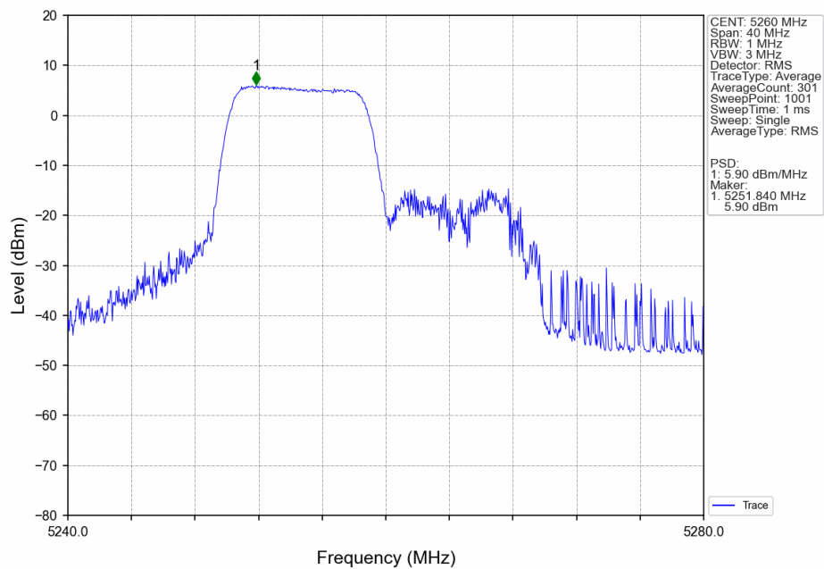
802.11ax(HEW20) LCH_5260MHz RU106 Left Ant6 NTN
