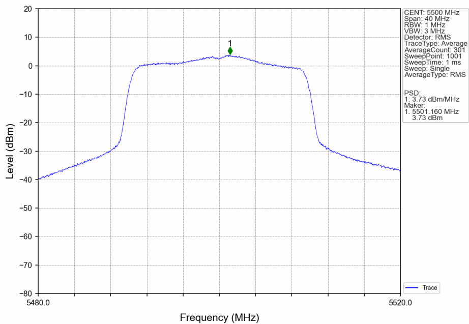
802.11ax(HEW20)_LCH_5500MHz_SU_ / Ant7_NTNV
