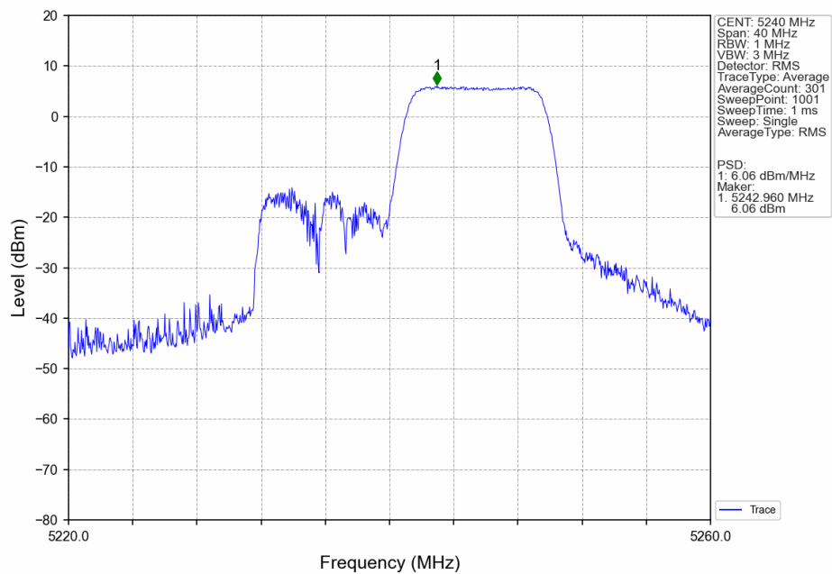
802.11ax(HEW20) HCH 5240MHz RU106 Right Ant6 NTN
