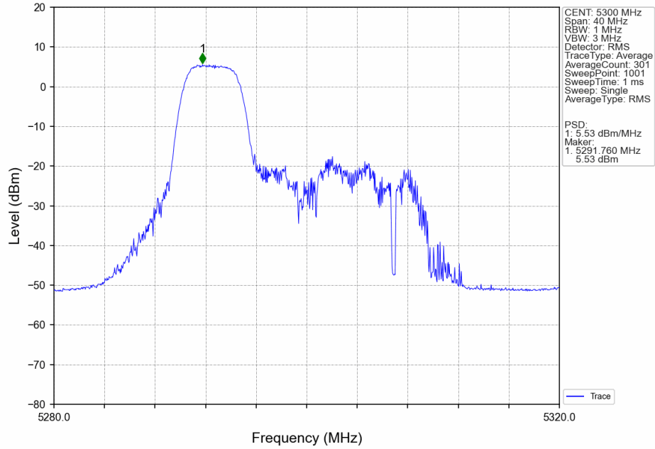
802.11ax(HEW20) MCH 5300MHz RU52 Left Ant7_NTNV
