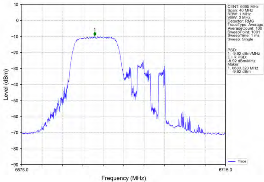
802.11ax(HEW20)_MCH_6695MHz_RU106_Left_MIMO_NTNV
