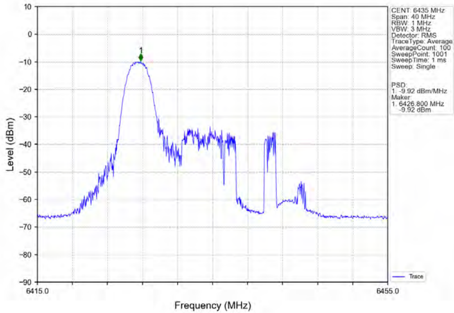
802.11ax(HEW20) LCH_6435MHz_RU26_Left_MIMO_NTNV
