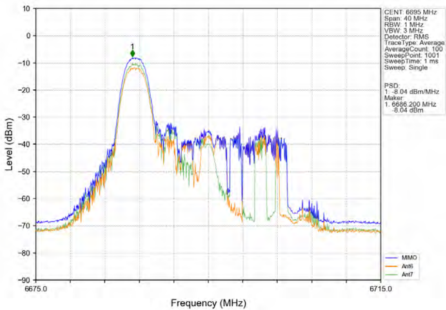
802.11ax(HEW20)_MCH_6695MHz_RU26_Left_MIMO_NTNV
