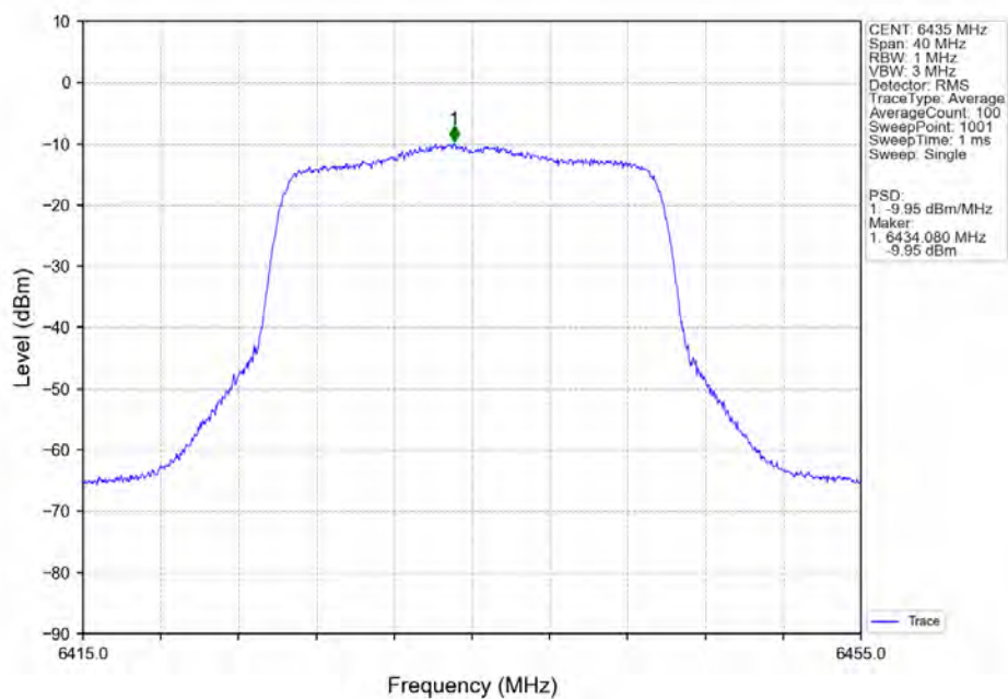
802.11ax(HEW20)_LCH_6435MHz_SU_ / Ant7_NTNV
