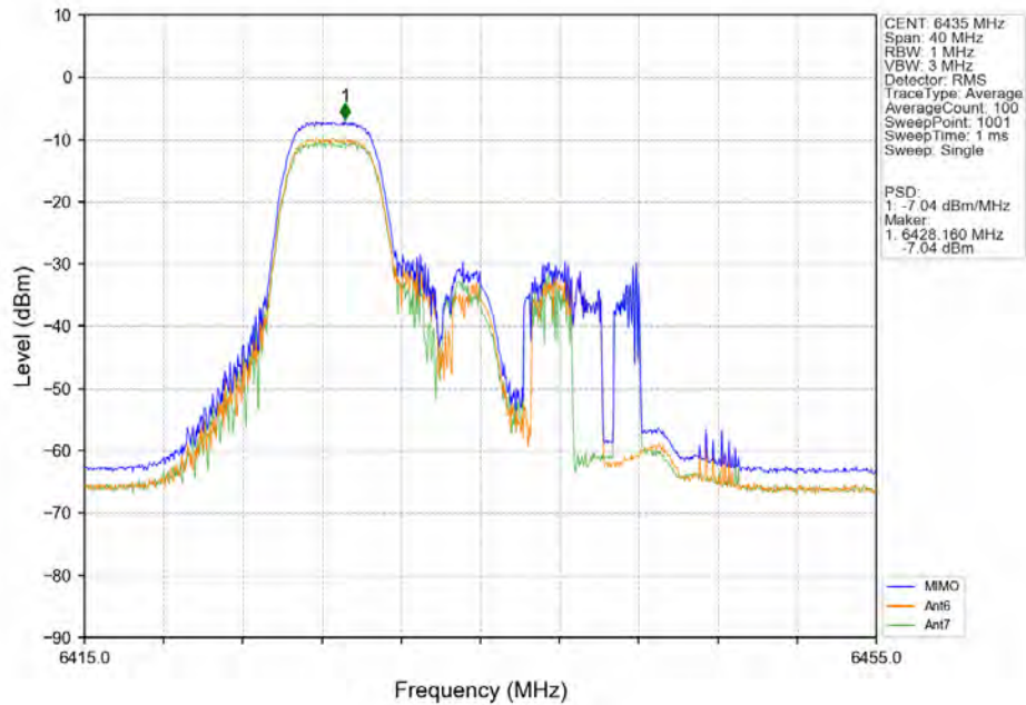
802.11ax(HEW20)_LCH_6435MHz_RU106_Left_Ant6_NTNV
