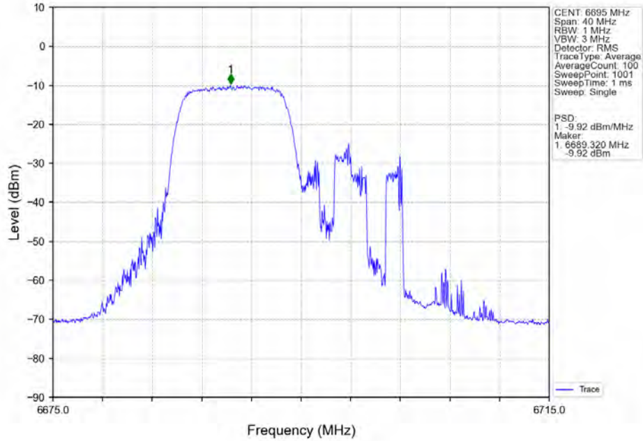
802.11ax(HEW20)_MCH_6695MHz_RU106_Left_MIMO_NTNV
