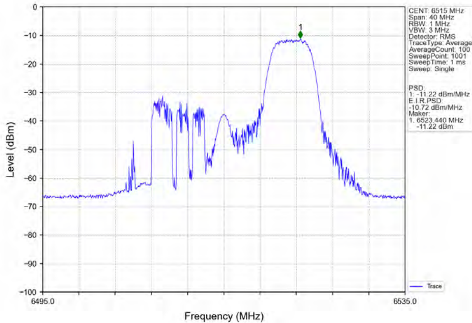
802.11ax(HEW20)_HCH_6515MHz_RU52_Right_Ant7_NTNV
