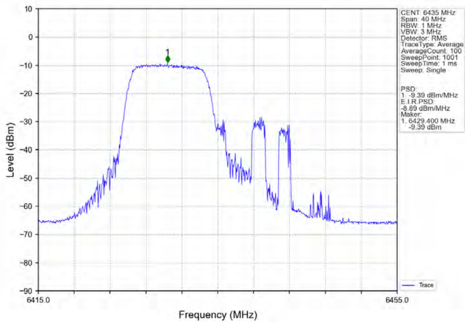
802.11ax(HEW20)_LCH_6435MHz_RU106_Left_Ant6_NTNV
