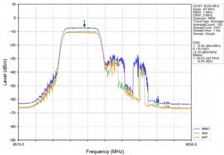
802.11ax(HEW20) LCH_6535MHz_RU106_Left_MIMO_NTNV
