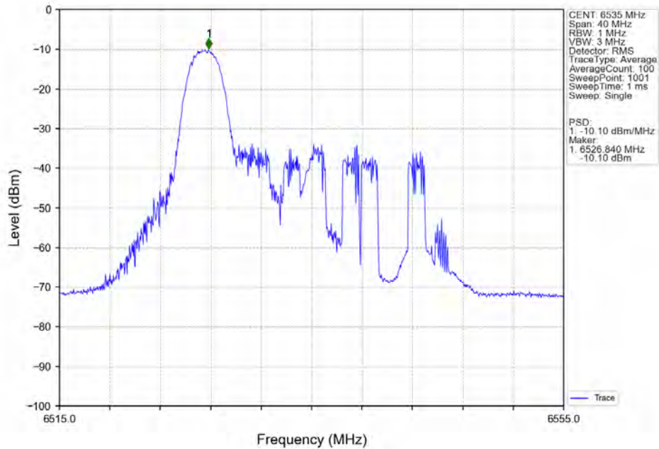
802.11ax(HEW20) LCH_6535MHz_RU26_Left_MIMO_NTNV
