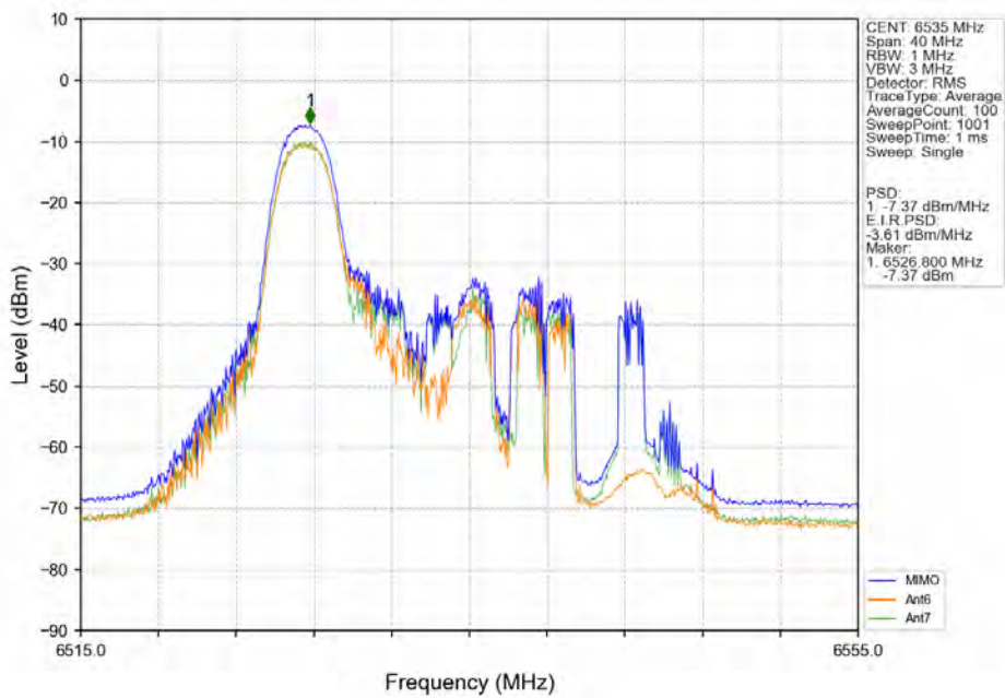
802.11ax(HEW20) LCH_6535MHz_RU26_Left_MIMO_NTNV
