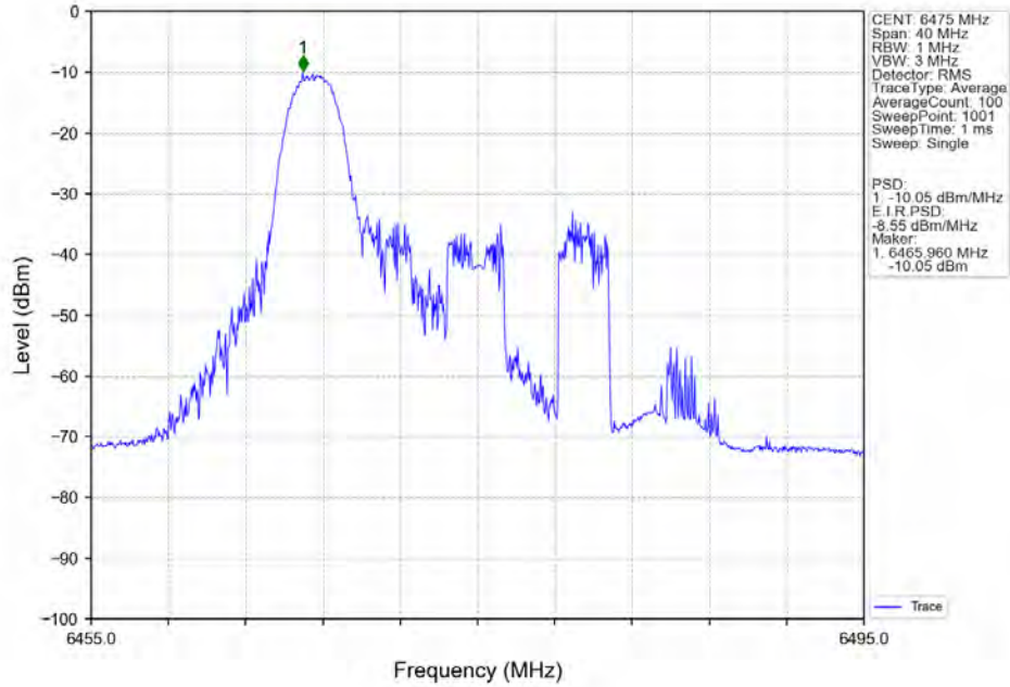
802.11ax(HEW20)_MCH_6475MHz_RU26_Left_MIMO_NTNV
