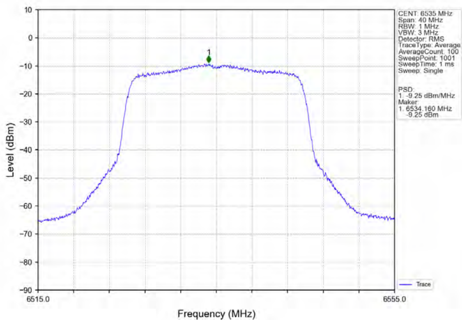
802.11ax(HEW20)_LCH_6535MHz_SU_ / Ant7_NTNV
