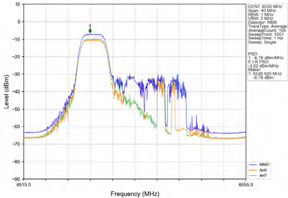
802.11ax(HEW20)_LCH_6535MHz_RU106_Left_Ant6_NTNV
