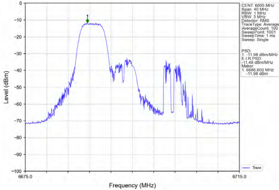
802.11ax(HEW20) MCH 6695MHz RU52 Left_Ant7_NTNV
