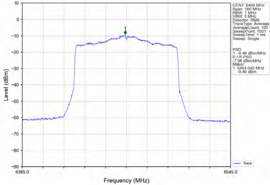
802.11ax(HEW80)_LCH_6465MHz_SU / MIMO_NTNV
