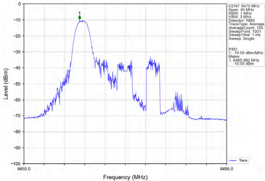
802.11ax(HEW20)_MCH_6475MHz_RU26_Left_MIMO_NTNV
