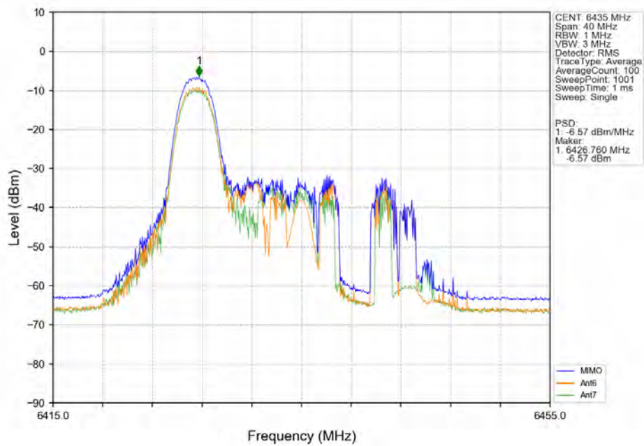
802.11ax(HEW20) LCH_6435MHz_RU26_Left_MIMO_NTNV
