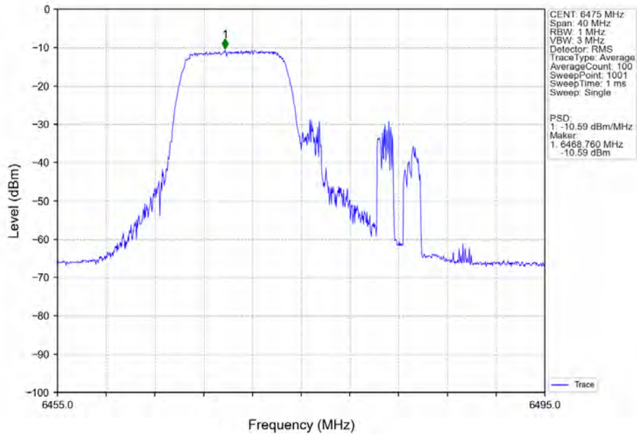
802.11ax(HEW20)_MCH_6475MHz_RU106_Left_MIMO_NTNV
