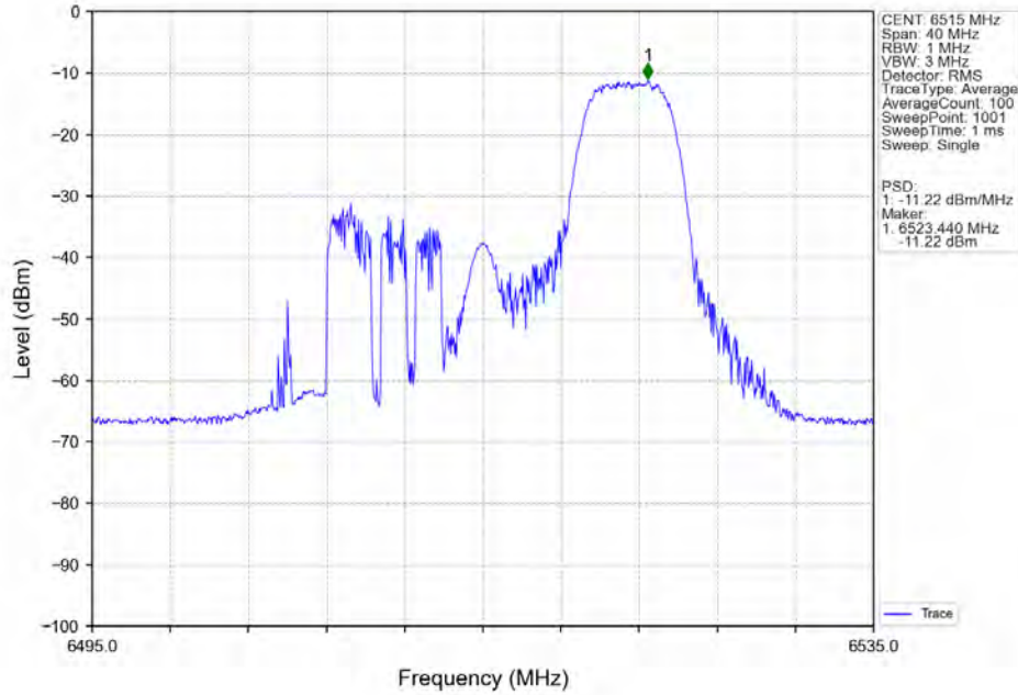
802.11ax(HEW20) HCH_6515MHz RU52_Right_Ant7_NTNV
