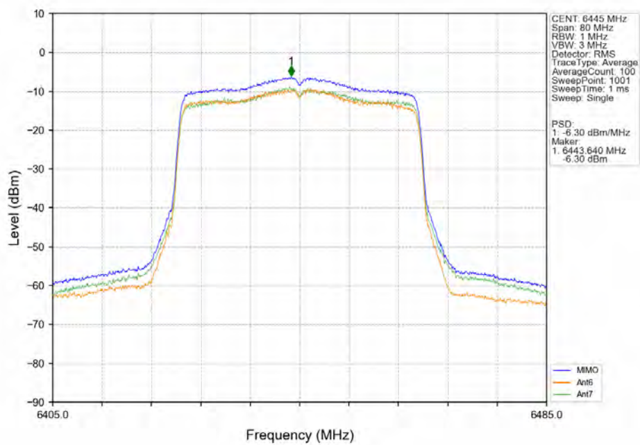
802.11ax(HEW40)_LCH_6445MHz_SU / MIMO_NTNV
