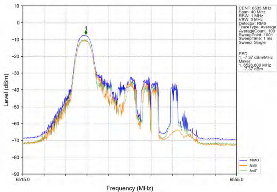
802.11ax(HEW20) LCH_6535MHz_RU26_Left_MIMO_NTNV
