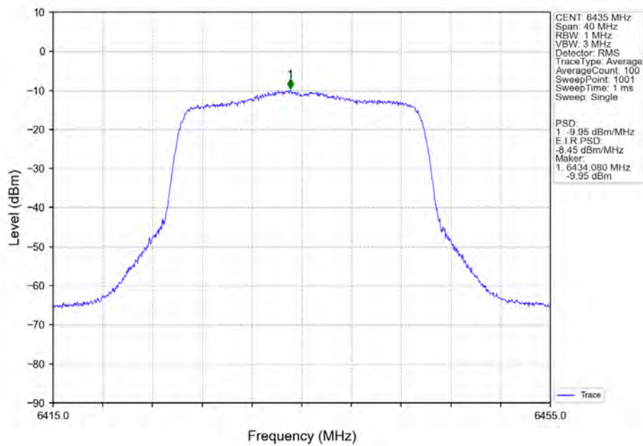
802.11ax(HEW20)_LCH_6435MHz_SU_ / Ant7_NTNV
