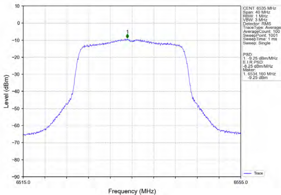
802.11ax(HEW20)_LCH_6535MHz_SU_ / Ant7_NTNV
