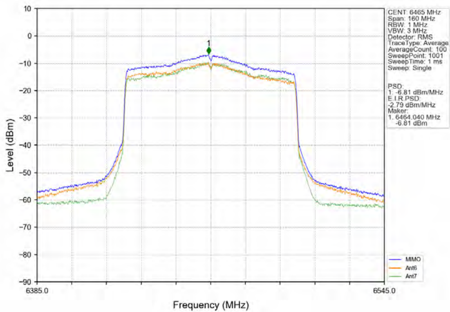
802.11ax(HEW80)_LCH_6465MHz_SU / MIMO_NTNV
