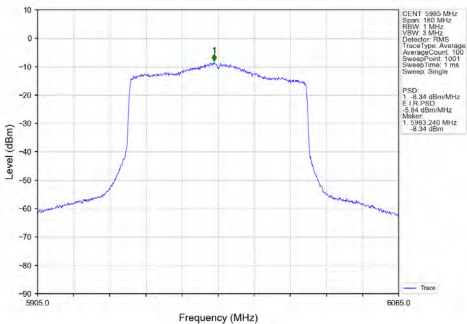
802.11ax(HEW80)_LCH_5985MHz_SU_ / Ant7_NTNV
