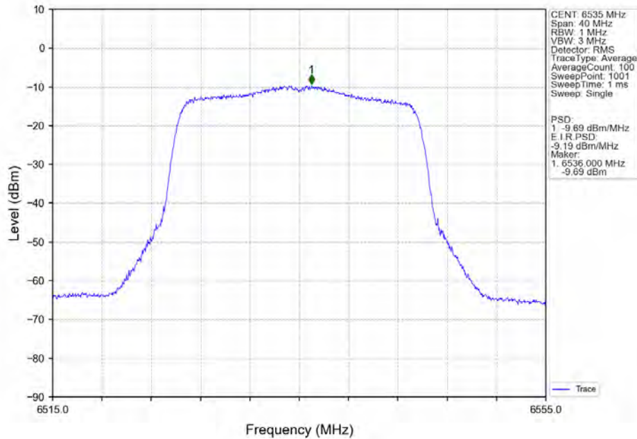
802.11ax(HEW20)_LCH_6535MHz_SU_ / Ant7_NTNV
