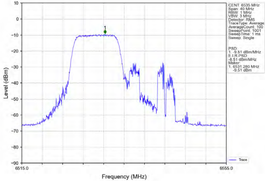
802.11ax(HEW20) LCH_6535MHz_RU106_Left_MIMO_NTNV
