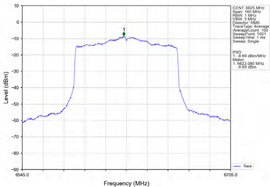
802.11ax(HEW80)_LCH_6625MHz_SU_ / Ant7_NTNV
