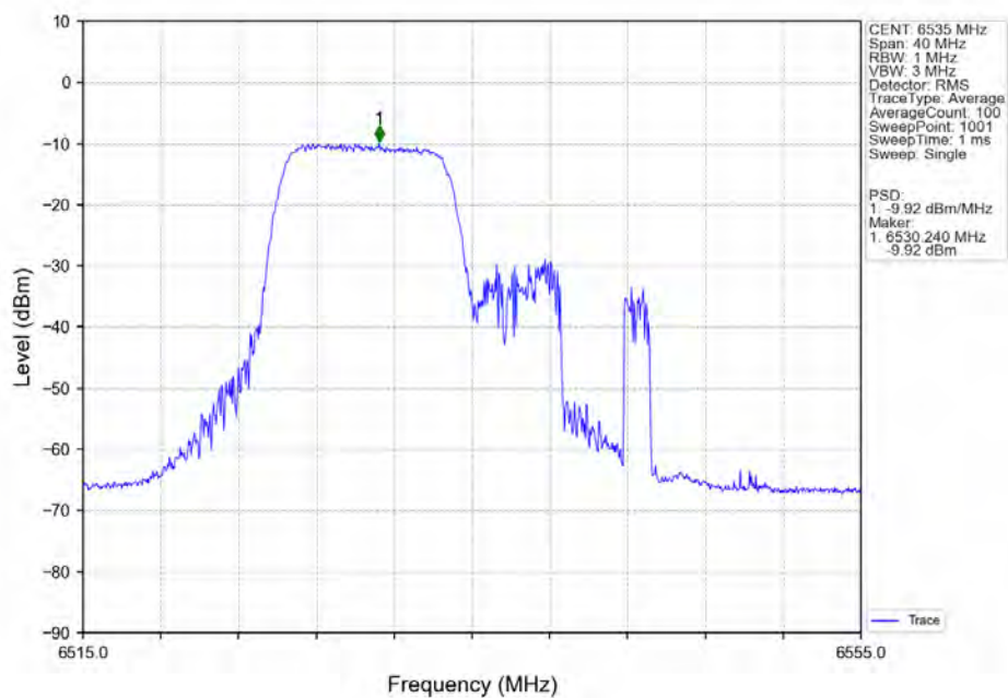
802.11ax(HEW20)_LCH_6535MHz_RU106_Left_Ant6_NTNV
