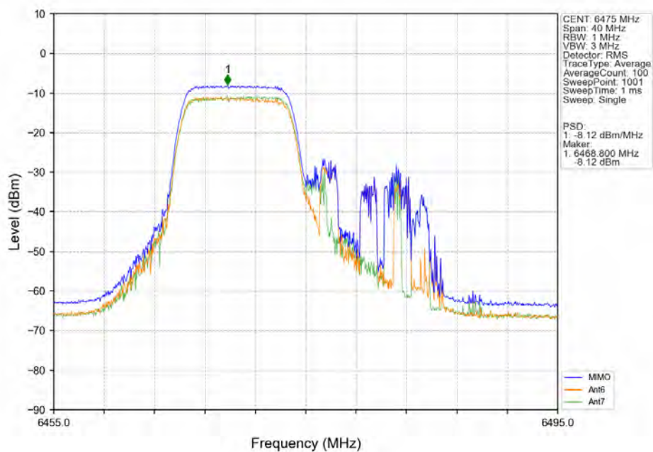
802.11ax(HEW20)_MCH_6475MHz_RU106_Left_MIMO_NTNV
