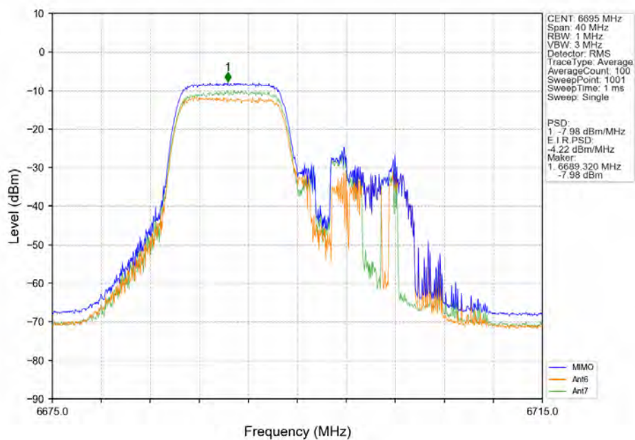
802.11ax(HEW20)_MCH_6695MHz_RU106_Left_MIMO_NTNV
