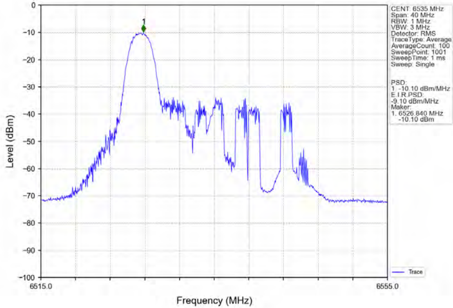
802.11ax(HEW20) LCH_6535MHz_RU26_Left_MIMO_NTNV
