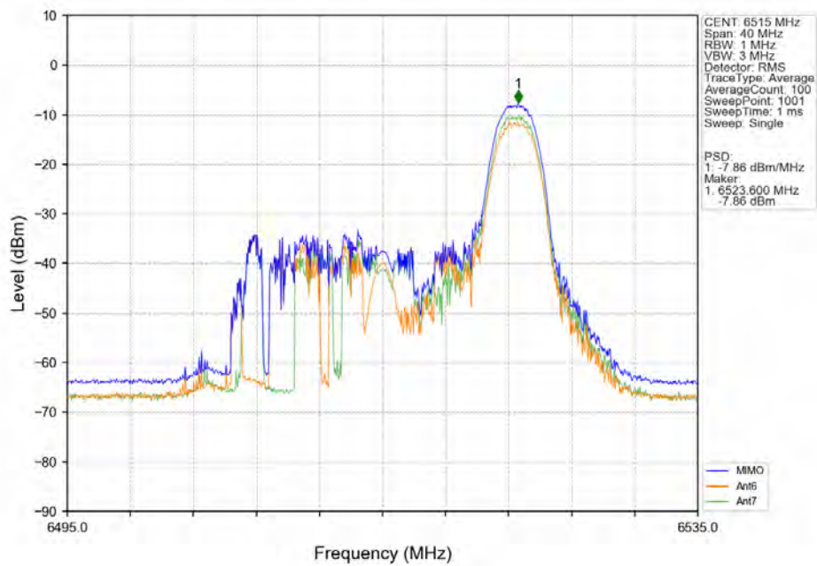
802.11ax(HEW20) HCH 6515MHz RU26 Right MIMO NTN
