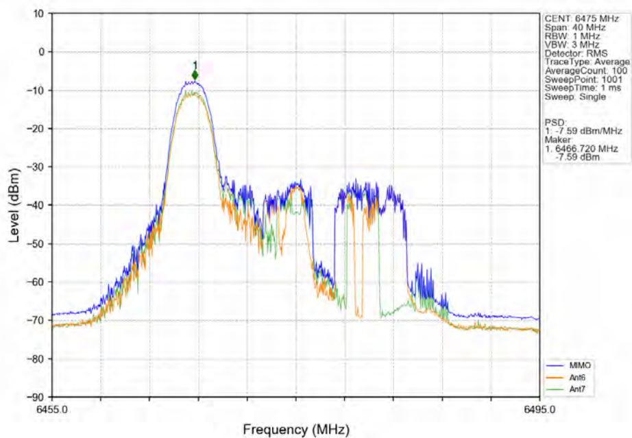
802.11ax(HEW20)_MCH_6475MHz_RU26_Left_MIMO_NTNV
