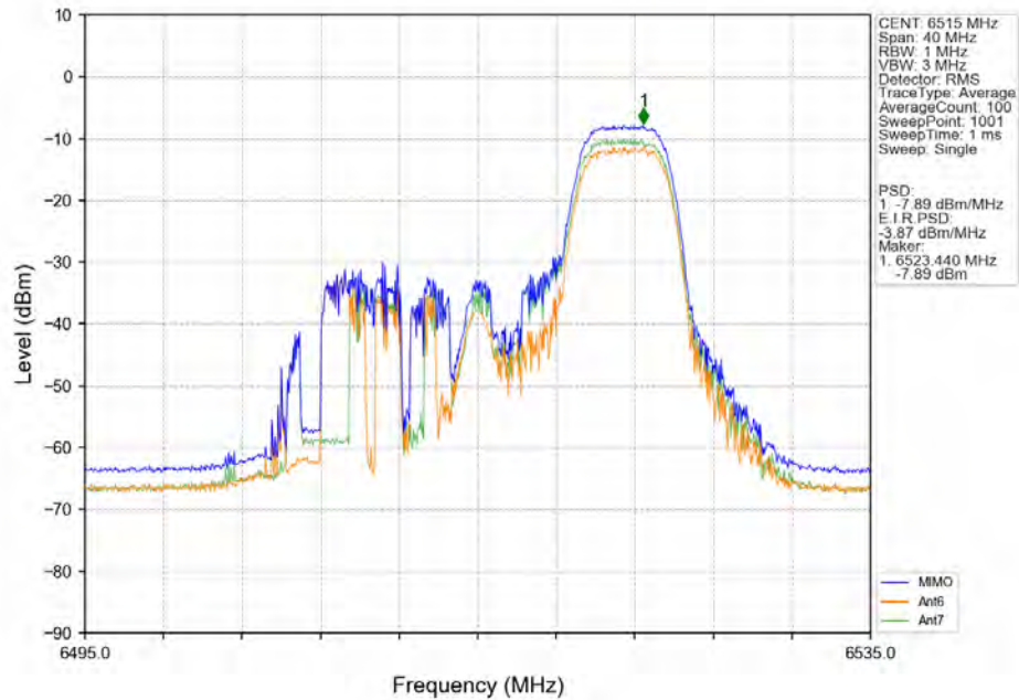
802.11ax(HEW20) HCH 6515MHz RU106 Right Ant6 NTN
