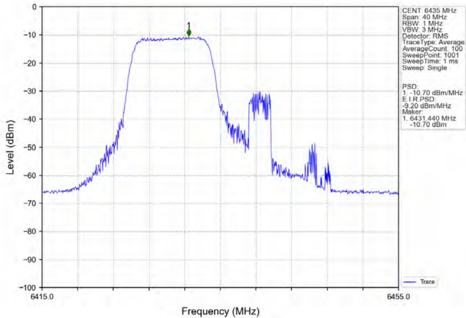
802.11ax(HEW20) LCH_6435MHz_RU106_Left_MIMO_NTNV
