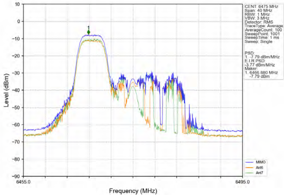
802.11ax(HEW20)_MCH_6475MHz_RU106_Left_Ant6_NTNV
