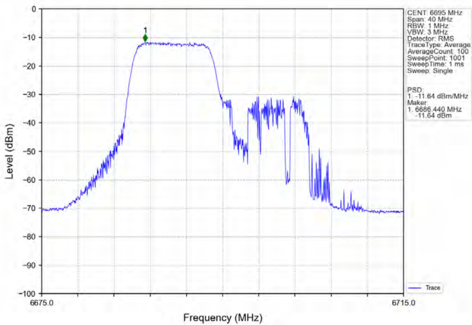
802.11ax(HEW20)_MCH_6695MHz_RU106_Left_Ant6_NTNV
