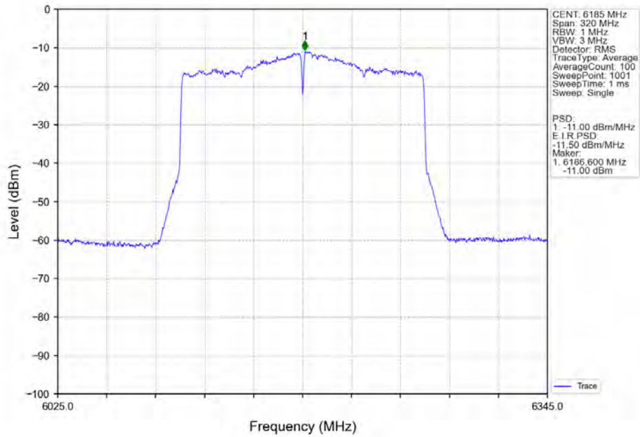
802.11ax(HEW160)_MCH_6185MHz_SU_/_Ant7_NTNV
