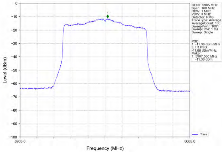
802.11ax(HEW80)_LCH_5985MHz_SU_ / Ant7_NTNV
