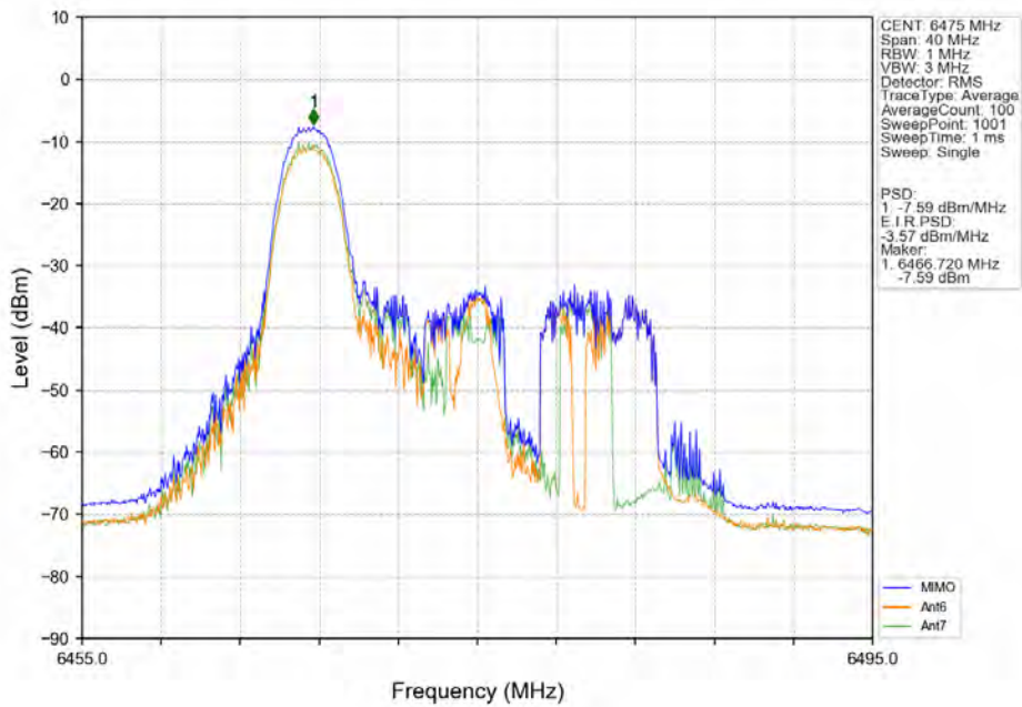
802.11ax(HEW20)_MCH_6475MHz_RU26_Left_MIMO_NTNV
