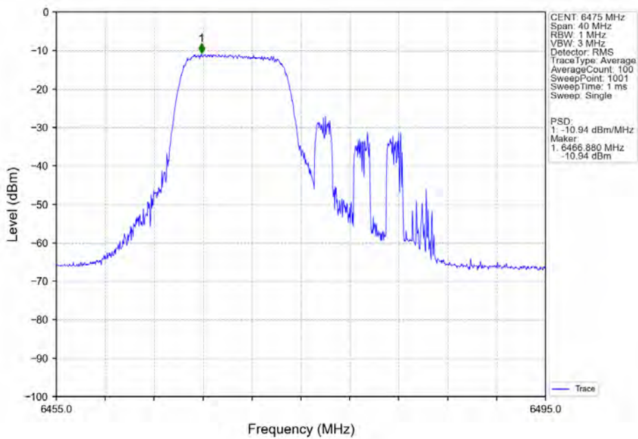
802.11ax(HEW20)_MCH_6475MHz_RU106_Left_Ant6_NTNV
