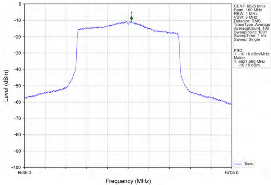
802.11ax(HEW80)_LCH_6625MHz_SU_ / Ant7_NTNV
