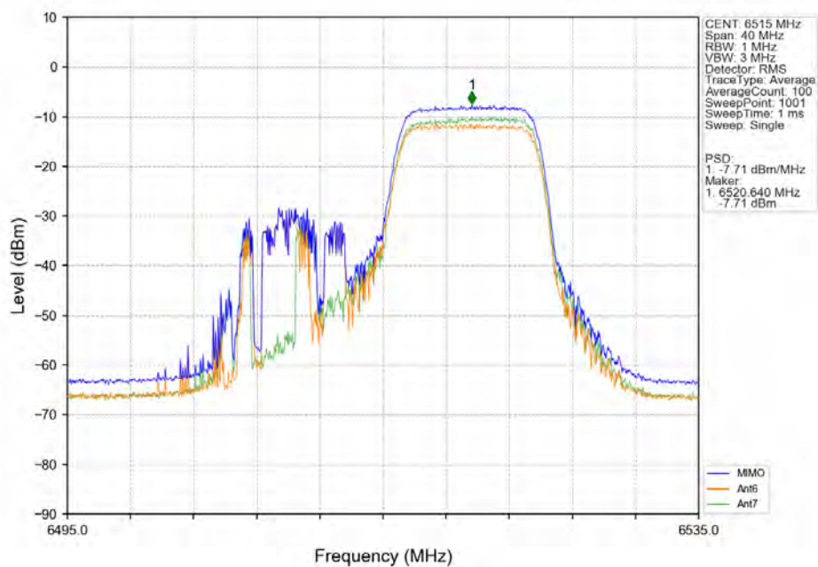
802.11ax(HEW20) HCH 6515MHz RU106 Right MIMO NTN
