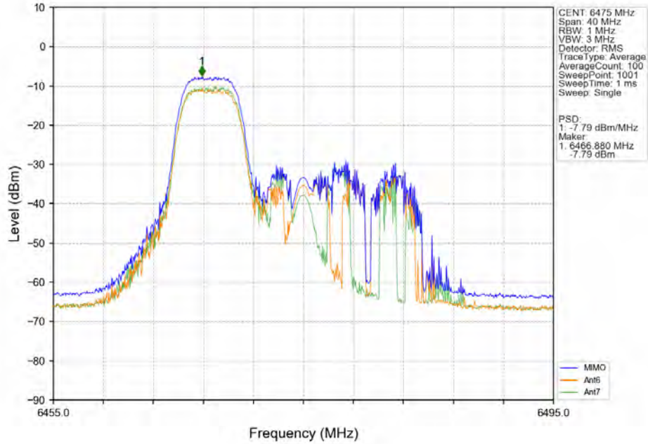
802.11ax(HEW20)_MCH_6475MHz_RU106_Left_Ant6_NTNV
