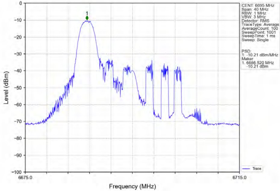
802.11ax(HEW20)_MCH_6695MHz_RU26_Left_MIMO_NTNV
