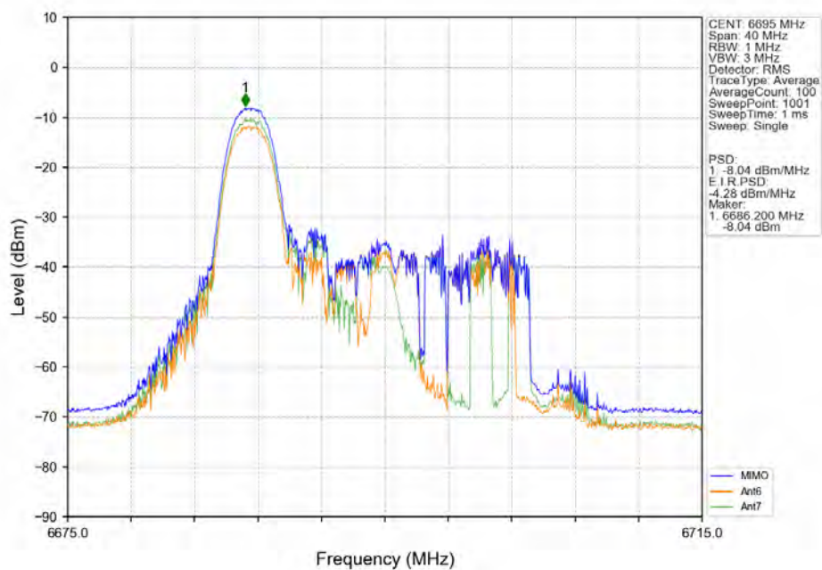
802.11ax(HEW20)_MCH_6695MHz_RU26_Left_MIMO_NTNV
