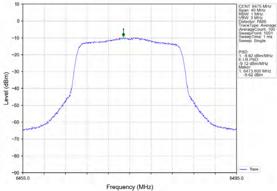
802.11ax(HEW20)_MCH_6475MHz_SU / Ant7 NTN
