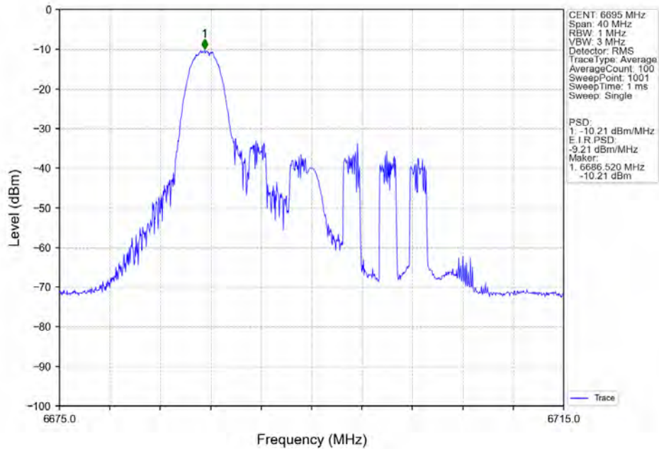
802.11ax(HEW20)_MCH_6695MHz_RU26_Left_MIMO_NTNV
