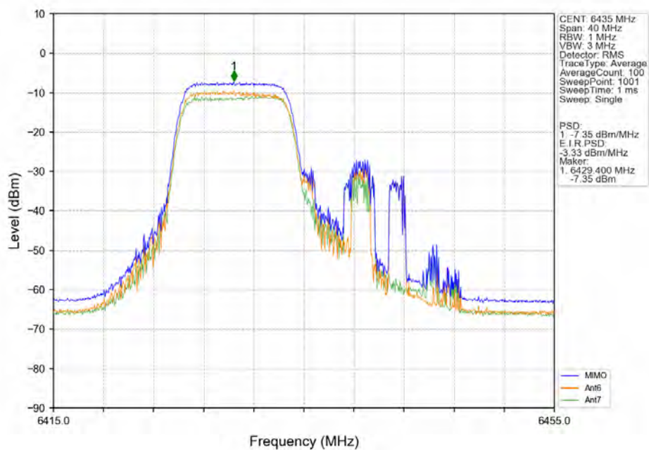
802.11ax(HEW20) LCH_6435MHz_RU106_Left_MIMO_NTNV
