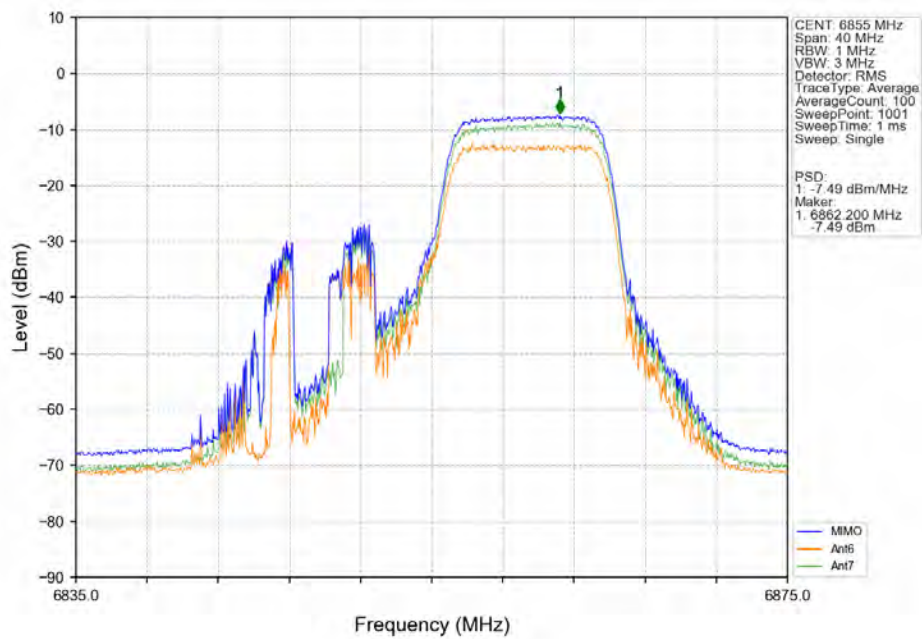
802.11ax(HEW20) HCH 6855MHz RU106 Right MIMO NTN
