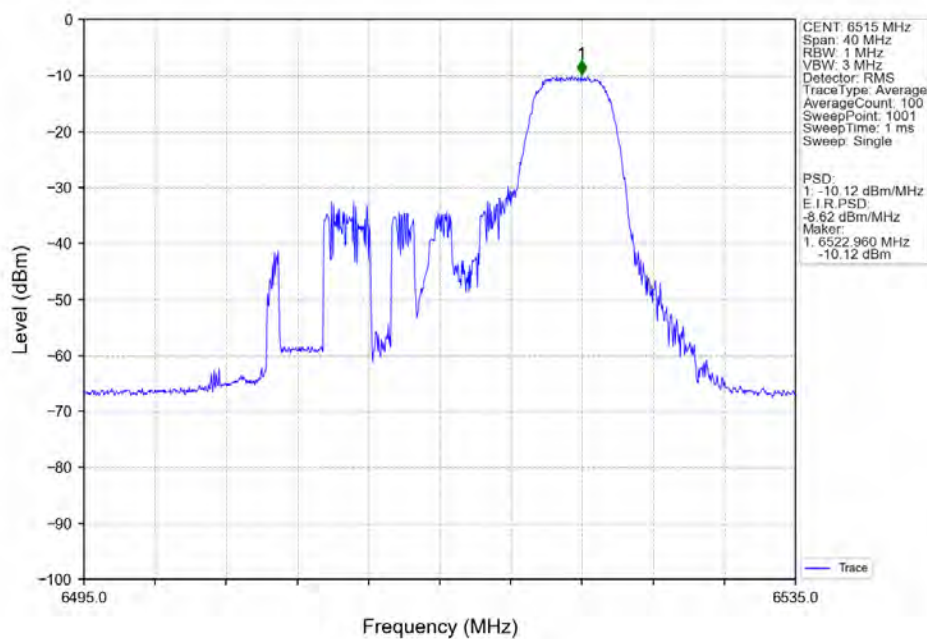
802.11ax(HEW20)_HCH_6515MHz_RU52_Right_Ant7_NTNV
