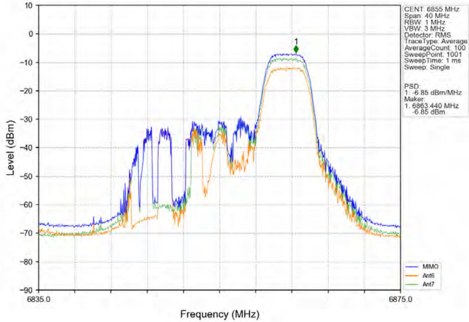
802.11ax(HEW20) HCH 6855MHz RU106 Right Ant6 NTN
