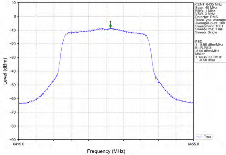
802.11ax(HEW20)_LCH_6435MHz_SU_ / Ant7_NTNV
