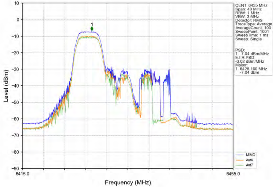
802.11ax(HEW20)_LCH_6435MHz_RU106_Left_Ant6_NTNV
