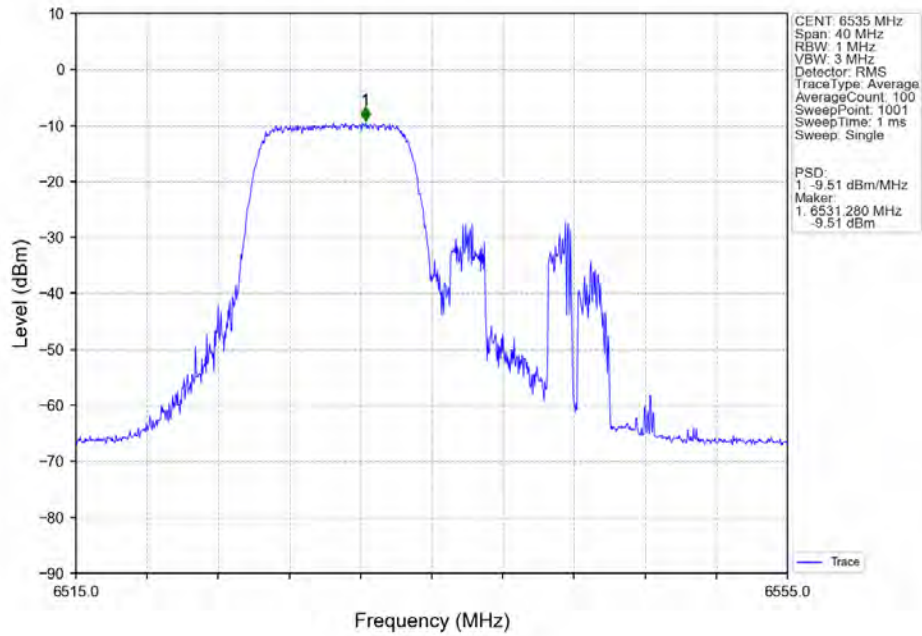
802.11ax(HEW20) LCH_6535MHz_RU106_Left_MIMO_NTNV
