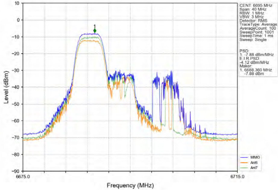
802.11ax(HEW20)_MCH_6695MHz_RU106_Left_Ant6_NTNV
