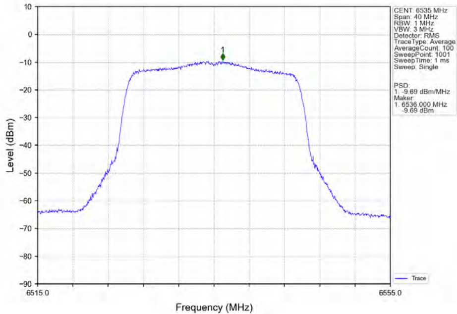
802.11ax(HEW20)_LCH_6535MHz_SU_ / Ant7_NTNV
