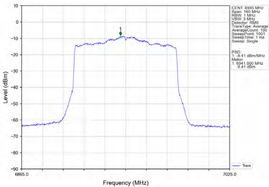
802.11ax(HEW80)_LCH_6945MHz_SU_ / Ant7_NTNV
