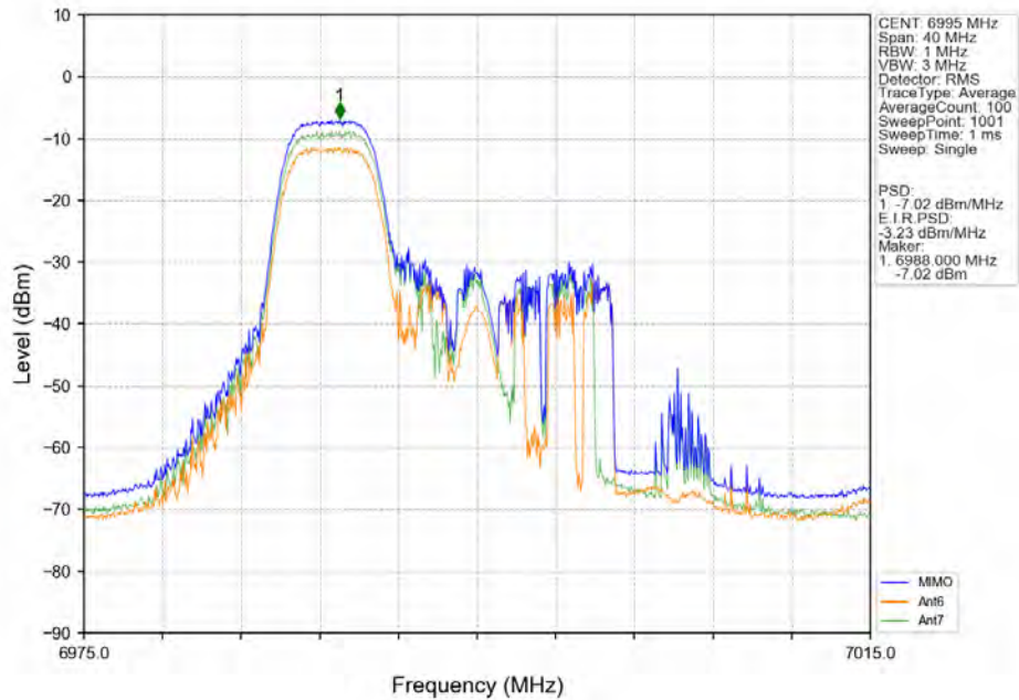
802.11ax(HEW20)_MCH_6995MHz_RU106_Left_Ant6_NTNV
