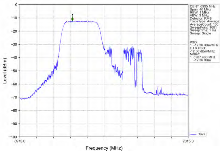
802.11ax(HEW20)_MCH_6995MHz_RU106_Left_Ant6_NTNV
