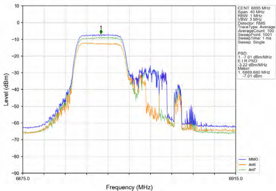
802.11ax(HEW20) LCH_6895MHz_RU106_Left_MIMO_NTNV
