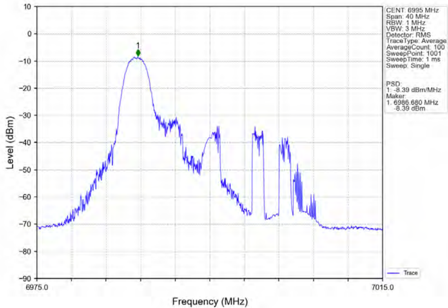
802.11ax(HEW20)_MCH_6995MHz_RU26_Left_MIMO_NTNV
