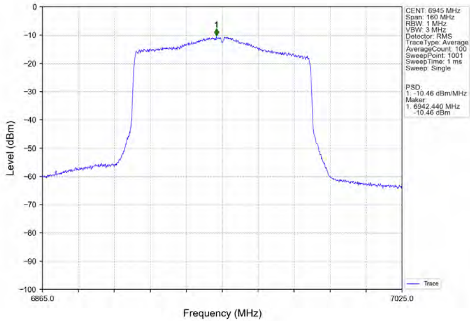
802.11ax(HEW80)_LCH_6945MHz_SU_ / Ant7_NTNV
