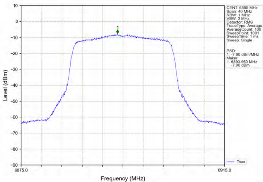
802.11ax(HEW20)_LCH_6895MHz_SU_ / Ant7_NTNV
