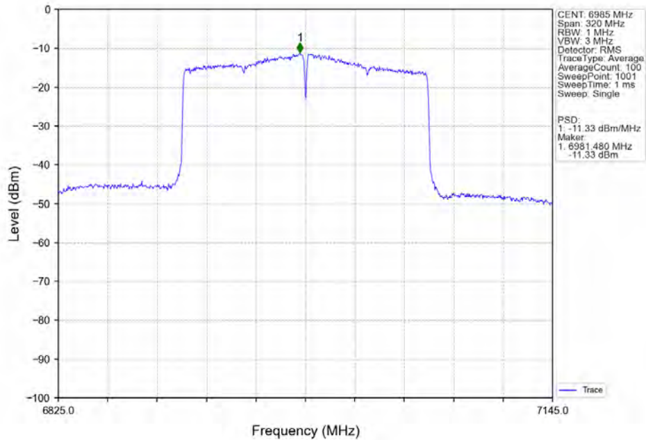
802.11ax(HEW160)_MCH_6985MHz_SU_/_Ant7_NTNV
