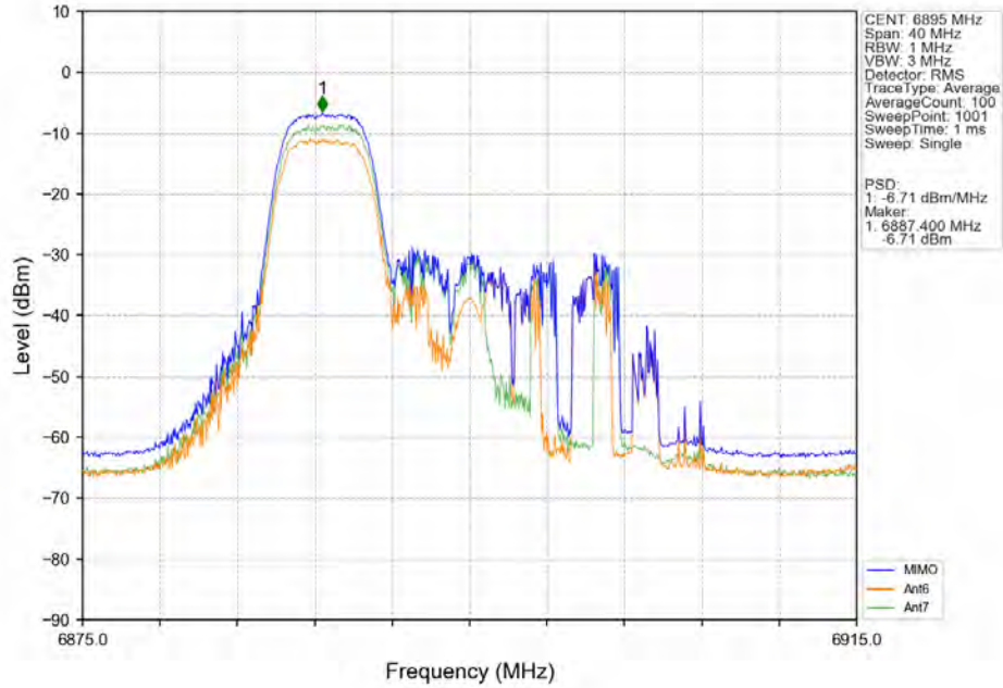
802.11ax(HEW20) LCH_6895MHz RU106 Left Ant6 NTN
