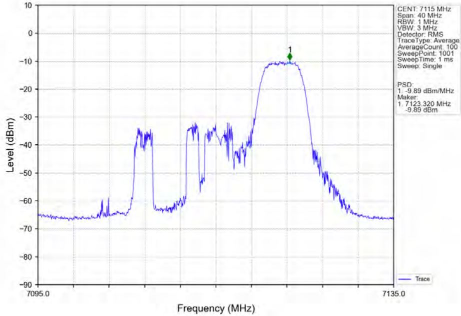
802.11ax(HEW20)_HCH_7115MHz_RU52_Right_Ant7_NTNV
