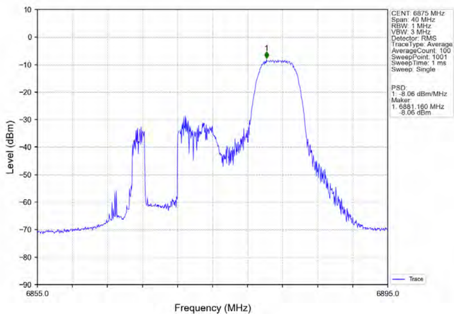
802.11ax(HEW20)_HCH_6875MHz_RU52_Right_Ant7_NTNV
