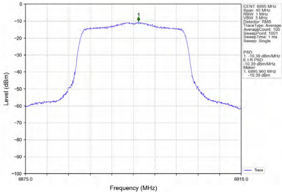
802.11ax(HEW20)_LCH_6895MHz_SU_ / Ant7_NTNV
