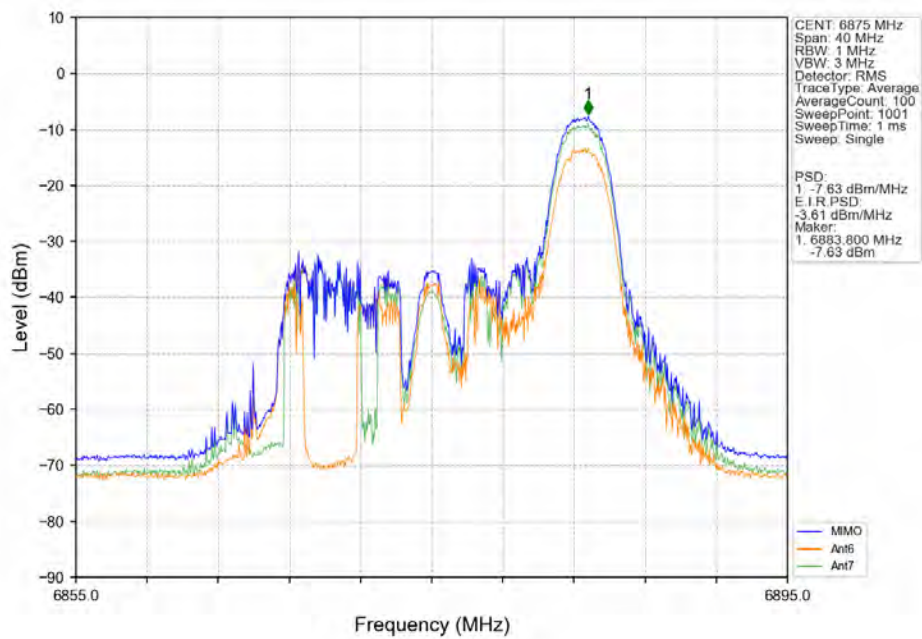
802.11ax(HEW20)_HCH_6875MHz_RU26_Right_MIMO_NTNV
