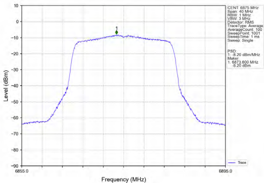
802.11ax(HEW20) HCH_6875MHz_SU / Ant7 NTN
