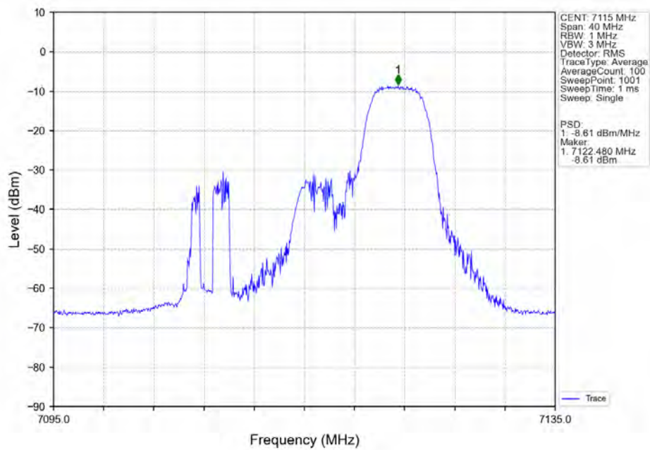
802.11ax(HEW20)_HCH_7115MHz_RU52_Right_Ant7_NTNV
