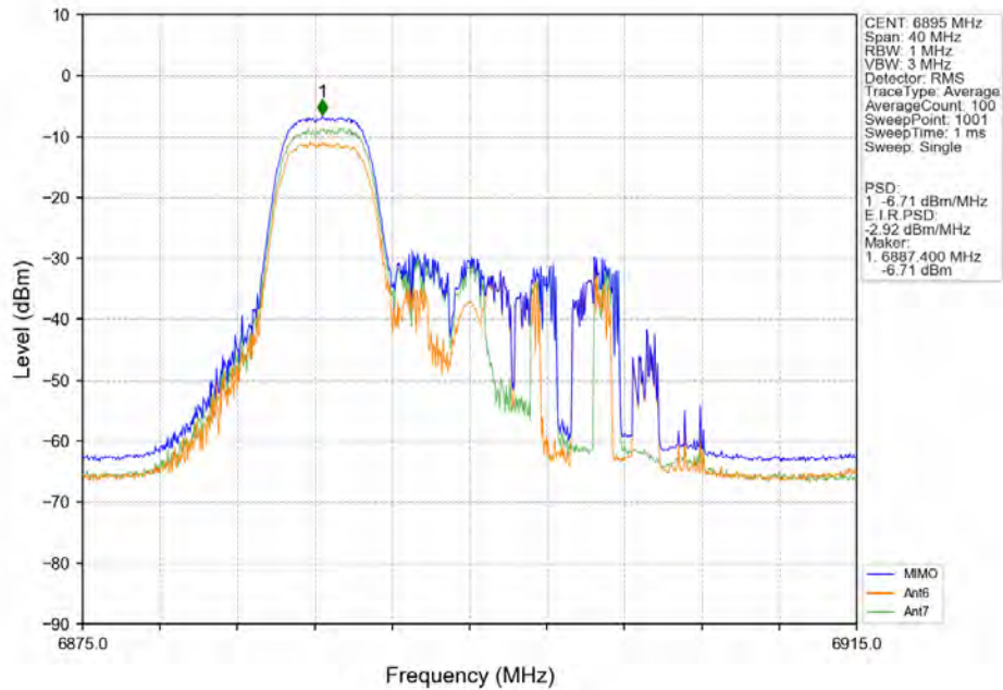
802.11ax(HEW20)_LCH_6895MHz_RU106_Left_Ant6_NTNV
