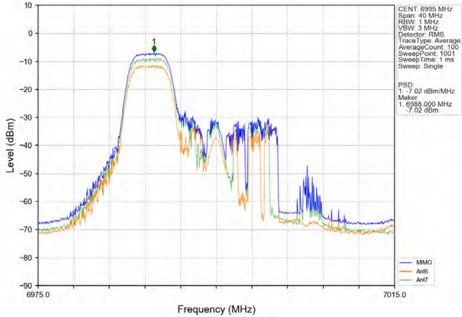
802.11ax(HEW20)_MCH_6995MHz_RU106_Left_Ant6_NTNV
