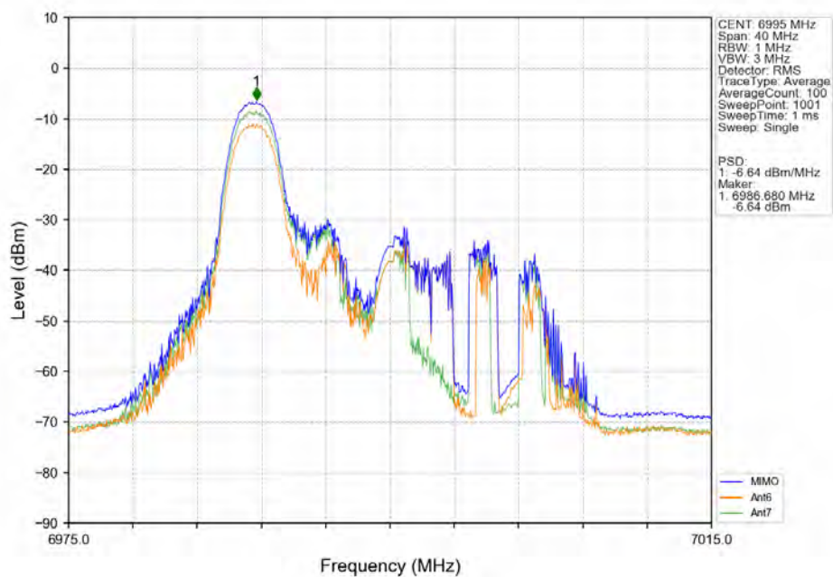
802.11ax(HEW20)_MCH_6995MHz_RU26_Left_MIMO_NTNV
