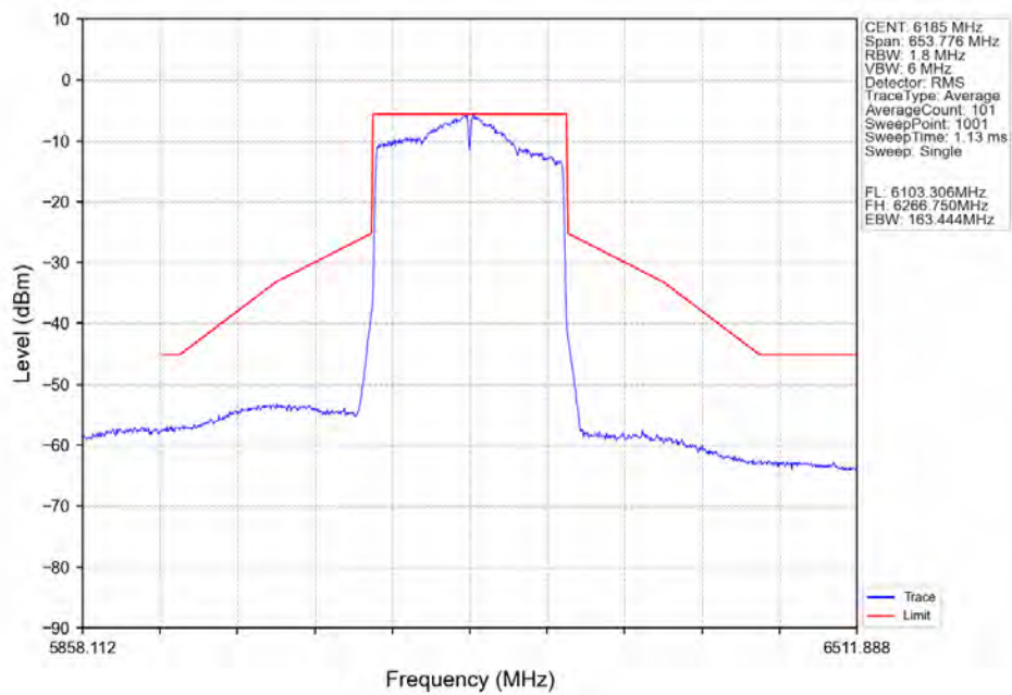
802.11ax(HEW160)_MCH_6185MHz_SU_/_Ant7_NTNV
