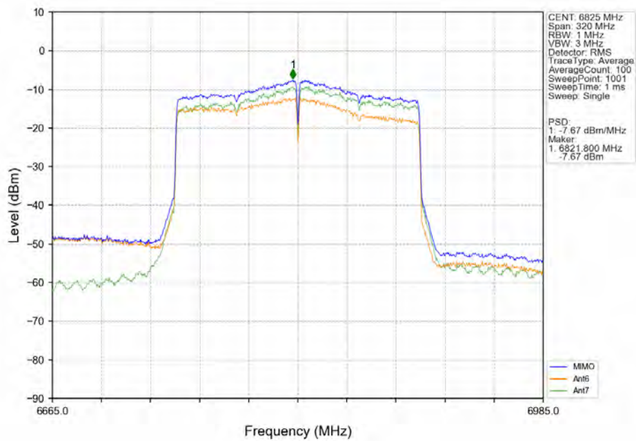
802.11ax(HEW160)_HCH_6825MHz_SU / MIMO_NTNV
