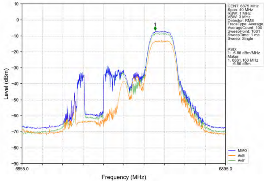
802.11ax(HEW20) HCH 6875MHz RU106 Right Ant6 NTN
