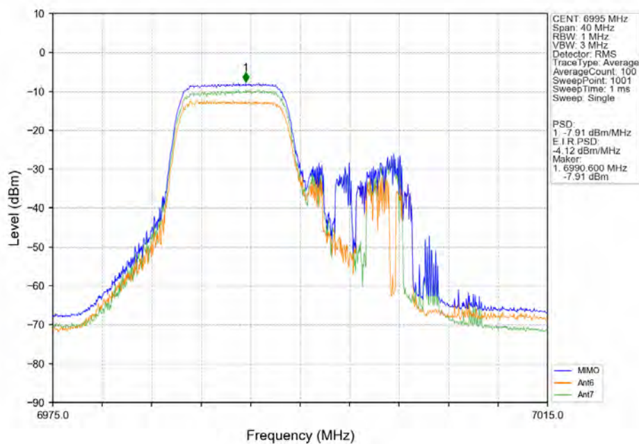
802.11ax(HEW20)_MCH_6995MHz_RU106_Left_MIMO_NTNV
