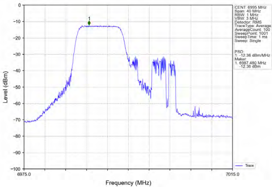
802.11ax(HEW20)_MCH_6995MHz_RU106_Left_Ant6_NTNV
