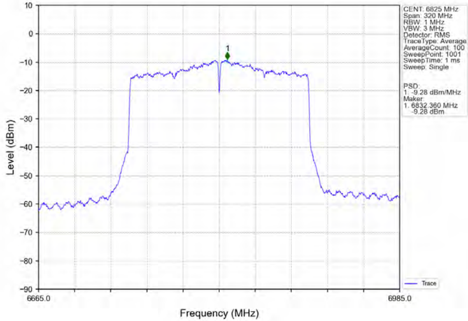
802.11ax(HEW160)_HCH_6825MHz_SU / MIMO_NTNV
