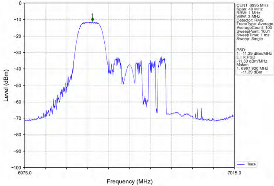
802.11ax(HEW20) MCH 6995MHz RU52 Left_Ant7_NTNV
