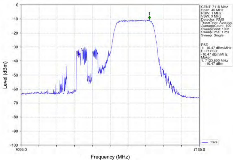
802.11ax(HEW20) HCH 7115MHz RU106 Right Ant6 NTN
