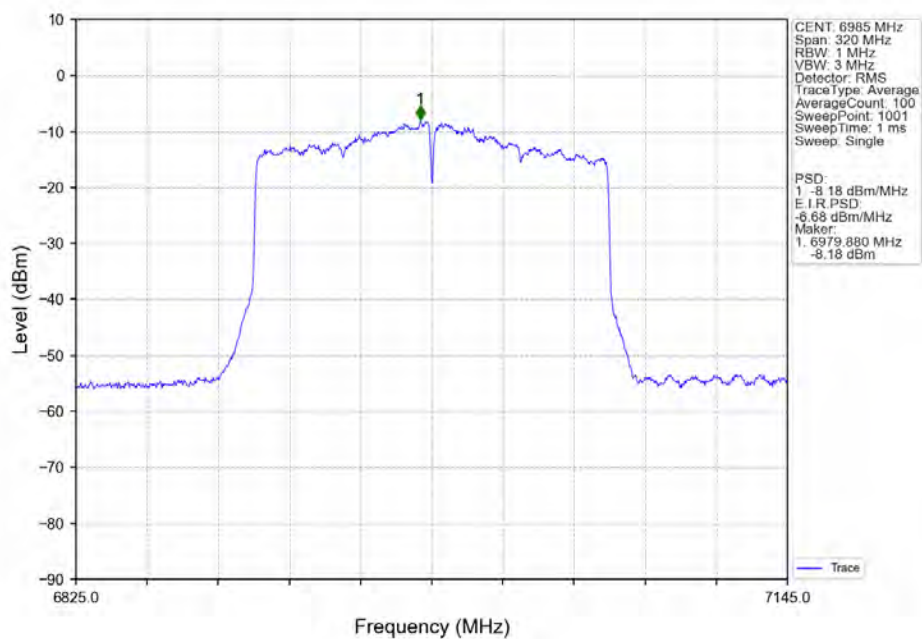
802.11ax(HEW160)_MCH_6985MHz_SU_/_Ant7_NTNV
