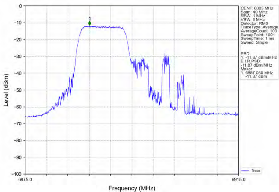
802.11ax(HEW20)_LCH_6895MHz_RU106_Left_Ant6_NTNV
