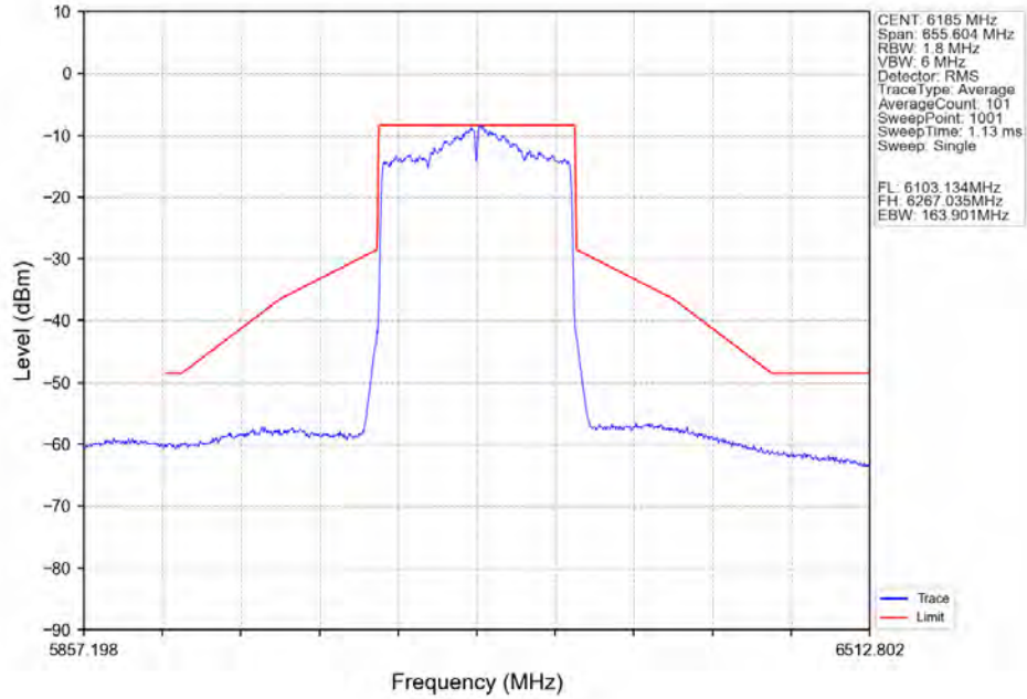
802.11ax(HEW160)_MCH_6185MHz_SU_/_Ant7_NTNV
