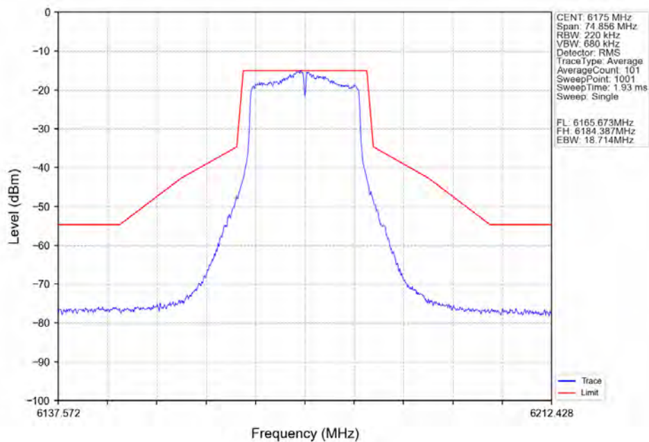
802.11a_MCH_6175MHz_Ant7_NTNV
