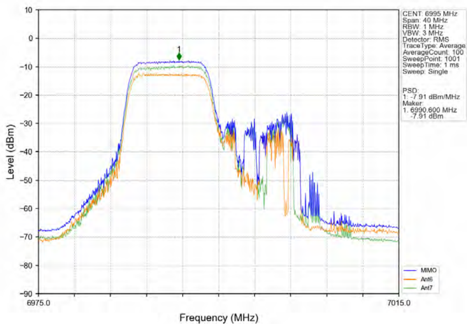
802.11ax(HEW20)_MCH_6995MHz_RU106_Left_MIMO_NTNV
