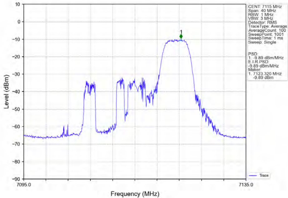
802.11ax(HEW20)_HCH_7115MHz_RU52_Right_Ant7_NTNV
