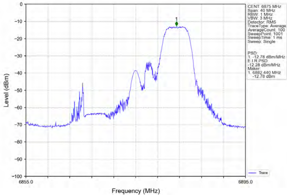
802.11ax(HEW20)_HCH_6875MHz_RU52_Right_Ant7_NTNV
