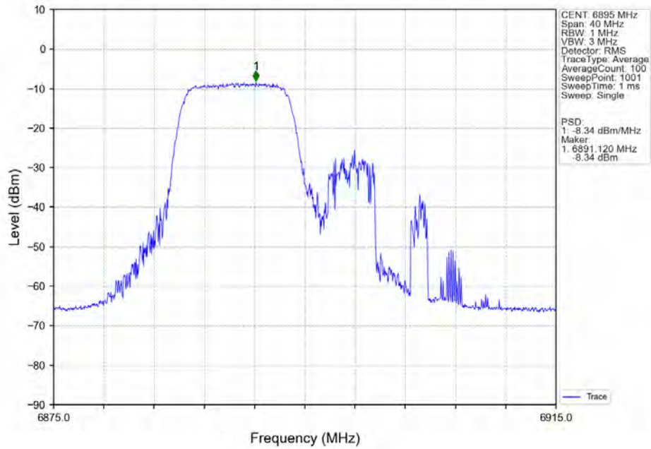
802.11ax(HEW20) LCH_6895MHz_RU106_Left_MIMO_NTNV
