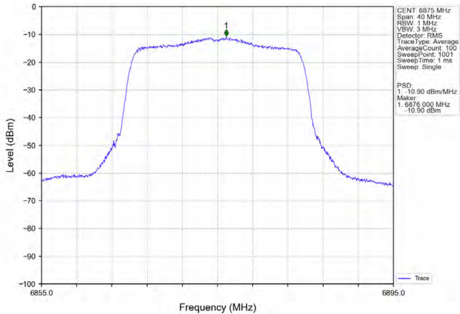
802.11ax(HEW20) HCH_6875MHz_SU / Ant7 NTN
