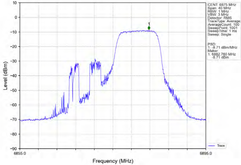
802.11ax(HEW20) HCH 6875MHz RU106 Right MIMO NTN
