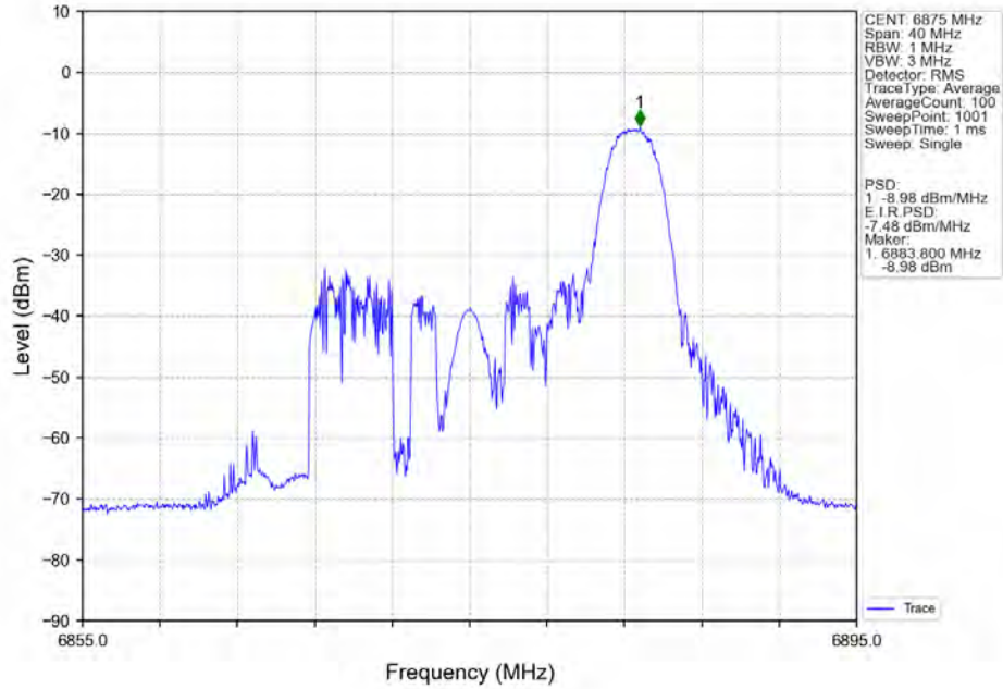
802.11ax(HEW20)_HCH_6875MHz_RU26_Right_MIMO_NTNV
