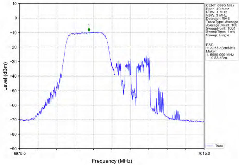
802.11ax(HEW20)_MCH_6995MHz_RU106_Left_MIMO_NTNV
