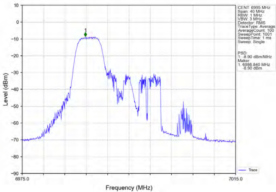
802.11ax(HEW20) MCH 6995MHz RU52 Left_Ant7_NTNV
