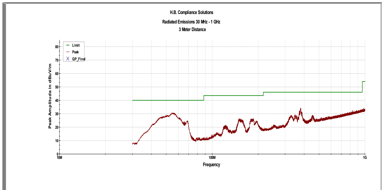
Plot 1 – Radiated Emissions – 30MHz to 1GHz – Idle Mode
