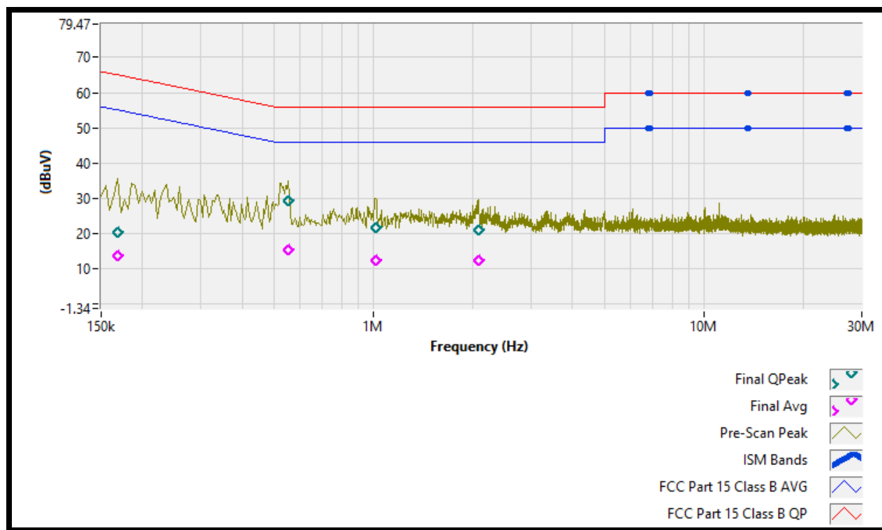
Plot 4 – Conducted Emissions – Neutral Side – Idle Mode
