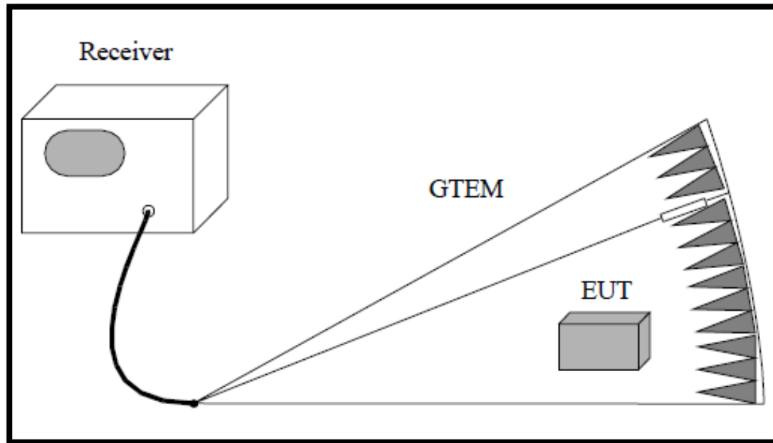
Figure 1. Radiated Emissions Test Setup (30MHz – 1GHz)
