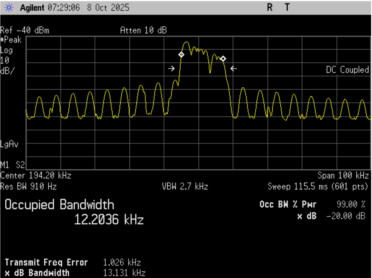
Plot 4 – 20dB BW
