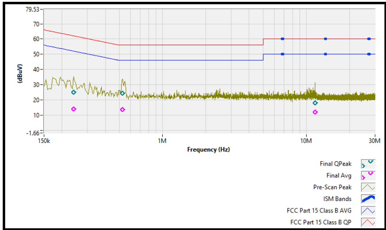
Plot 3 – Conducted Emission – Line Side – Idle Mode
