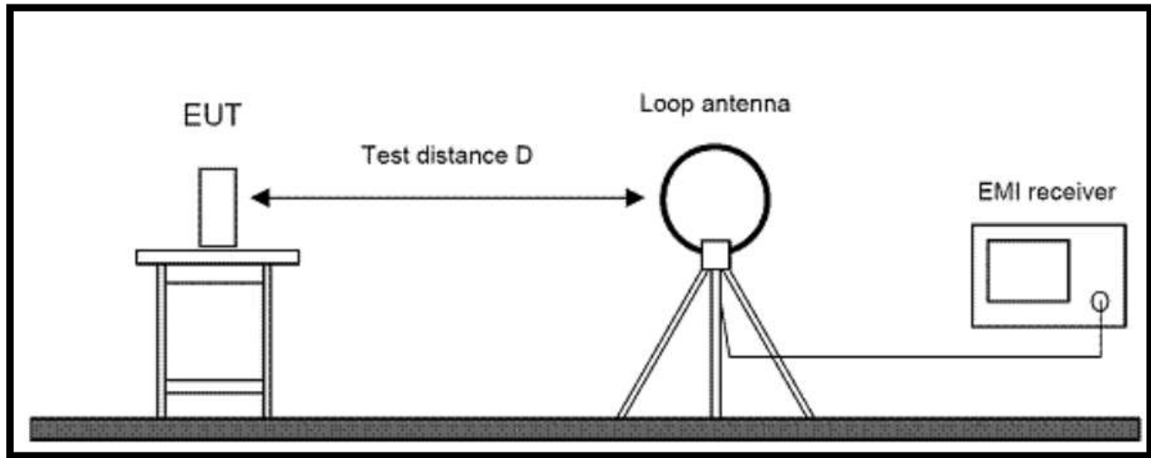
Figure 4. Radiated Emissions Test Setup (9kHz - 30MHz)
