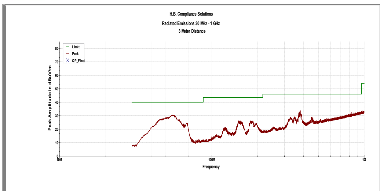
Plot 2 – Radiated Emissions – 30MHz to 1GHz – WPT Mode
