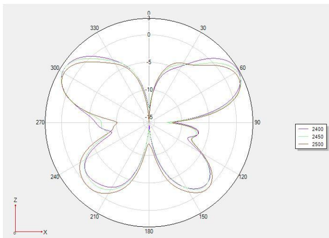
5-2 Antenna 2D Radiation Pattern
