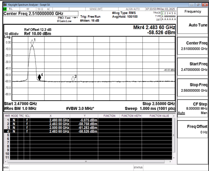
2DH5_Ant1_High_2480_Peak
