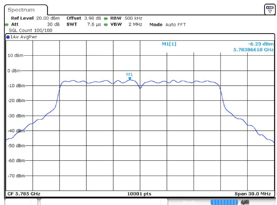
PSD ac20 5785MHz Ant2
