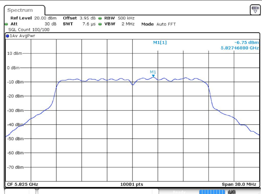
PSD ac20 5825MHz Ant2
