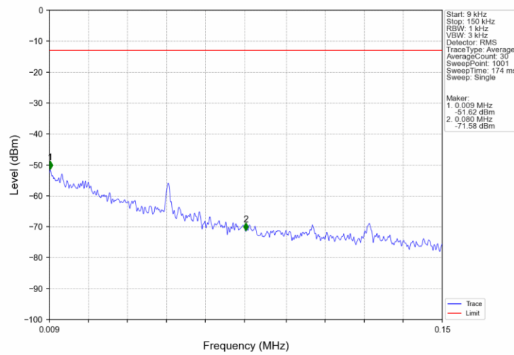
Band2_1.4MHz_16QAM_HCH_1909.3MHz_RB_1_0_NTNV
