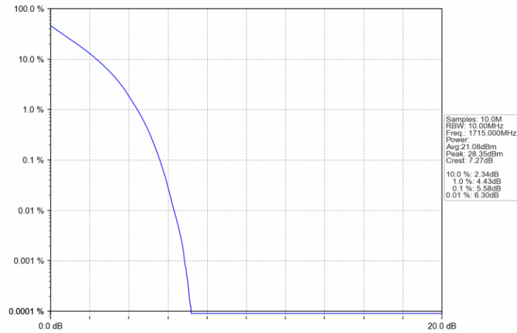
Band66 10MHz QPSK LCH 1715MHz RB 50 0 NTNV
