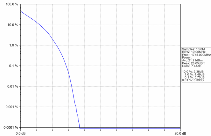
Band66 10MHz QPSK MCH 1745MHz RB 50 0 NTNV
