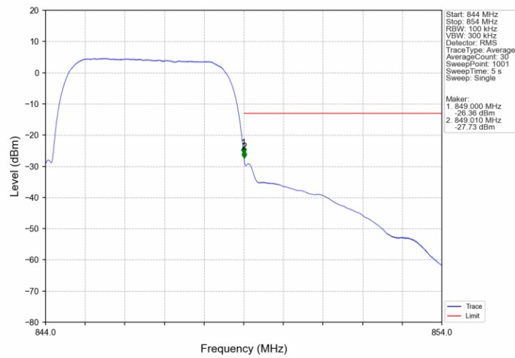
Band5_HSUPA_HCH_846.6MHz_Subtest 1_NTNV
