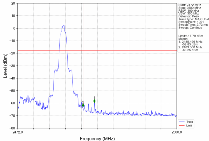
Pi/4DQPSK_2DH5_HCH_2480MHz_Ant1_NTNV
