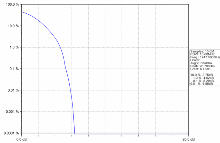
Band4_15MHz_QPSK_HCH_1747.5MHz_RB_75_0_NTNV
