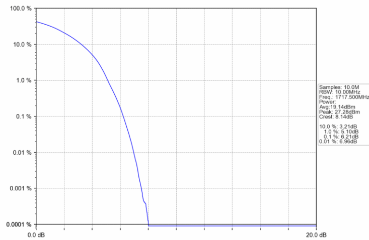
Band4_15MHz_16QAM_LCH_1717.5MHz_RB_75_0_NTNV
