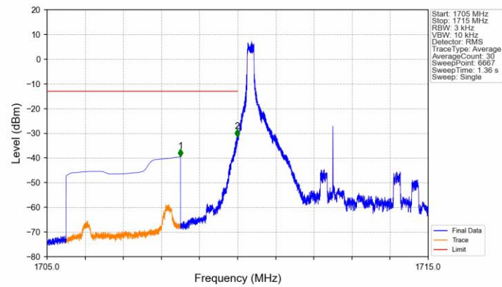
Band4_5MHz_QPSK_LCH_1712.5MHz_RB_1_0_NTNV
