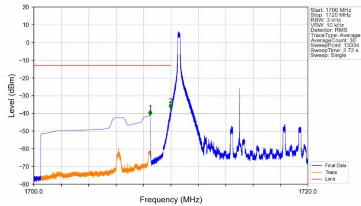
Band4_10MHz_QPSK_LCH_1715MHz_RB_1_0_NTNV
