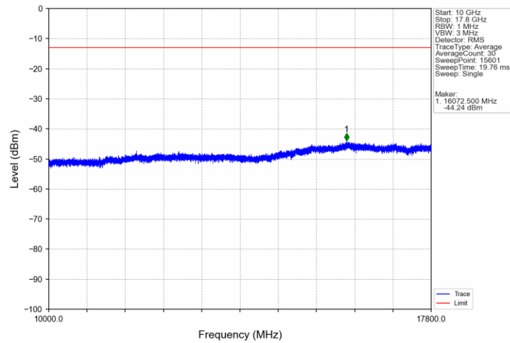
Band66_10MHz_16QAM_LCH_1715MHz_RB_50_0_NTNV
