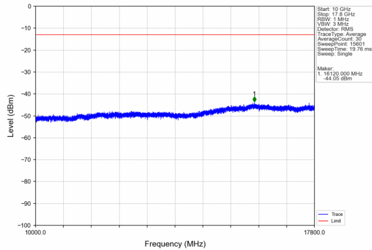
Band66_5MHz_16QAM_LCH_1712.5MHz_RB_25_0_NTNV
