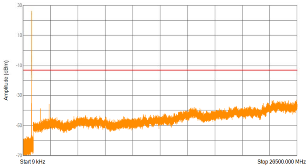
Band5 16QAM BW=5MHz Channel=20625 RB Size=1 Position=#0
