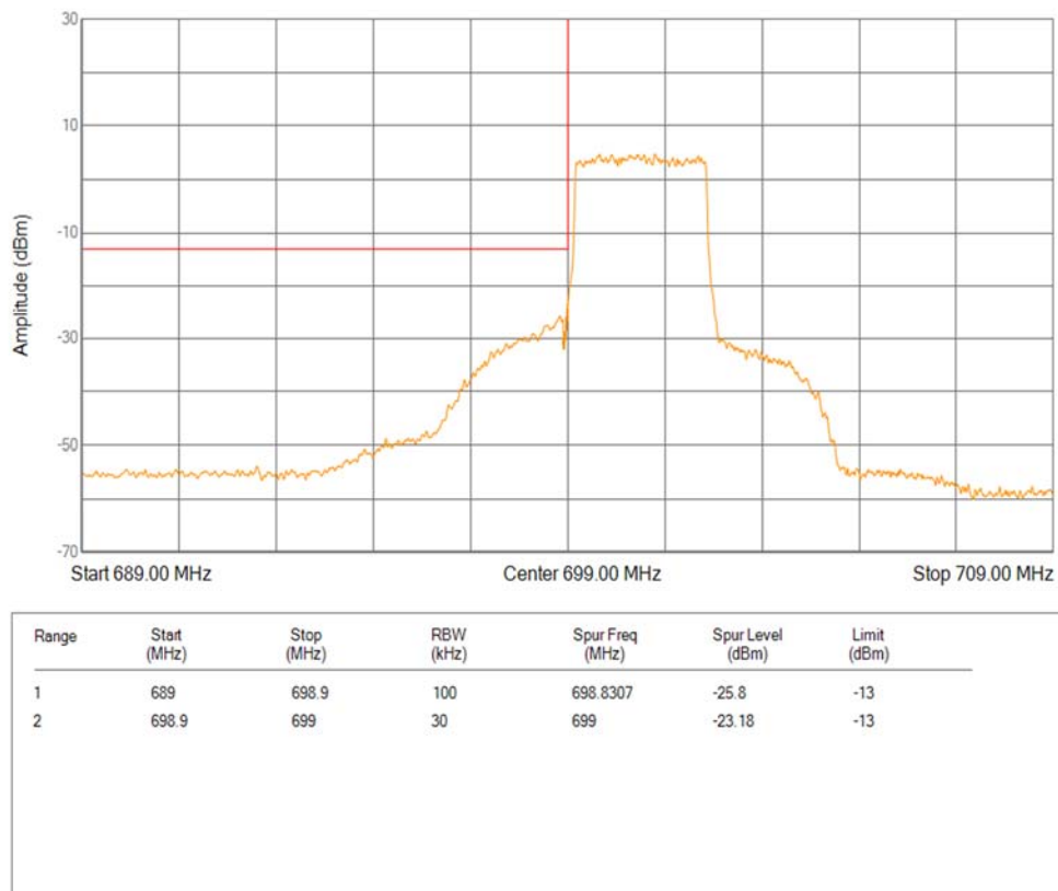
Band12 QPSK BW=3MHz Channel=23165 RB Size=1 Position=#0
