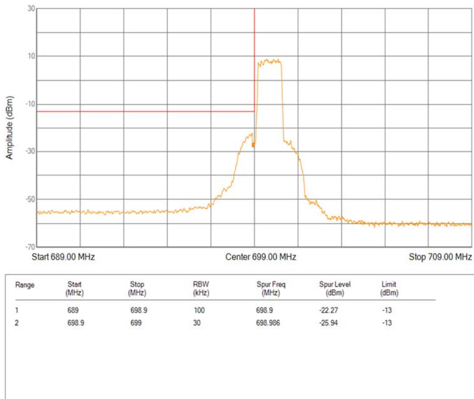
Band12 QPSK BW=1.4MHz Channel=23173 RB Size=1 Position=#0
