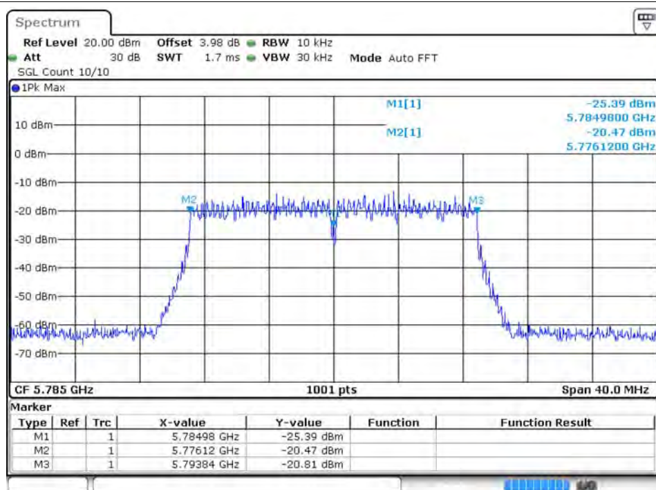
Freq. Stability 20C 120V n20 5785MHz Ant2
