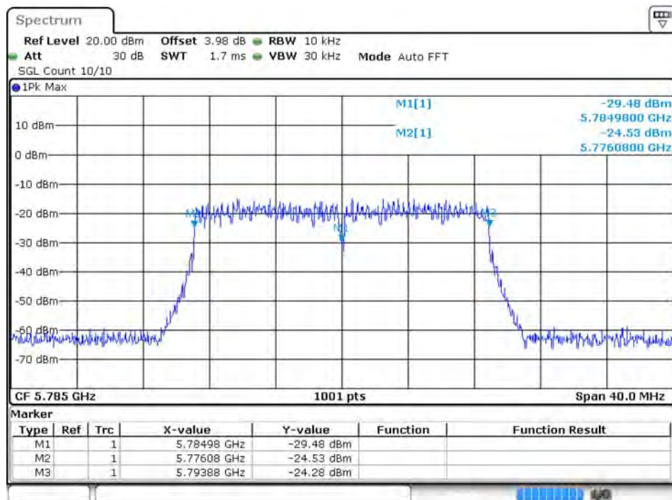
Freq. Stability 20C 102V n20 5785MHz Ant2
