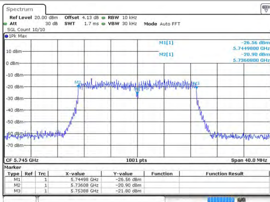
Freq. Stability 20C 120V n20 5745MHz Ant2
