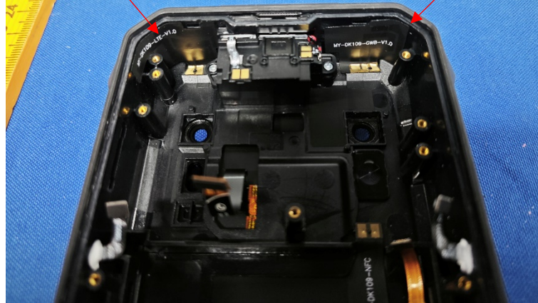
WLAN/BT antenna
