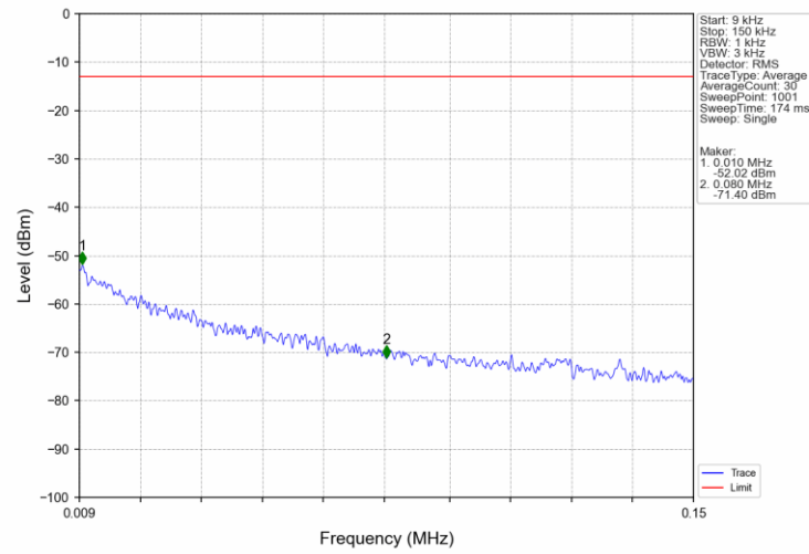
Band66 1.4MHz 16QAM LCH 1710.7MHz RB 1 0 NTN
