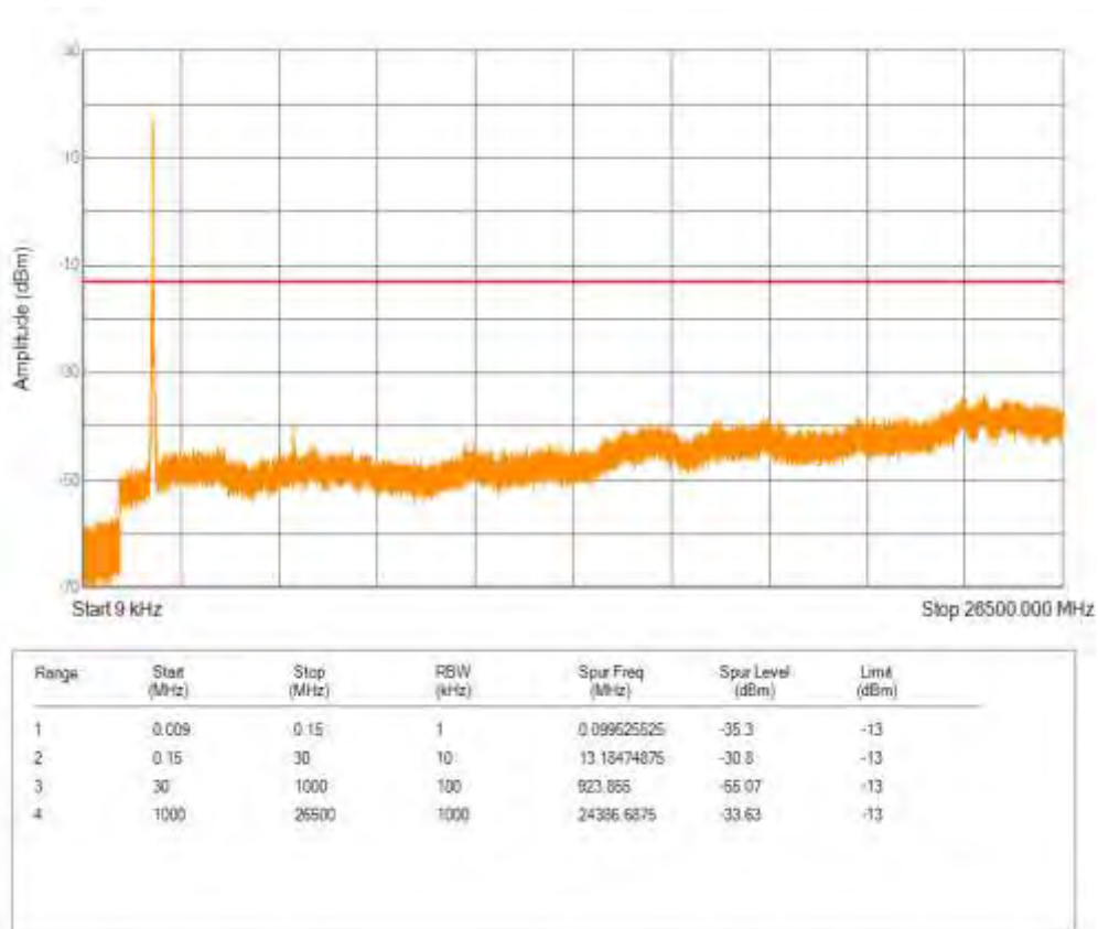
Band2 16QAM BW=3MHz Channel=18615 RB Size=15 Position=#0
