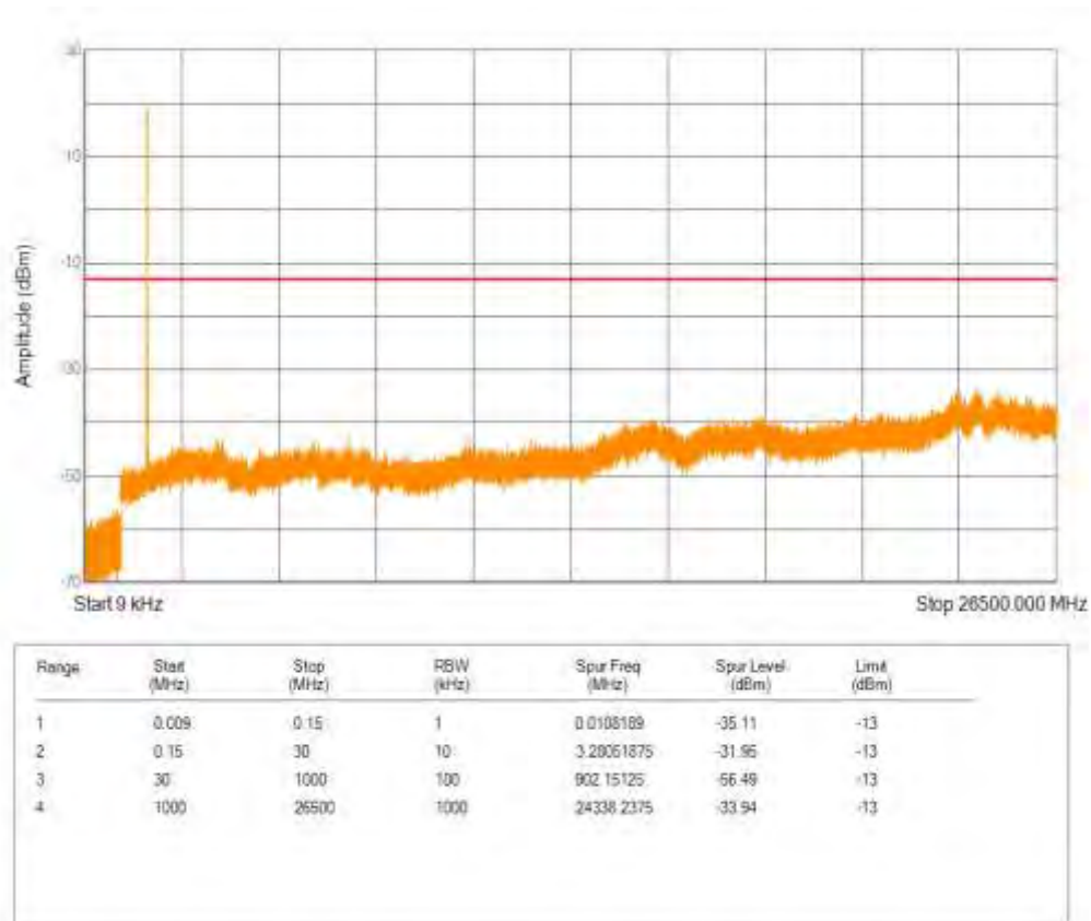
Band4 16QAM BW=10MHz Channel=20175 RB Size=50 Position=#0
