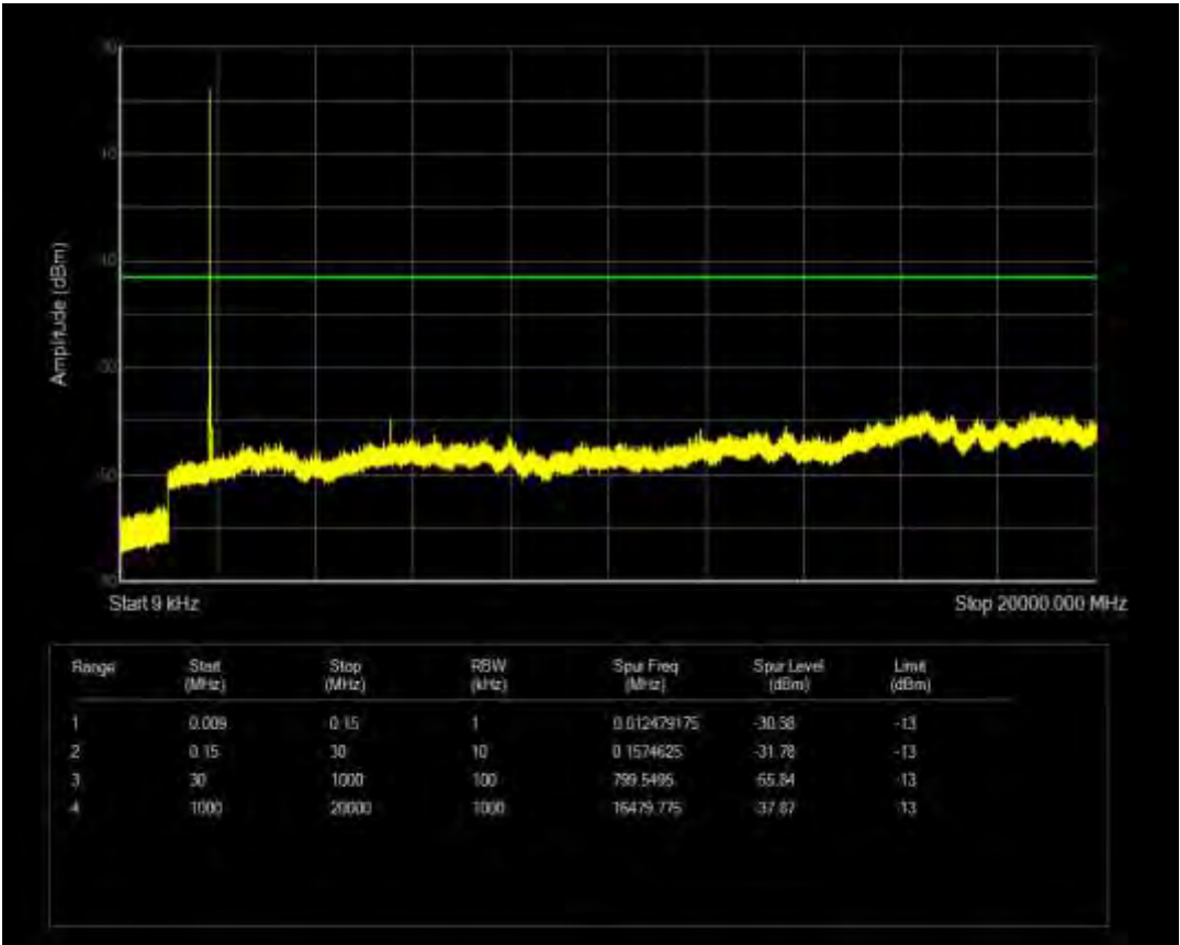
n2 SCS=15kHz CP QPSK BW=5MHz Channel=370500 RB=1@24
