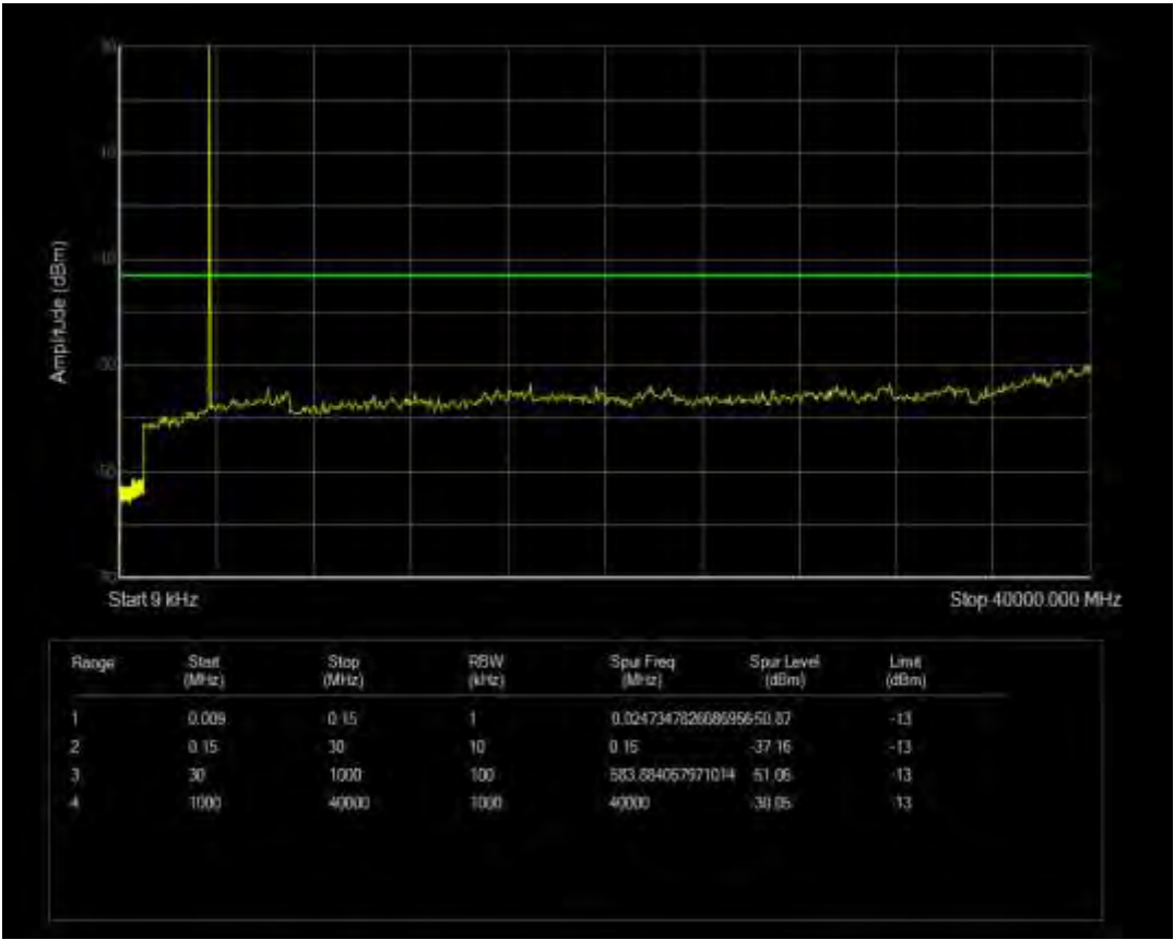
n78(3700-3800) SCS=30kHz CP QPSK BW=10MHz Channel=650000 RB=1@23
