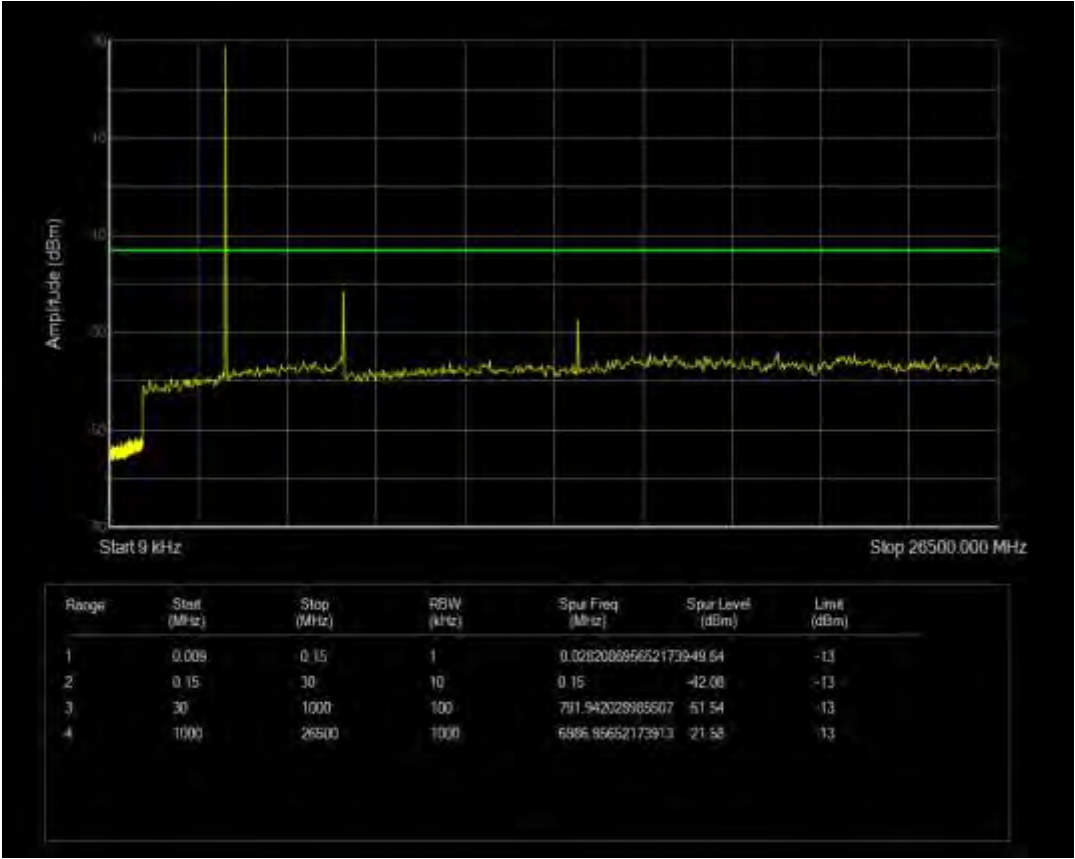
n77(3450-3550) SCS=30kHz CP QPSK BW=10MHz Channel=633334 RB=1@23
