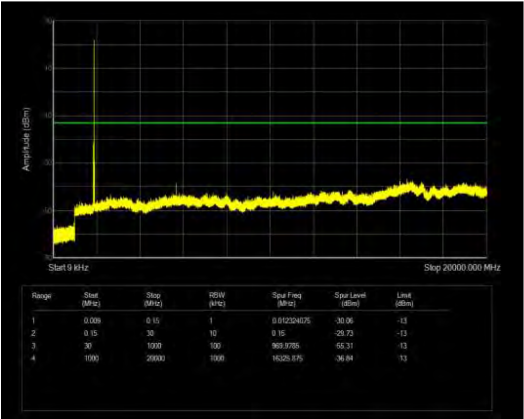
n2 SCS=15kHz CP QPSK BW=15MHz Channel=380500 RB=1@78
