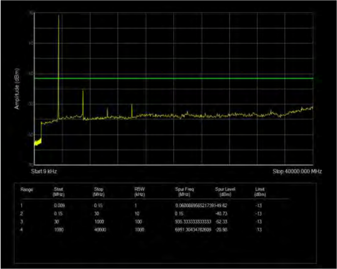
n77(3450-3550) SCS=30kHz CP QPSK BW=50MHz Channel=633334 RB=133@0
