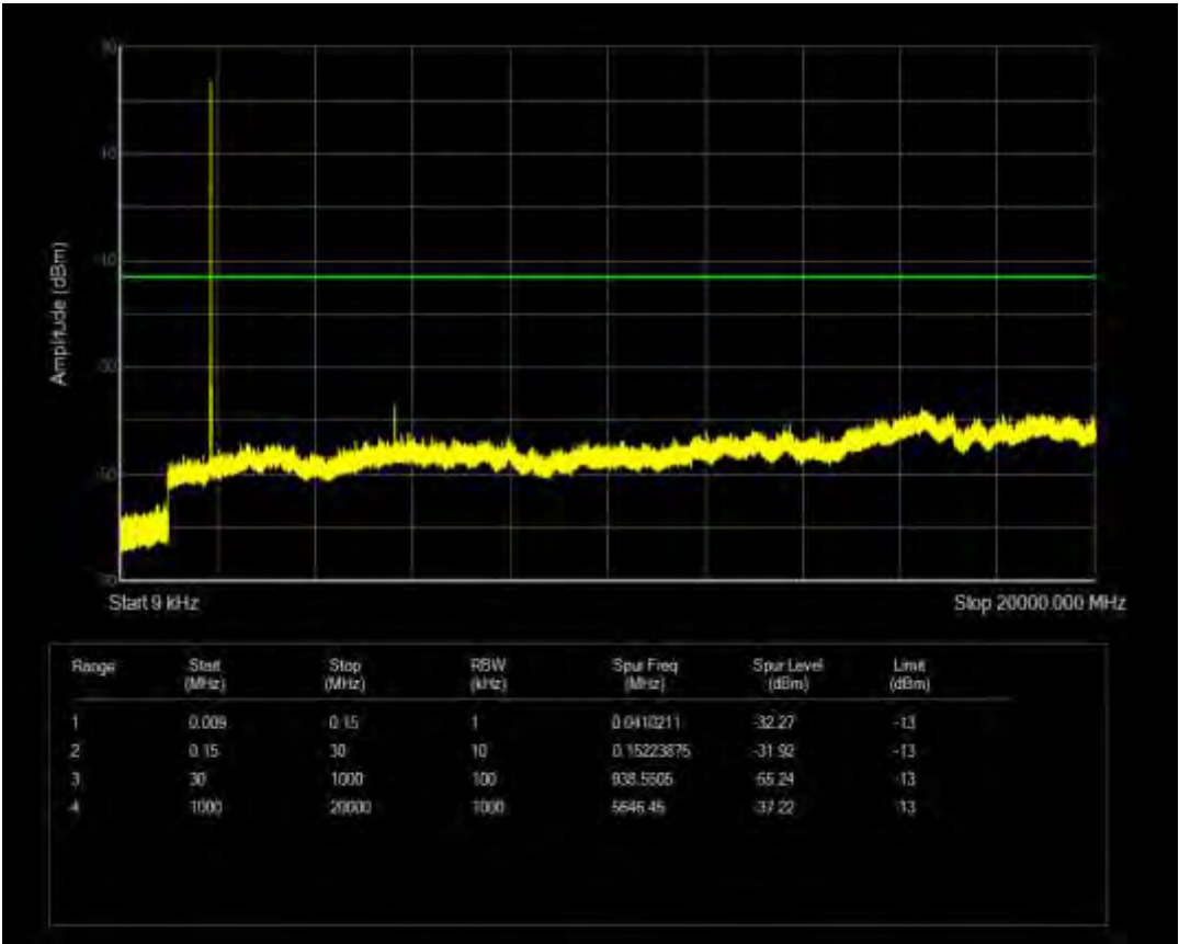
n2 SCS=15kHz CP QPSK BW=5MHz Channel=381500 RB=1@24
