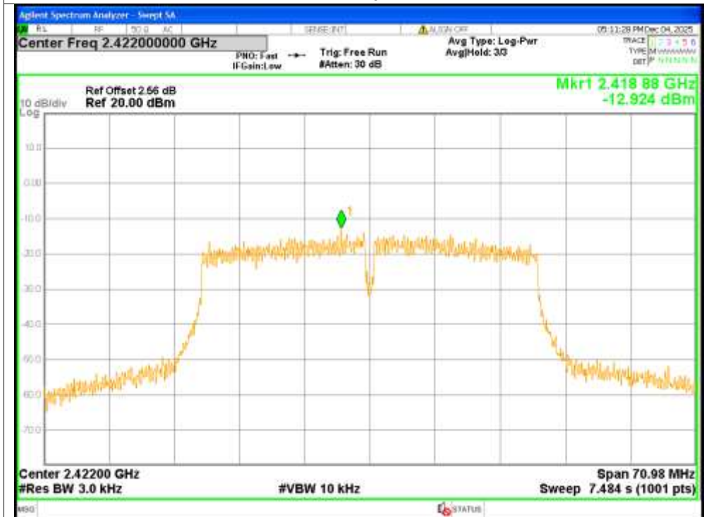
PSD NVNT n40 2422MHz
