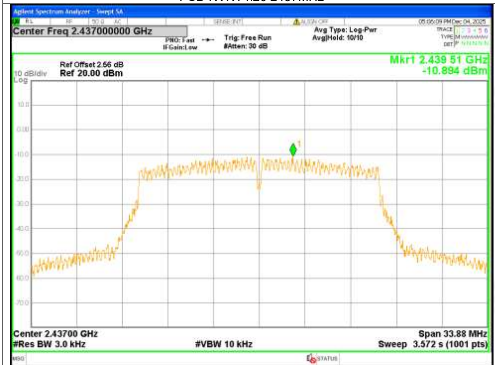
PSD NVNT n20 2437MHz
