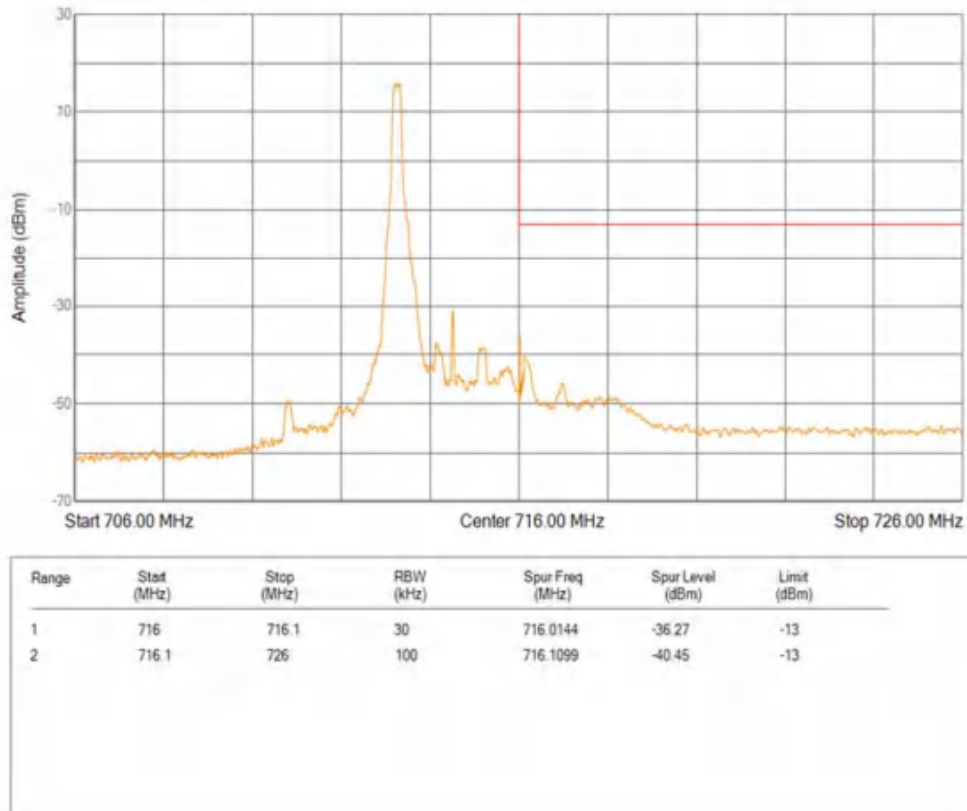
Band12 16QAM BW=3MHz Channel=23165 RB Size=1 Position=#Max
