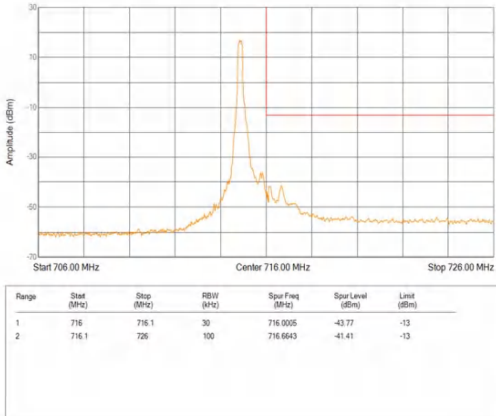
Band12 QPSK BW=1.4MHz Channel=23173 RB Size=1 Position=#Max
