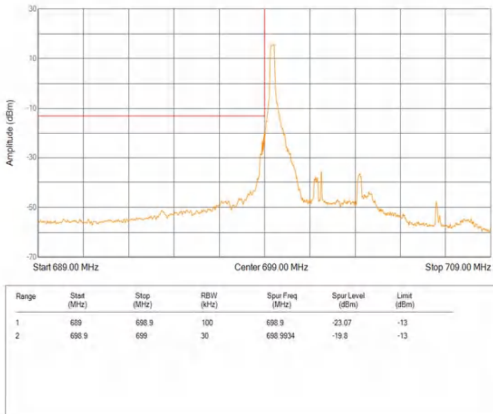
Band12 16QAM BW=5MHz Channel=23035 RB Size=1 Position=#Max
