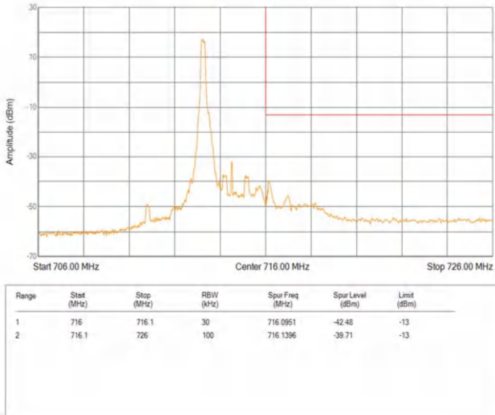
Band12 QPSK BW=3MHz Channel=23165 RB Size=1 Position=#Max
