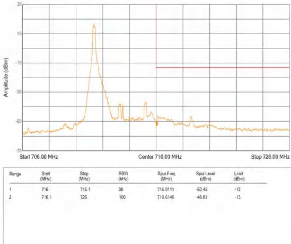
Band12 16QAM BW=5MHz Channel=23155 RB Size=1 Position=#Max
