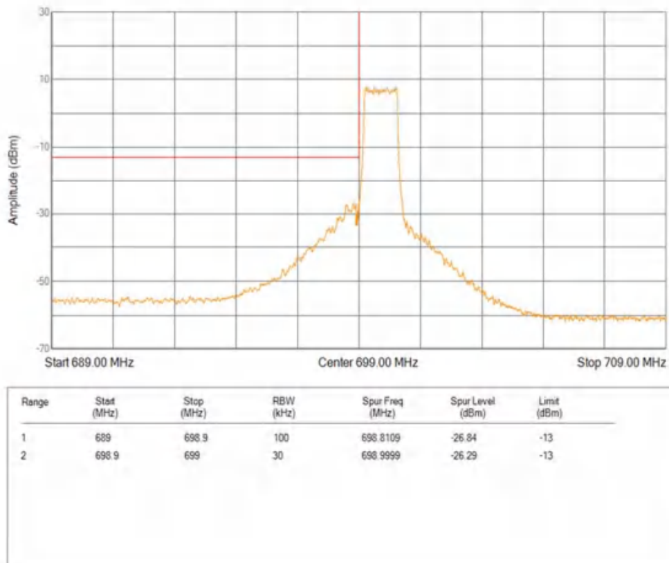
Band12 16QAM BW=1.4MHz Channel=23173 RB Size=1 Position=#0
