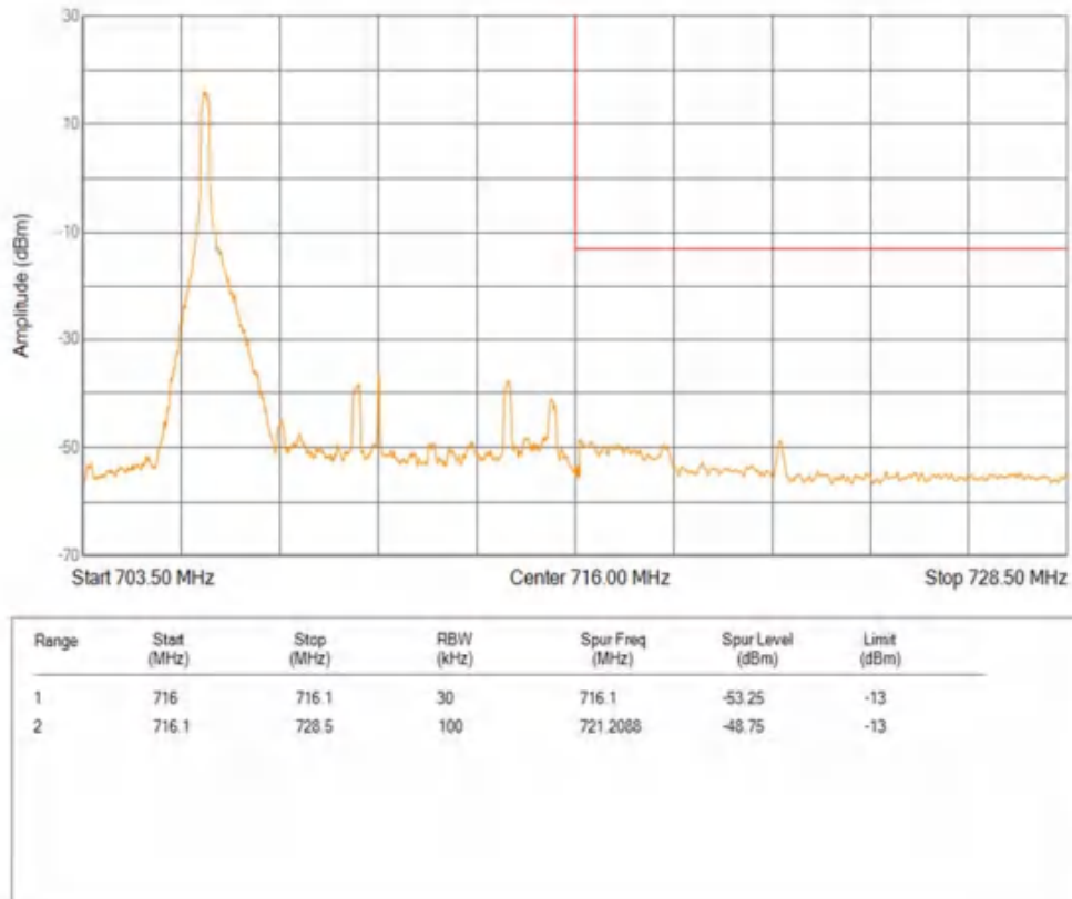
Band12 16QAM BW=10MHz Channel=23130 RB Size=1 Position=#Max
