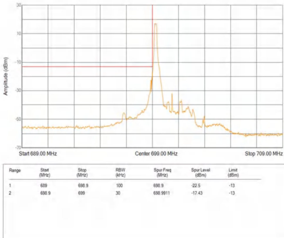
Band12 QPSK BW=3MHz Channel=23025 RB Size=1 Position=#Max
