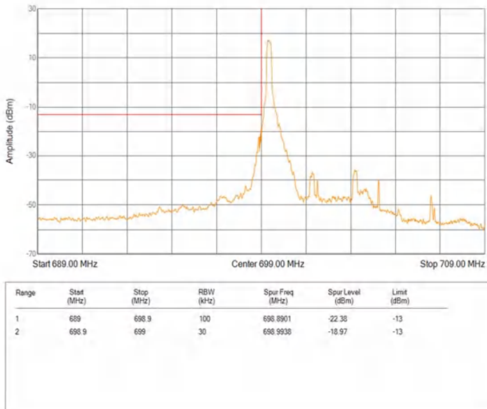
Band12 QPSK BW=5MHz Channel=23035 RB Size=1 Position=#Max
