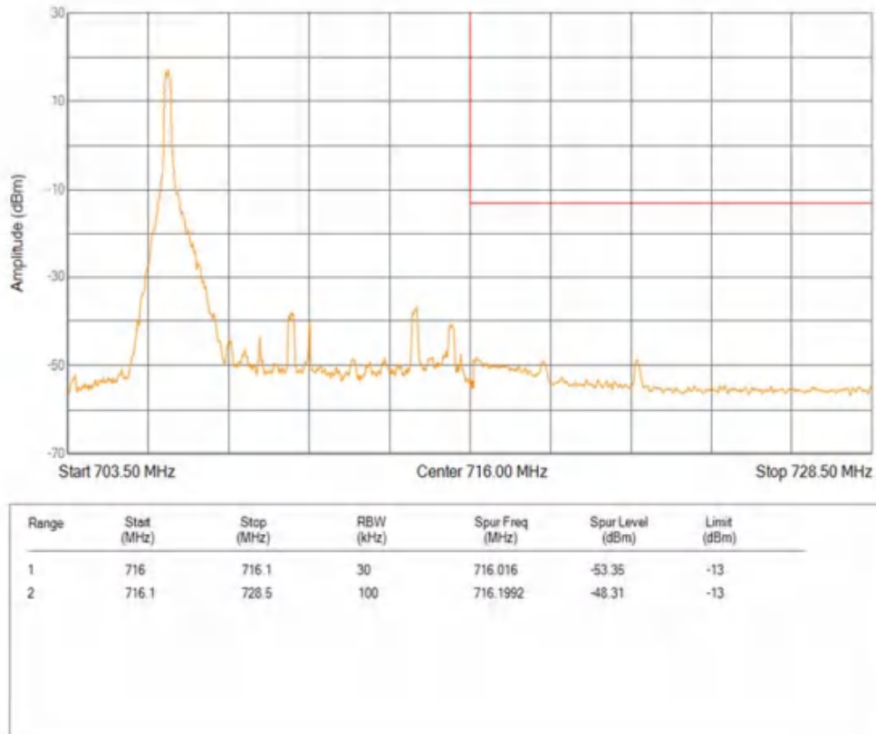
Band12 QPSK BW=10MHz Channel=23130 RB Size=1 Position=#Max
