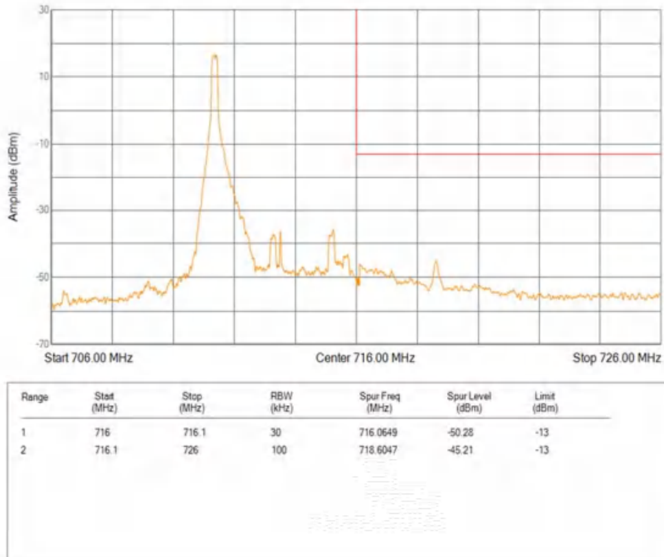
Band12 QPSK BW=5MHz Channel=23155 RB Size=1 Position=#Max
