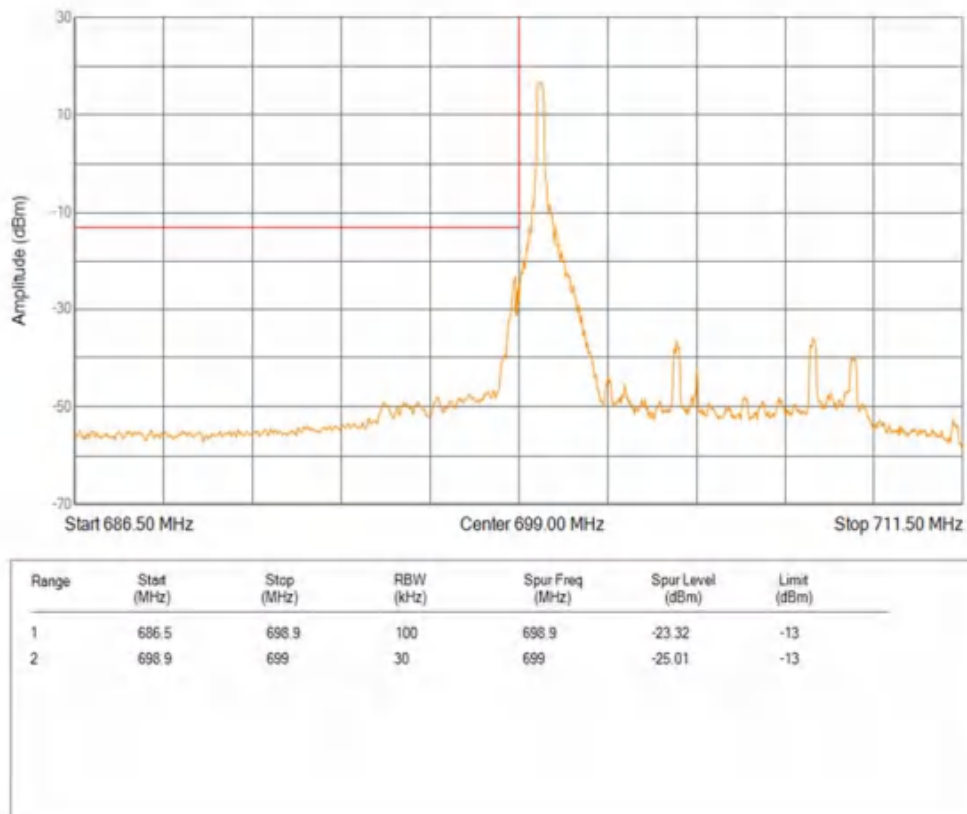
Band12 QPSK BW=10MHz Channel=23060 RB Size=1 Position=#Max
