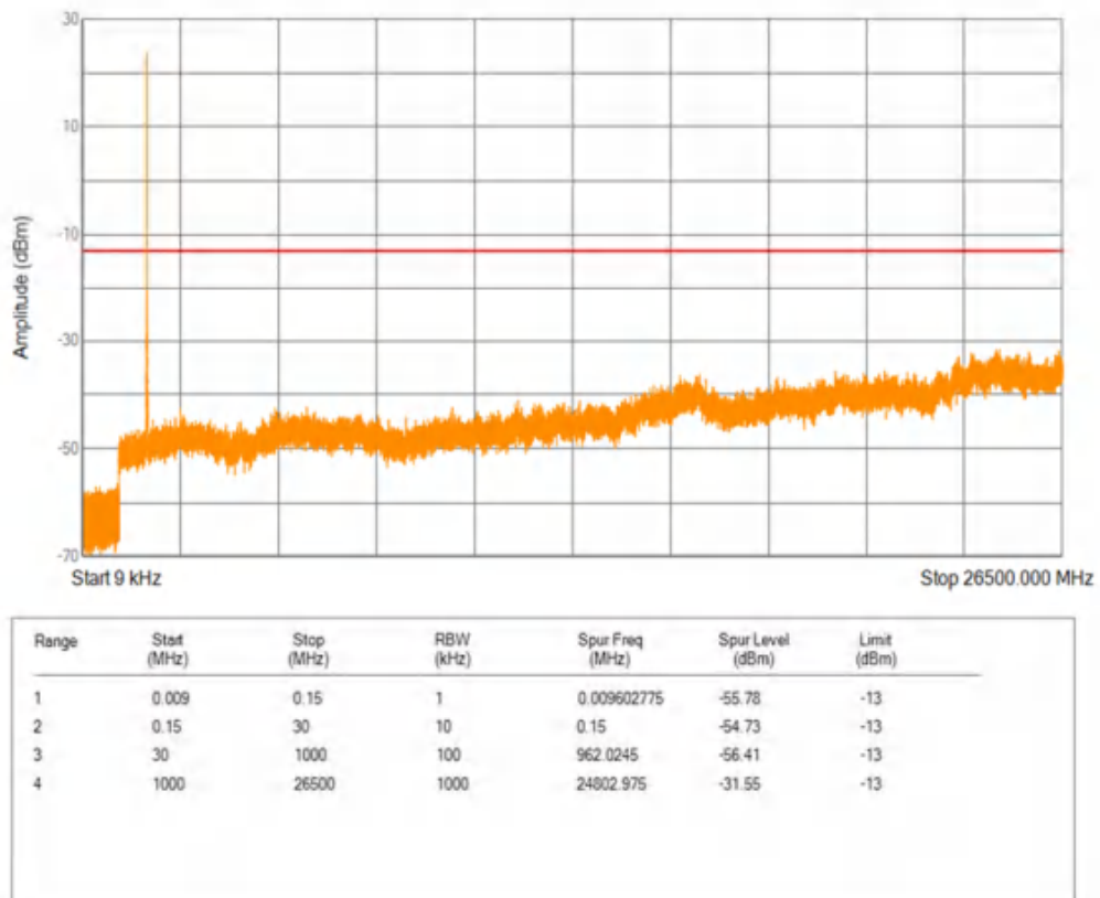
Band41 QPSK BW=5MHz Channel=39675 RB Size=1 Position=#0
