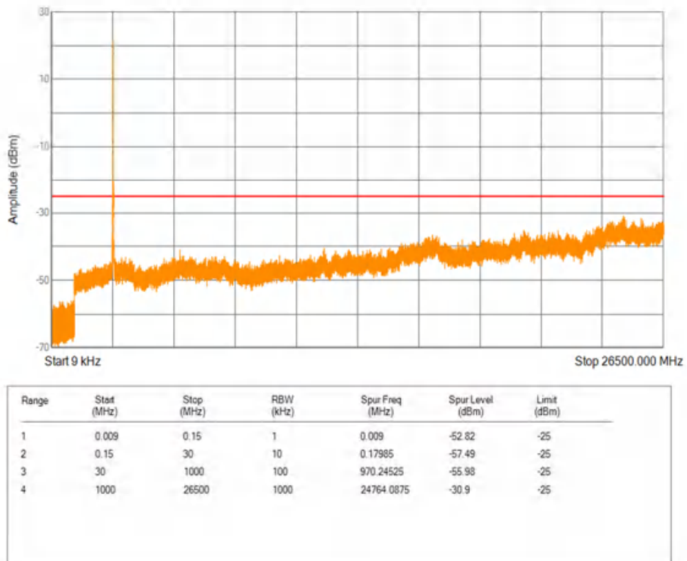
Band41 QPSK BW=20MHz Channel=39750 RB Size=1 Position=#0
