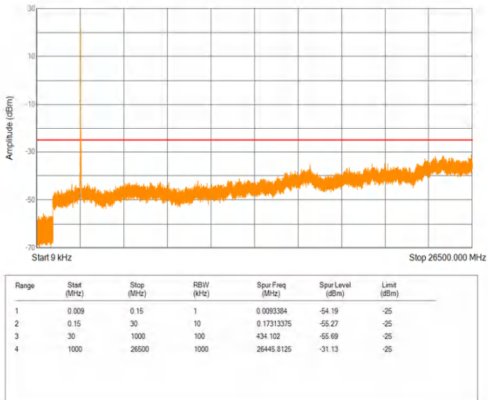
Band41 16QAM BW=15MHz Channel=41515 RB Size=1 Position=#0
