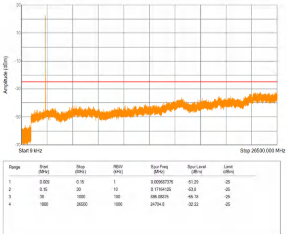
Band41 16QAM BW=5MHz Channel=39675 RB Size=1 Position=#0
