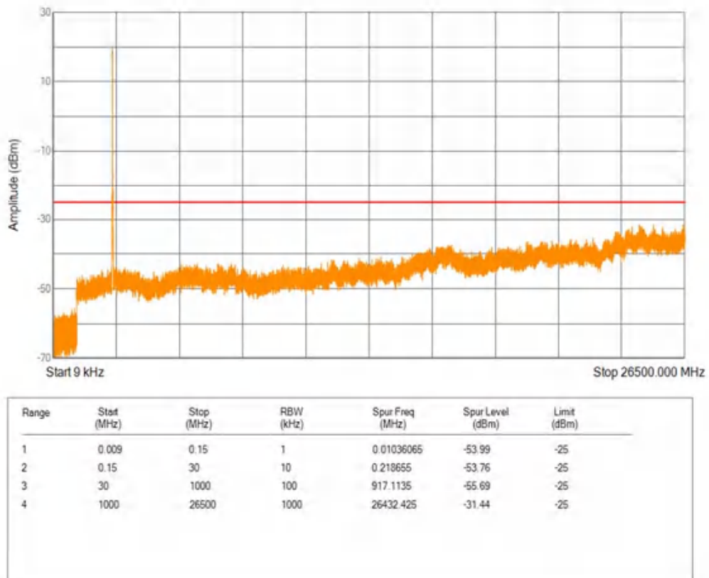
Band41 16QAM BW=15MHz Channel=39725 RB Size=1 Position=#0
