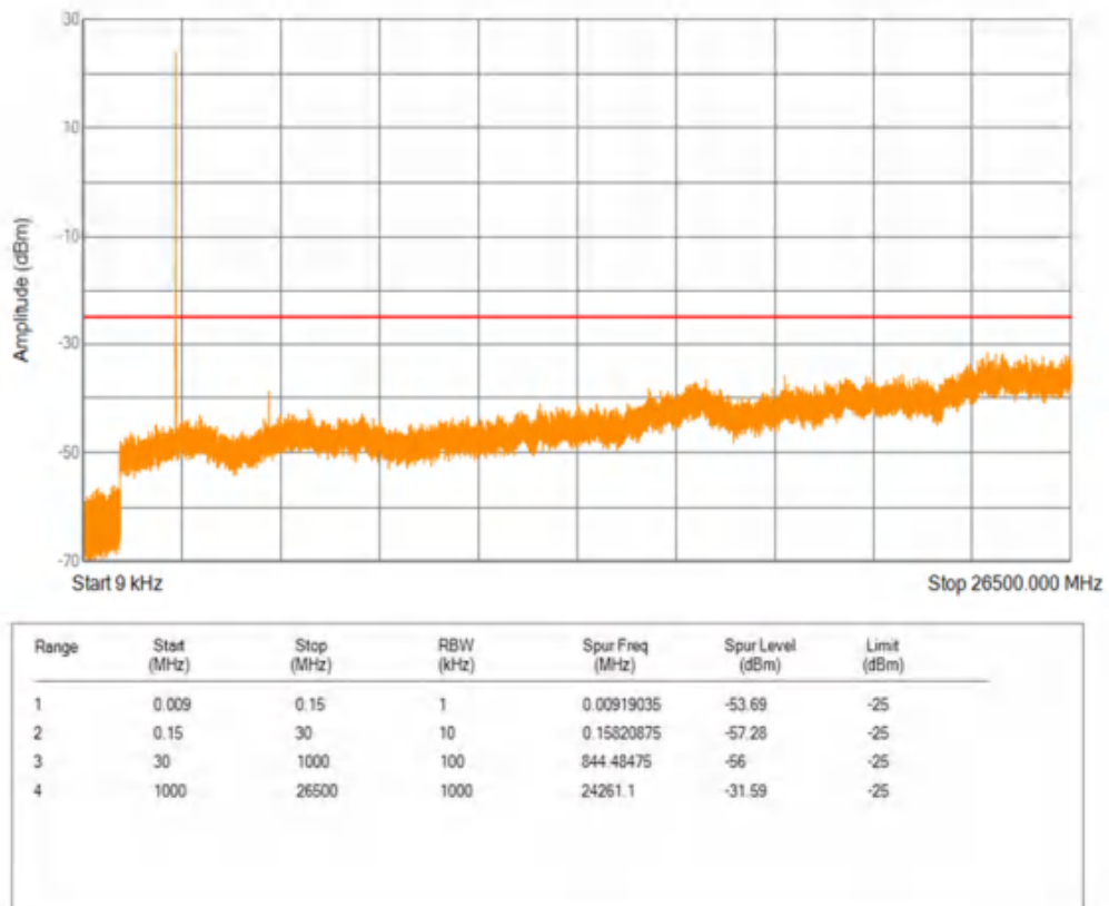
Band41 QPSK BW=5MHz Channel=41565 RB Size=1 Position=#0
