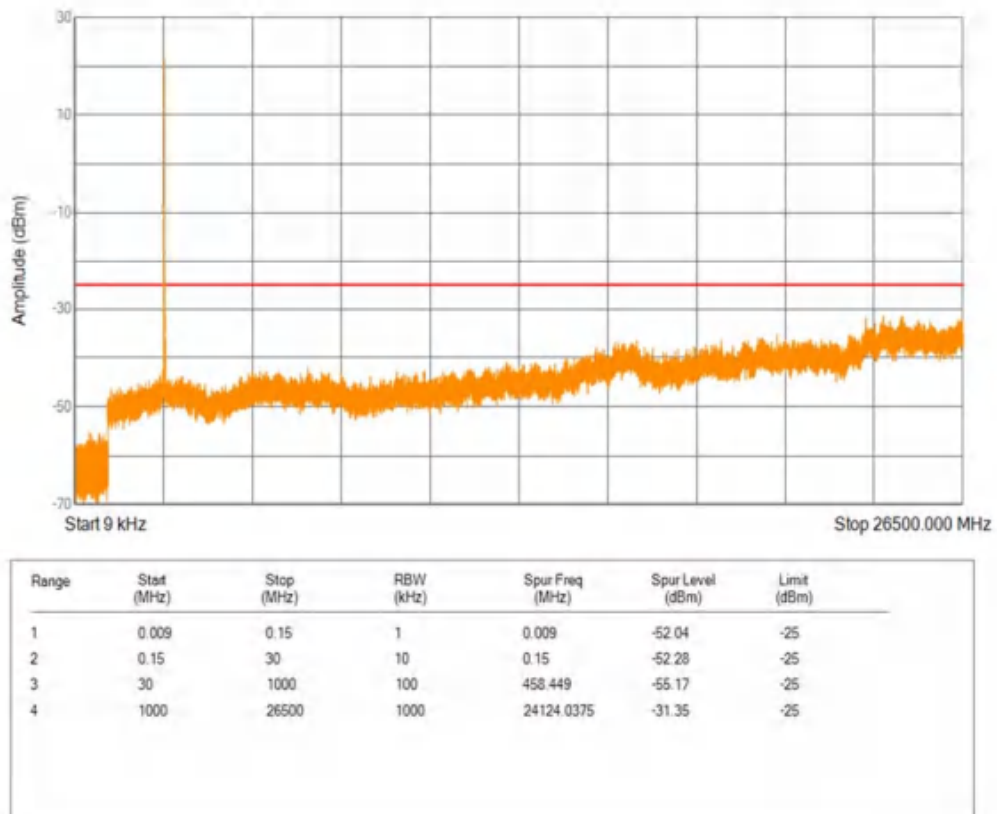
Band41 QPSK BW=15MHz Channel=39725 RB Size=1 Position=#0
