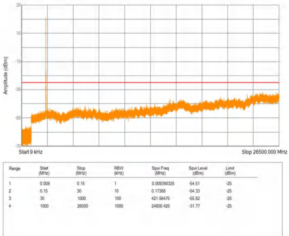
Band41 QPSK BW=10MHz Channel=41540 RB Size=1 Position=#0
