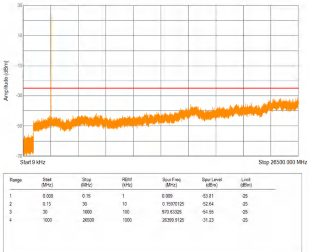
Band41 16QAM BW=5MHz Channel=41565 RB Size=1 Position=#0
