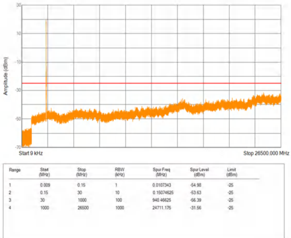
Band41 QPSK BW=15MHz Channel=41515 RB Size=1 Position=#0
