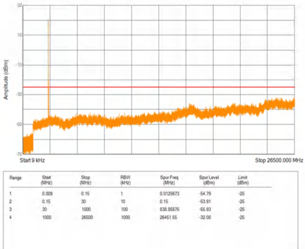
Band41 16QAM BW=10MHz Channel=39700 RB Size=1 Position=#0
