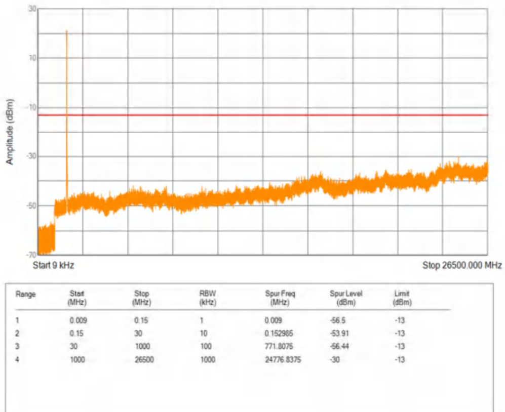
Band66 16QAM BW=10MHz Channel=132322 RB Size=1 Position=#0
