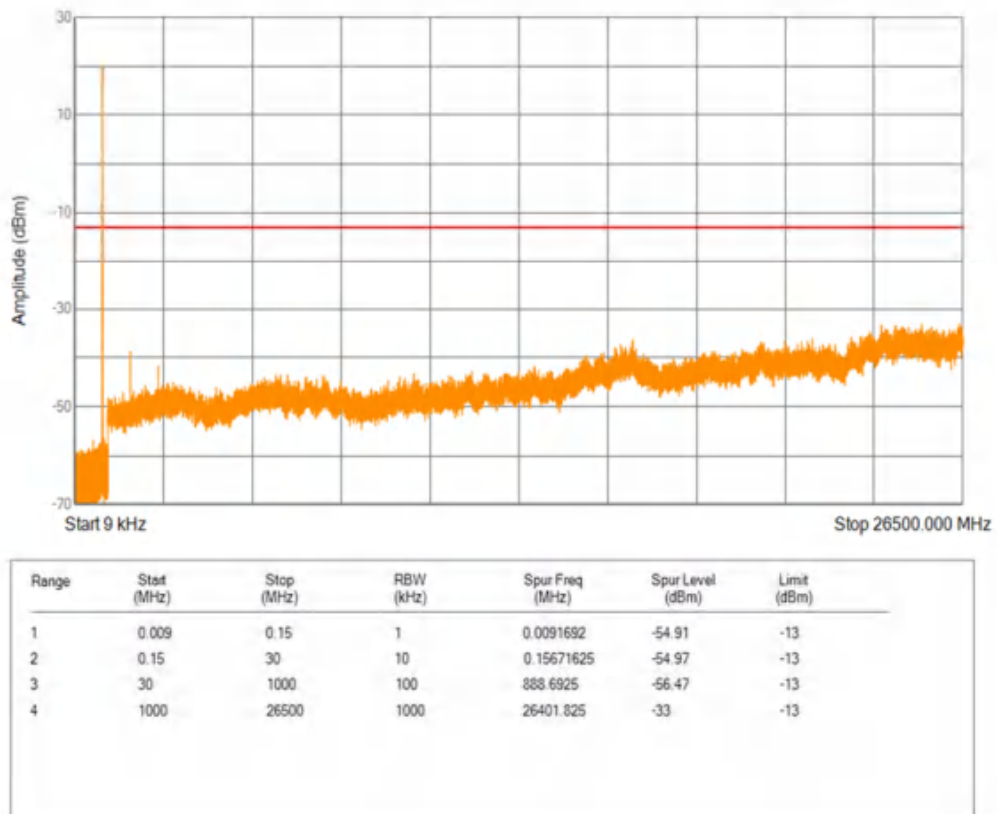
Band5 16QAM BW=1.4MHz Channel=20643 RB Size=1 Position=#0
