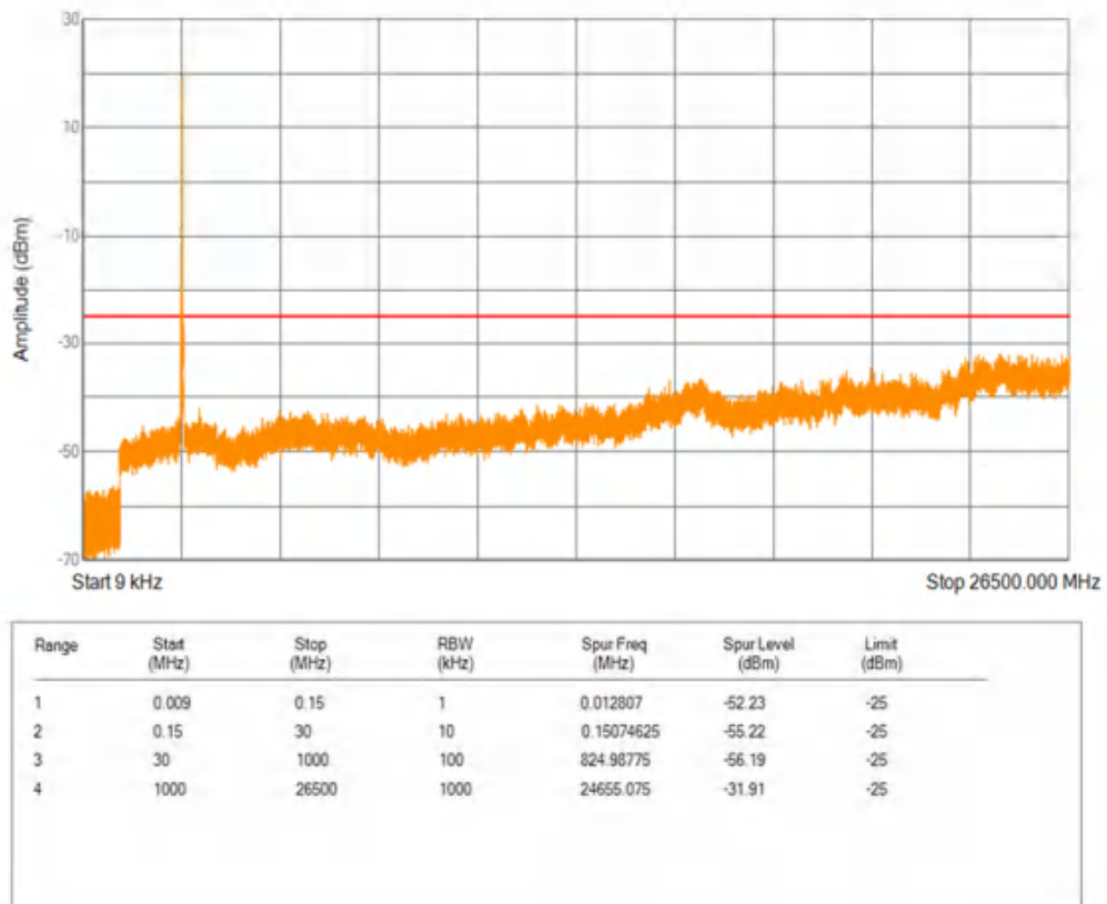
Band41 16QAM BW=20MHz Channel=41490 RB Size=1 Position=#0
