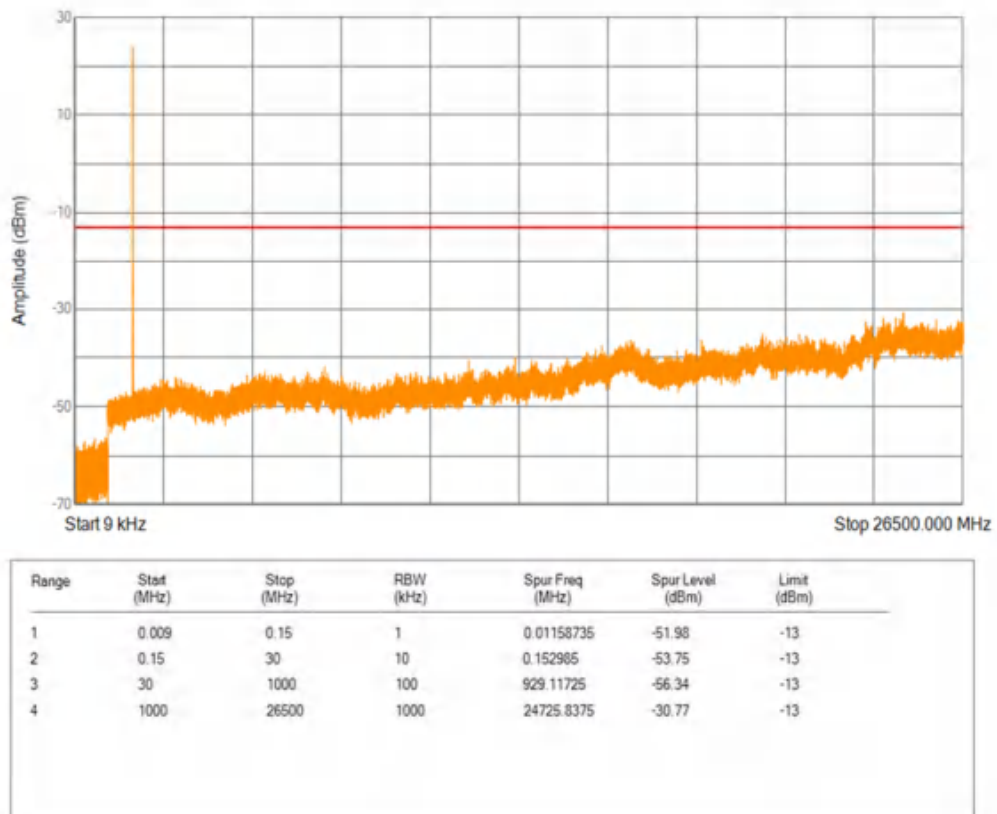
Band66 16QAM BW=3MHz Channel=132657 RB Size=1 Position=#0
