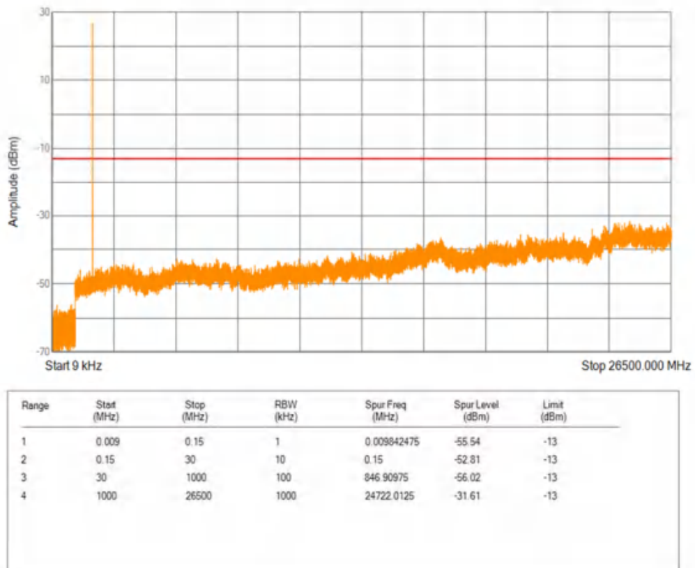
Band66 QPSK BW=1.4MHz Channel=132665 RB Size=1 Position=#0
