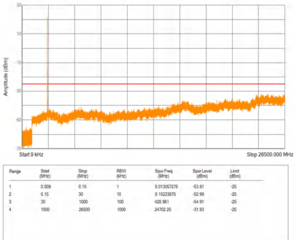
Band7 16QAM BW=15MHz Channel=20825 RB Size=1 Position=#0
