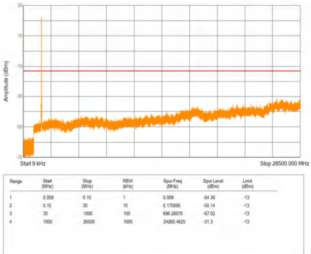
Band66 QPSK BW=10MHz Channel=132622 RB Size=1 Position=#0
