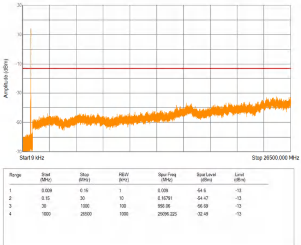
Band5 16QAM BW=5MHz Channel=20525 RB Size=1 Position=#0
