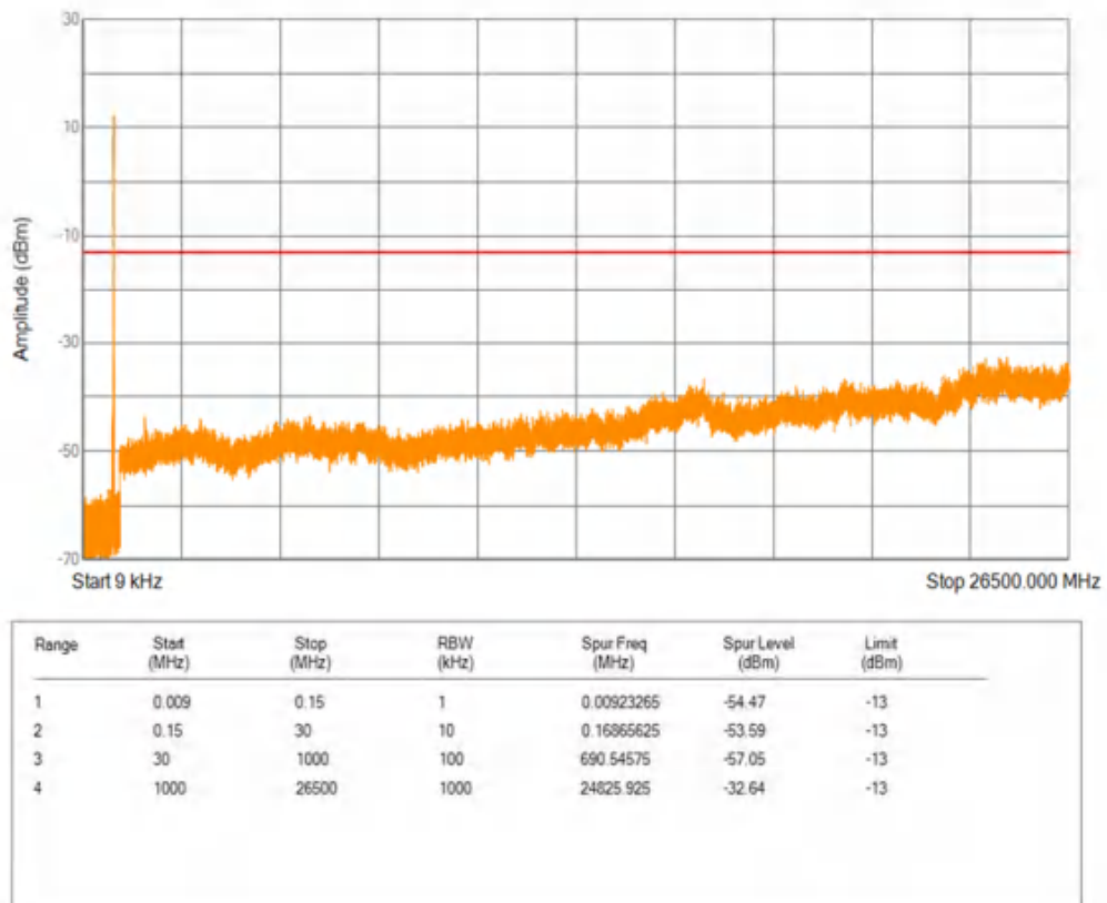
Band5 16QAM BW=10MHz Channel=20600 RB Size=1 Position=#0
