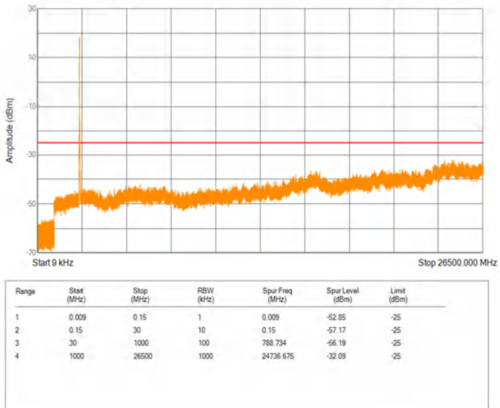
Band7 QPSK BW=20MHz Channel=21350 RB Size=1 Position=#0
