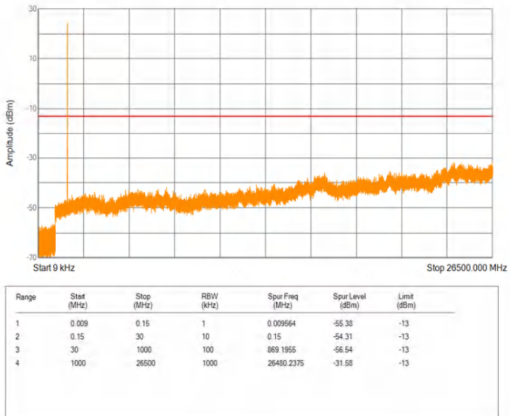
Band66 16QAM BW=3MHz Channel=132322 RB Size=1 Position=#0
