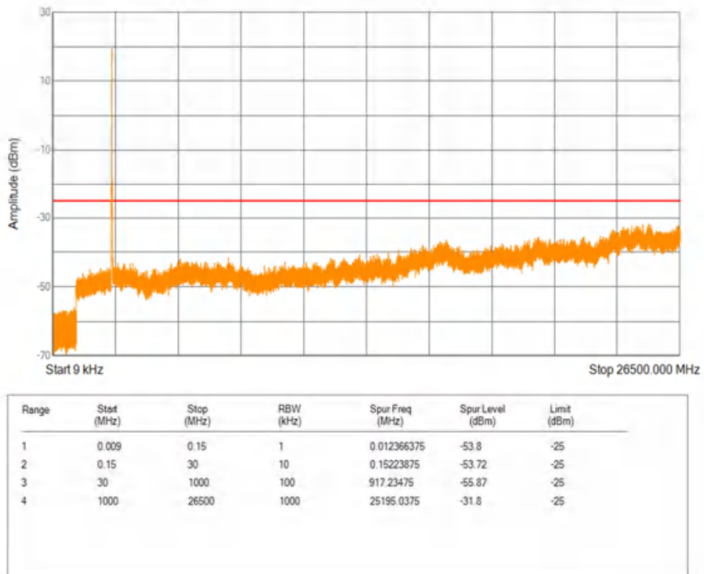
Band7 QPSK BW=15MHz Channel=21375 RB Size=1 Position=#0
