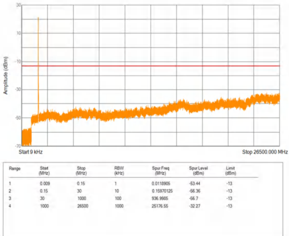
Band66 QPSK BW=10MHz Channel=132322 RB Size=1 Position=#0
