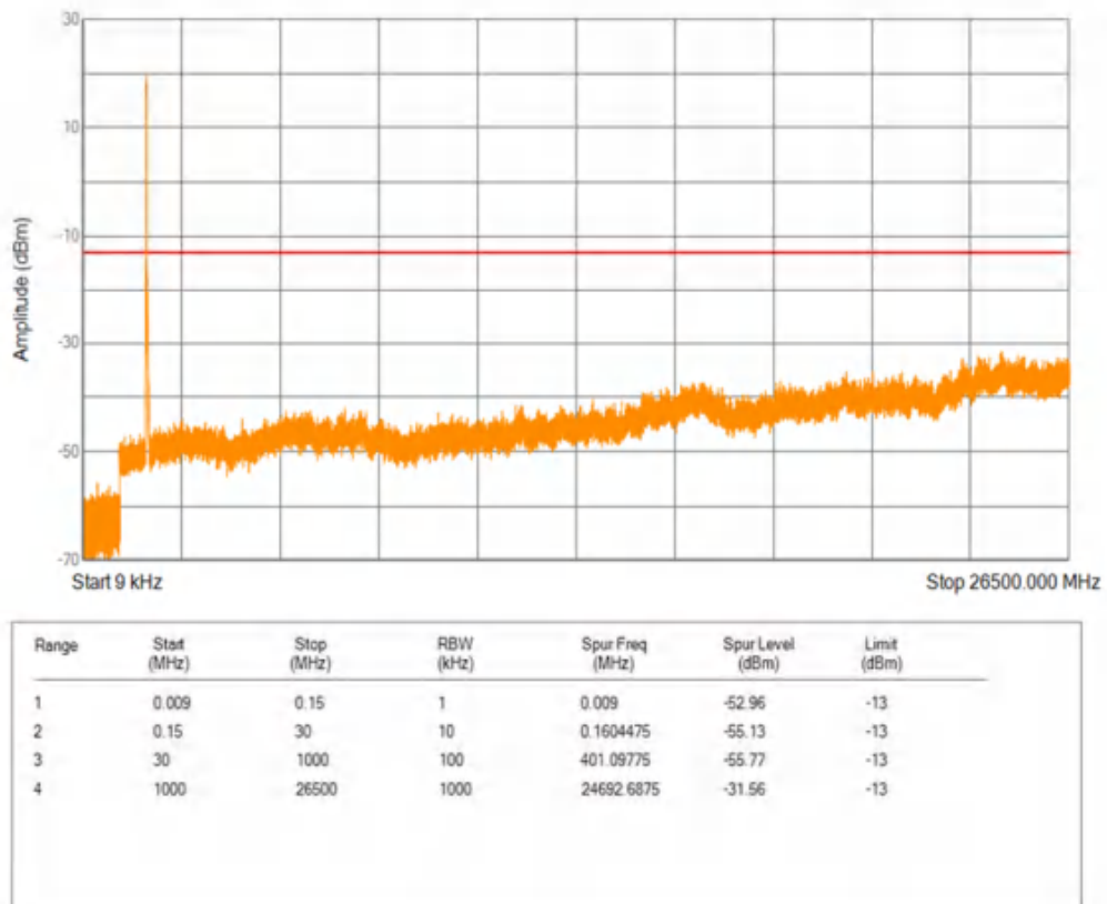
Band66 16QAM BW=20MHz Channel=132322 RB Size=1 Position=#0
