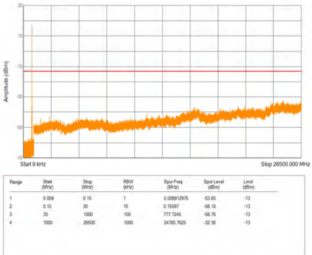
Band5 16QAM BW=3MHz Channel=20525 RB Size=1 Position=#0
