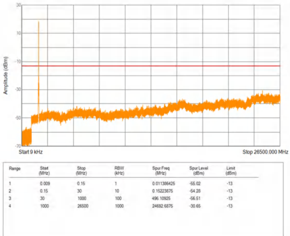
Band66 16QAM BW=20MHz Channel=132572 RB Size=1 Position=#0
