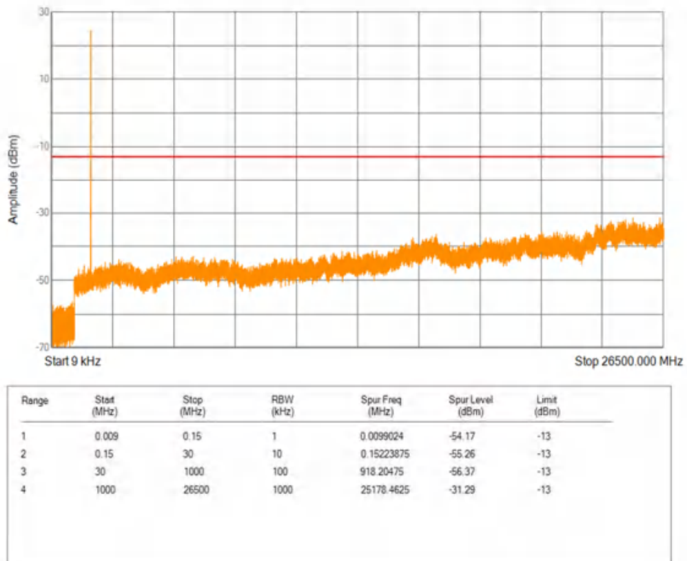
Band66 QPSK BW=3MHz Channel=132322 RB Size=1 Position=#0
