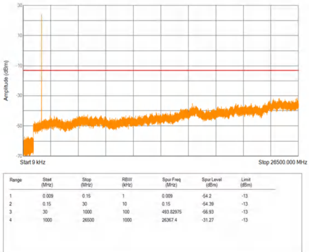
Band66 QPSK BW=5MHz Channel=131997 RB Size=1 Position=#0
