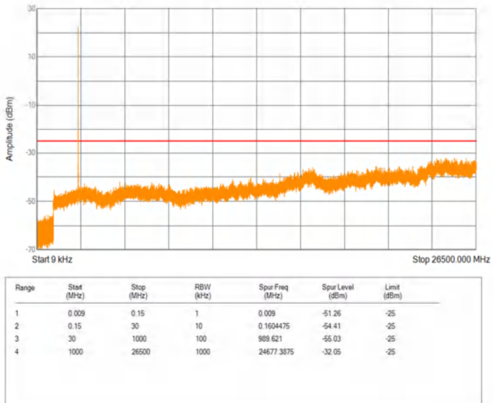
Band7 16QAM BW=5MHz Channel=21425 RB Size=1 Position=#0
