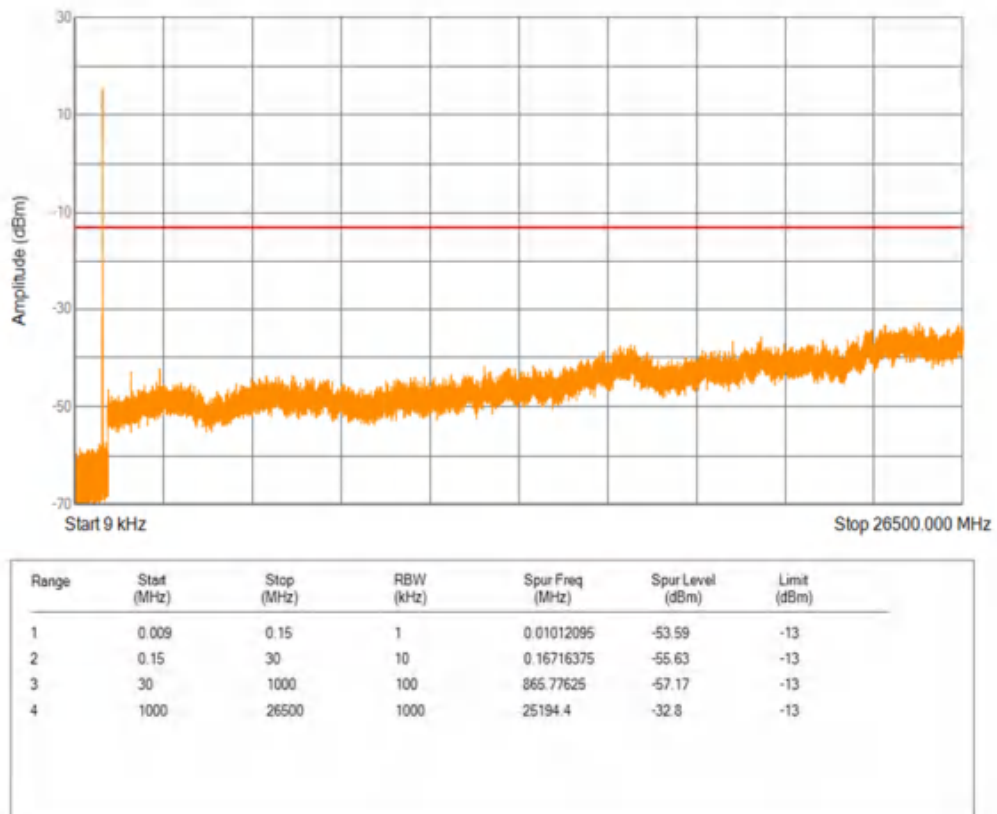
Band5 16QAM BW=5MHz Channel=20425 RB Size=1 Position=#0
