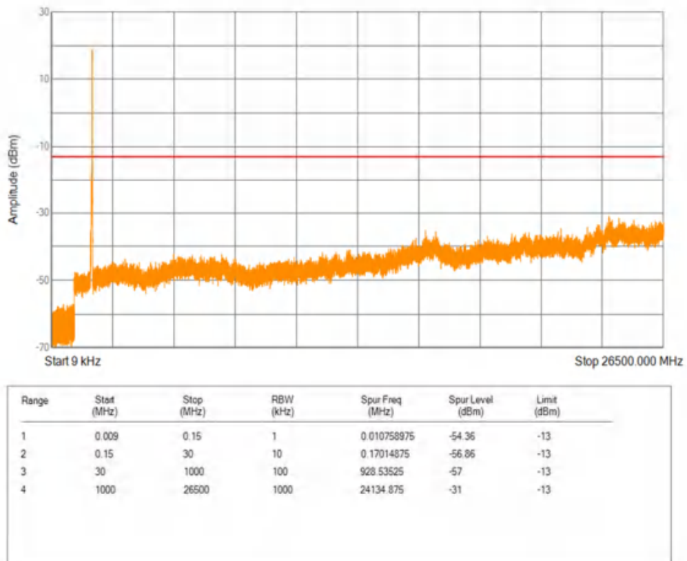
Band66 QPSK BW=3MHz Channel=131987 RB Size=1 Position=#0
