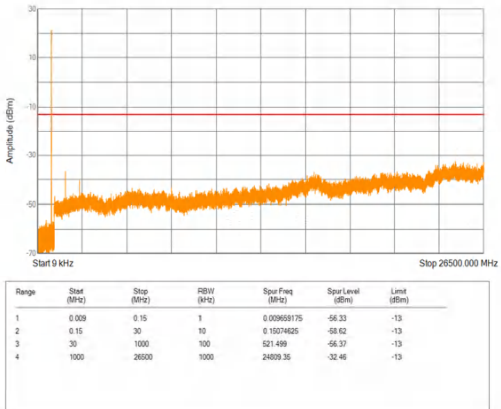
Band5 QPSK BW=1.4MHz Channel=20643 RB Size=1 Position=#0
