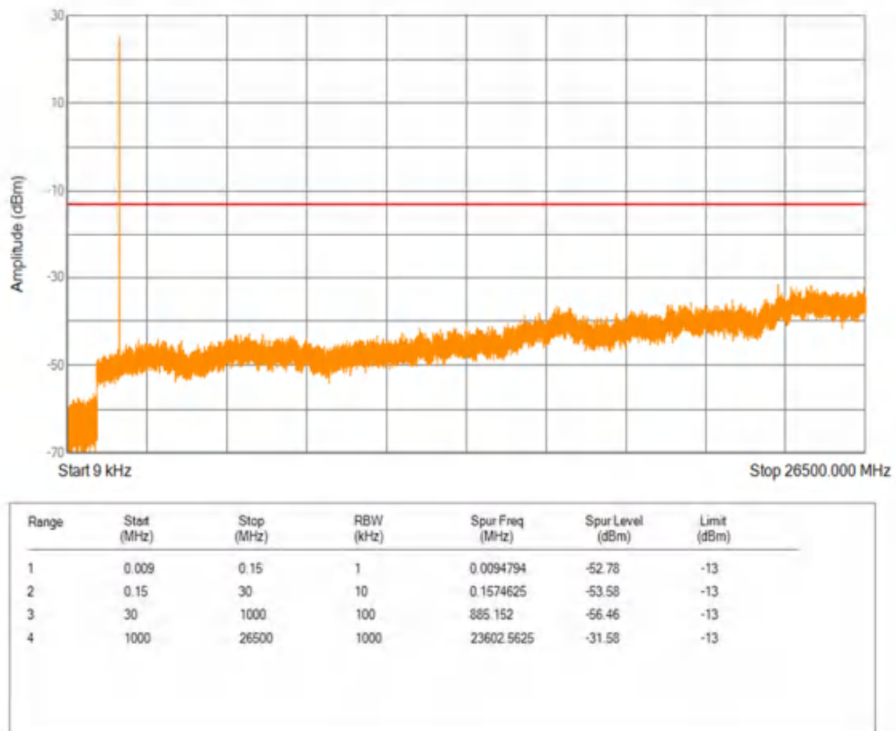
Band66 16QAM BW=1.4MHz Channel=132665 RB Size=1 Position=#0
