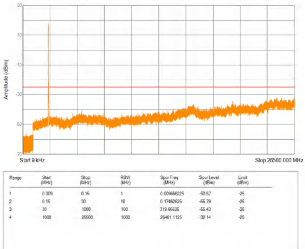
Band7 16QAM BW=20MHz Channel=21350 RB Size=1 Position=#0
