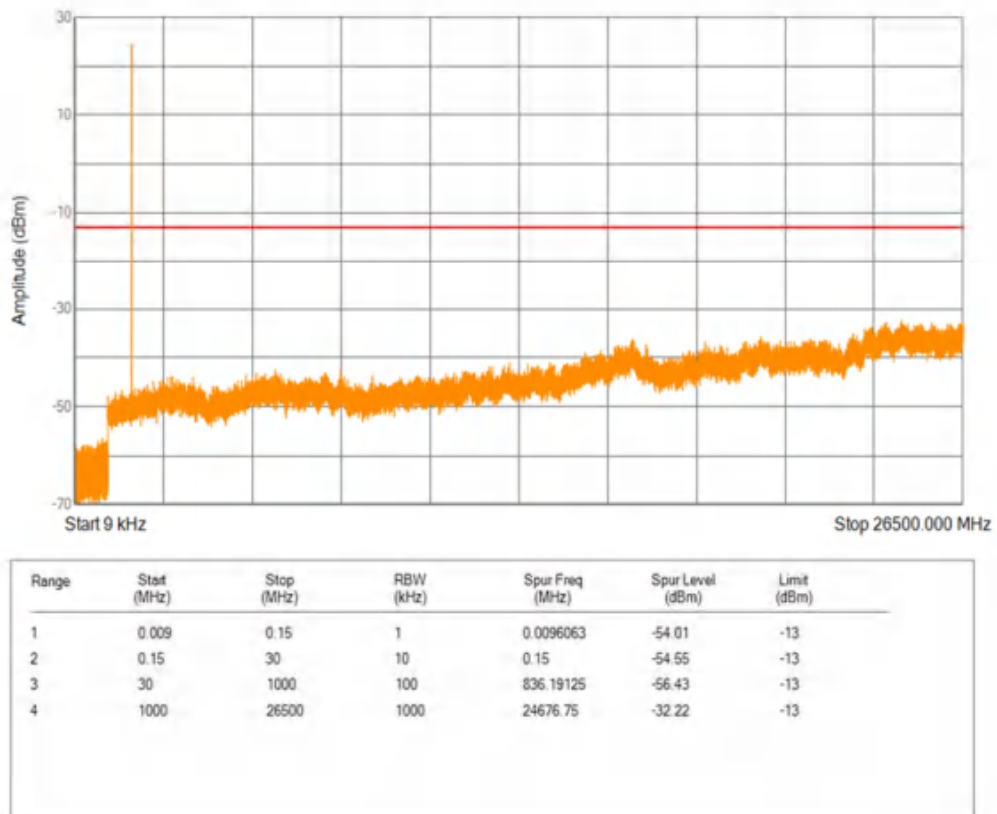
Band66 16QAM BW=1.4MHz Channel=132322 RB Size=1 Position=#0
