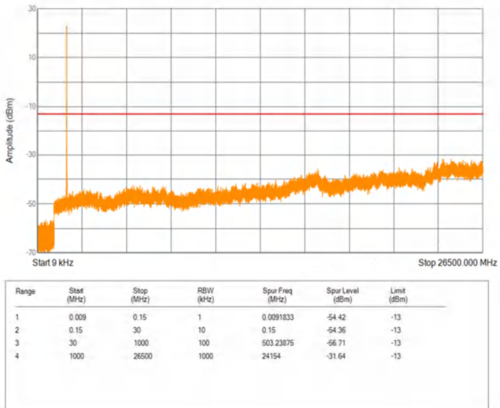
Band66 QPSK BW=5MHz Channel=132647 RB Size=1 Position=#0
