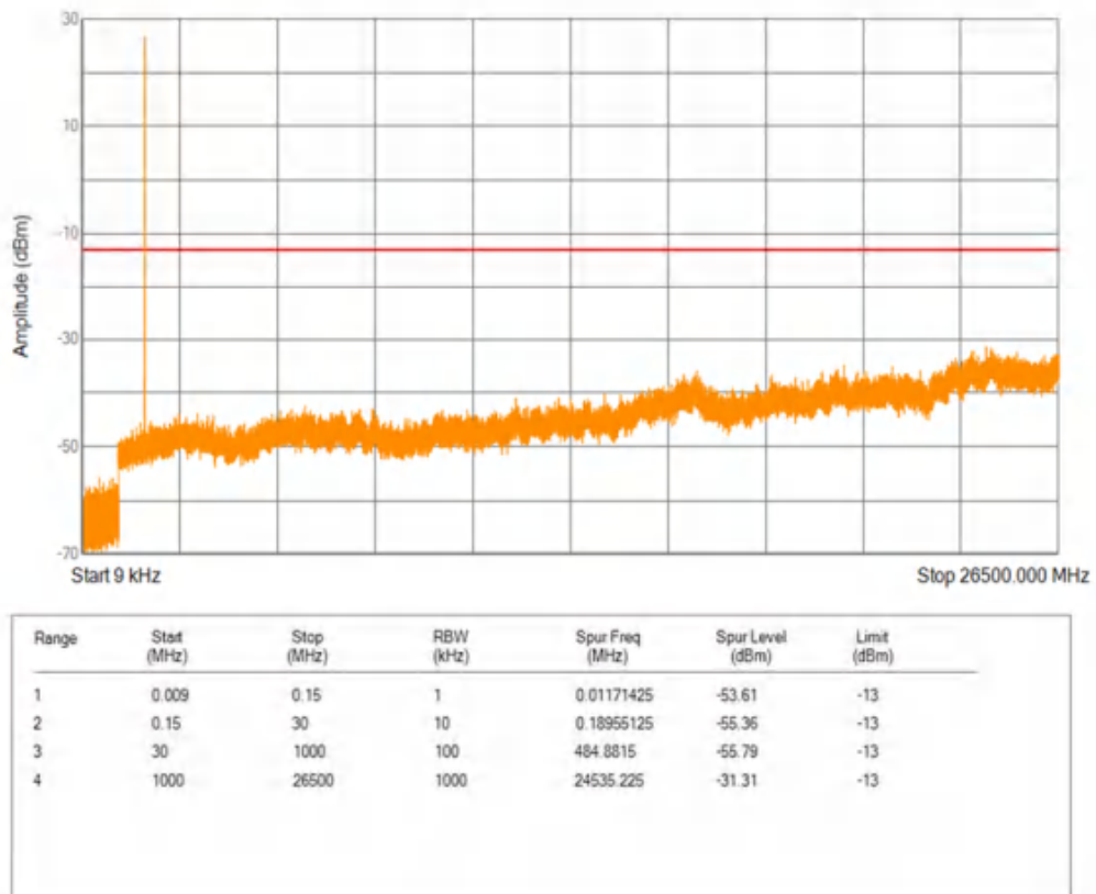
Band66 QPSK BW=1.4MHz Channel=132322 RB Size=1 Position=#0
