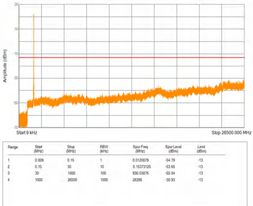
Band66 16QAM BW=10MHz Channel=132622 RB Size=1 Position=#0
