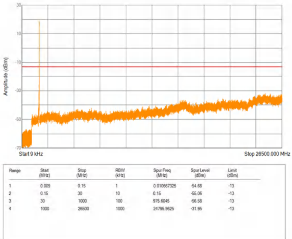
Band66 16QAM BW=20MHz Channel=132072 RB Size=1 Position=#0
