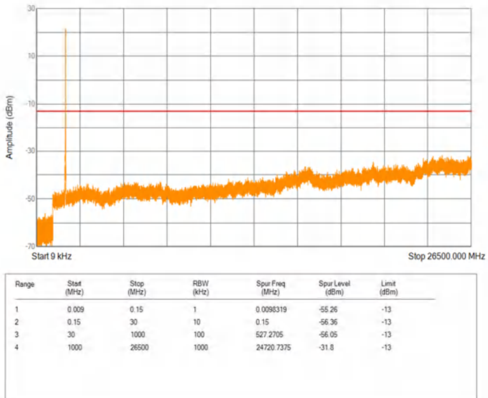
Band66 QPSK BW=15MHz Channel=132047 RB Size=1 Position=#0
