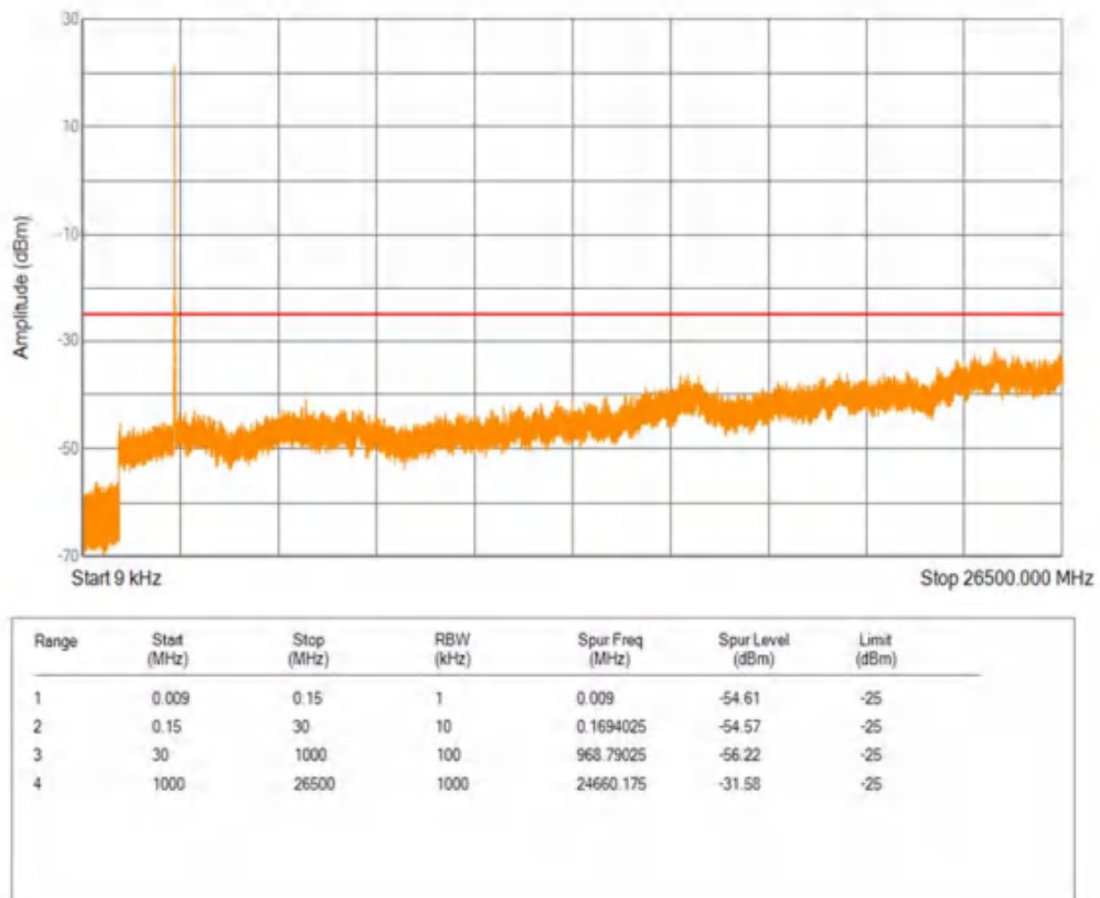
Band7 QPSK BW=10MHz Channel=21400 RB Size=1 Position=#0
