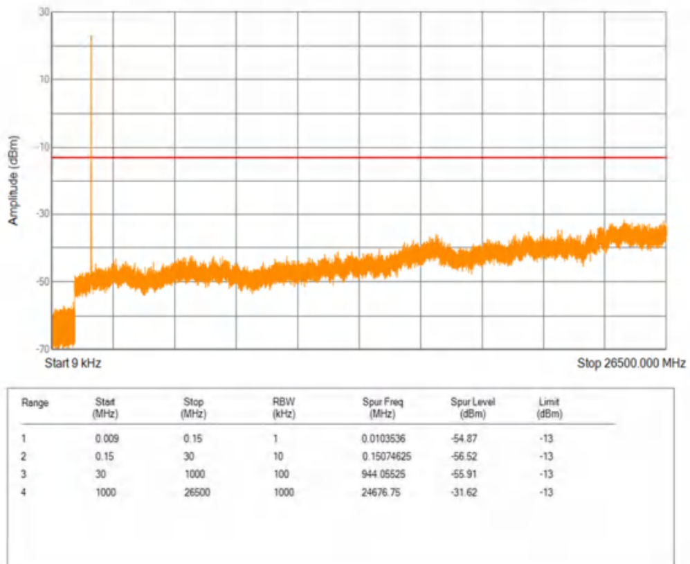
Band66 QPSK BW=5MHz Channel=132322 RB Size=1 Position=#0
