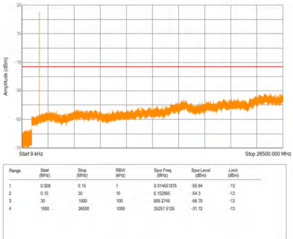
Band66 QPSK BW=10MHz Channel=132022 RB Size=1 Position=#0
