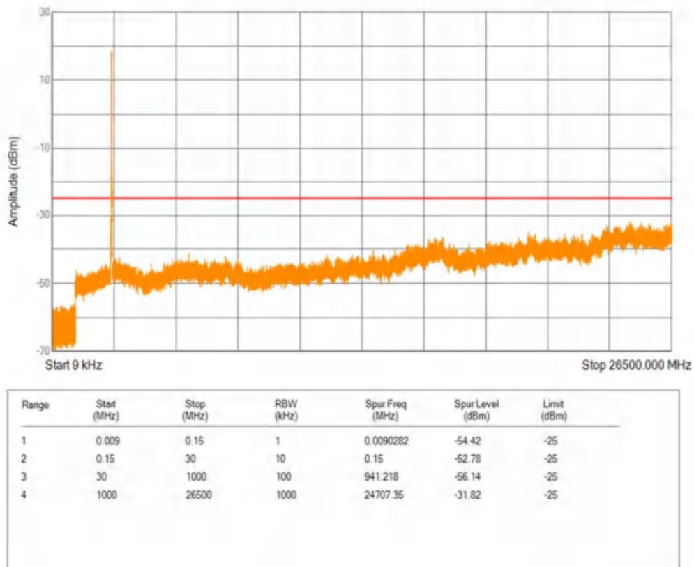
Band7 QPSK BW=5MHz Channel=20775 RB Size=1 Position=#0
