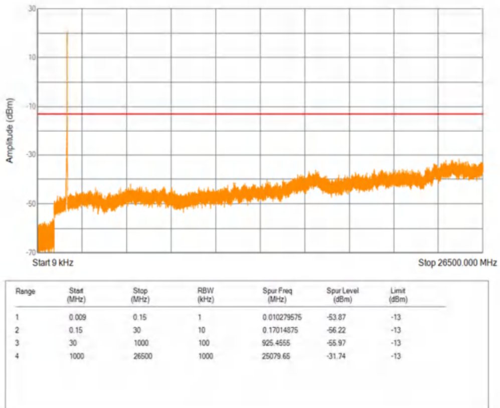
Band66 QPSK BW=20MHz Channel=132072 RB Size=1 Position=#0
