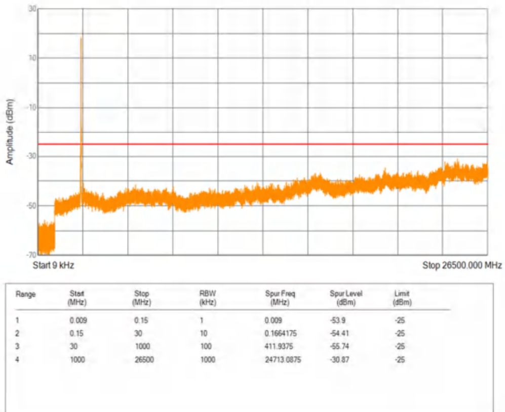
Band7 16QAM BW=5MHz Channel=20775 RB Size=1 Position=#0
