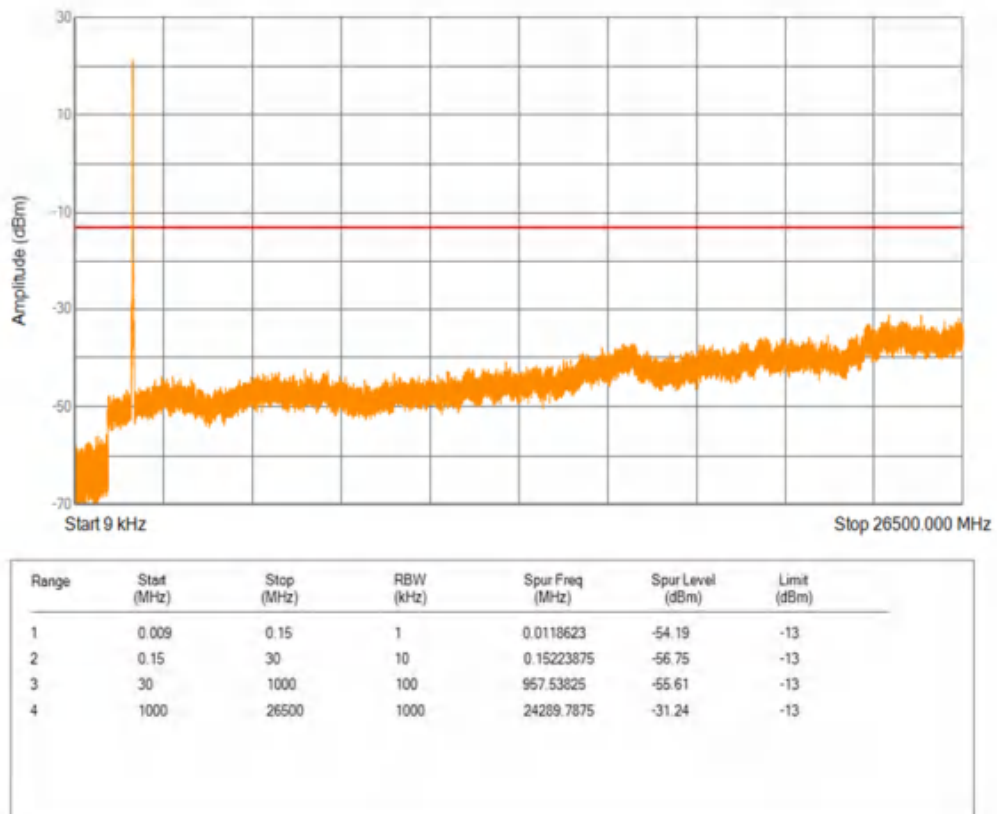
Band66 QPSK BW=15MHz Channel=132597 RB Size=1 Position=#0
