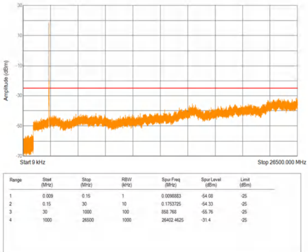
Band7 16QAM BW=15MHz Channel=21375 RB Size=1 Position=#0
