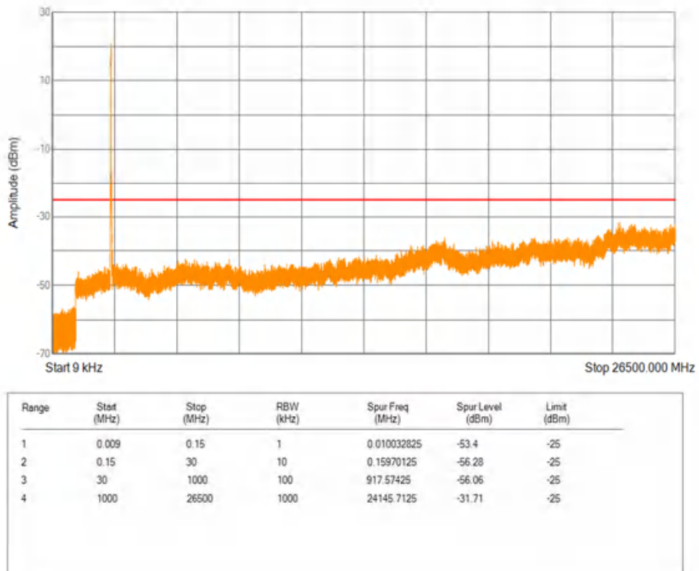
Band41 QPSK BW=20MHz Channel=41490 RB Size=1 Position=#0
