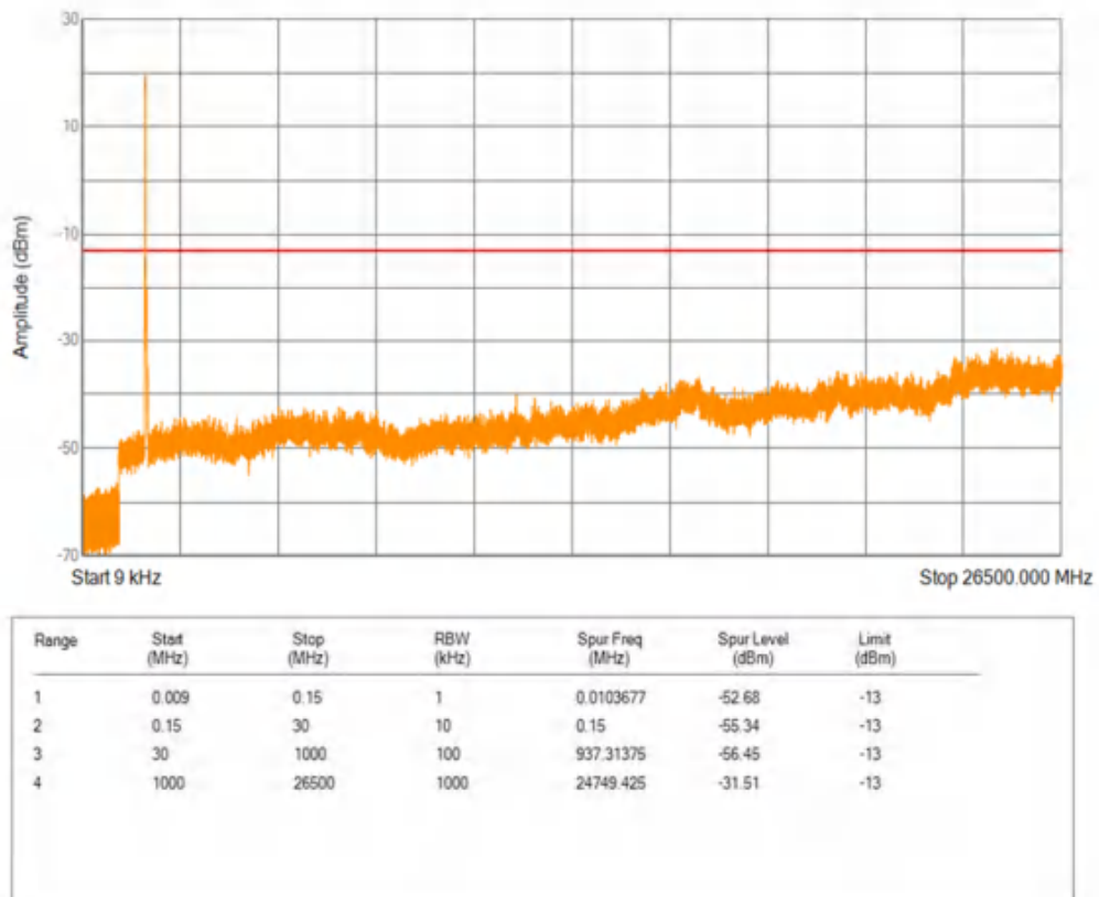
Band66 QPSK BW=20MHz Channel=132322 RB Size=1 Position=#0
