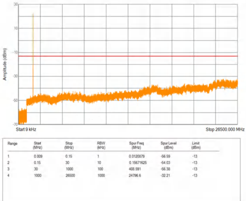
Band66 QPSK BW=1.4MHz Channel=131979 RB Size=1 Position=#0
