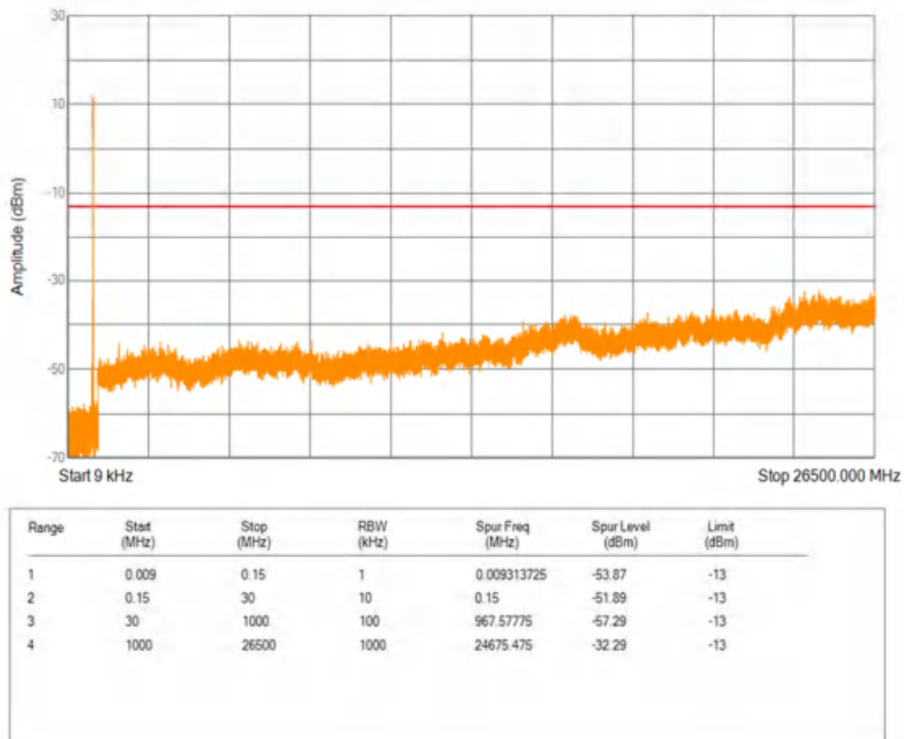
Band5 16QAM BW=3MHz Channel=20415 RB Size=1 Position=#0
