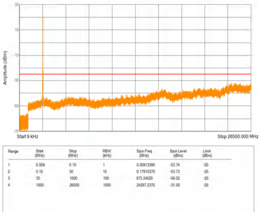
Band5 16QAM BW=1.4MHz Channel=20407 RB Size=1 Position=#0
