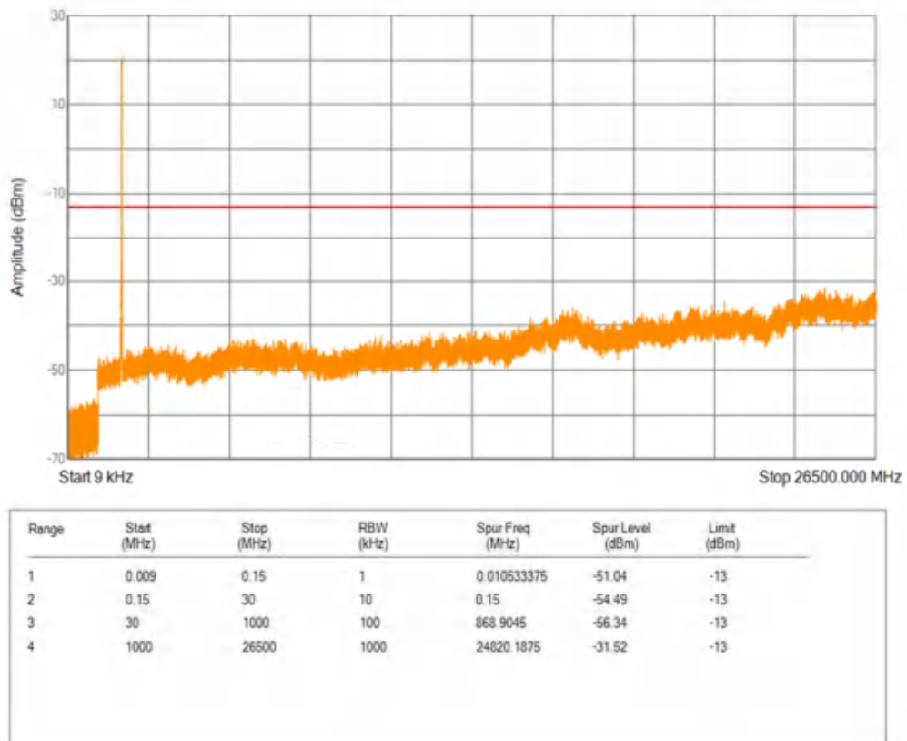
Band66 16QAM BW=15MHz Channel=132047 RB Size=1 Position=#0
