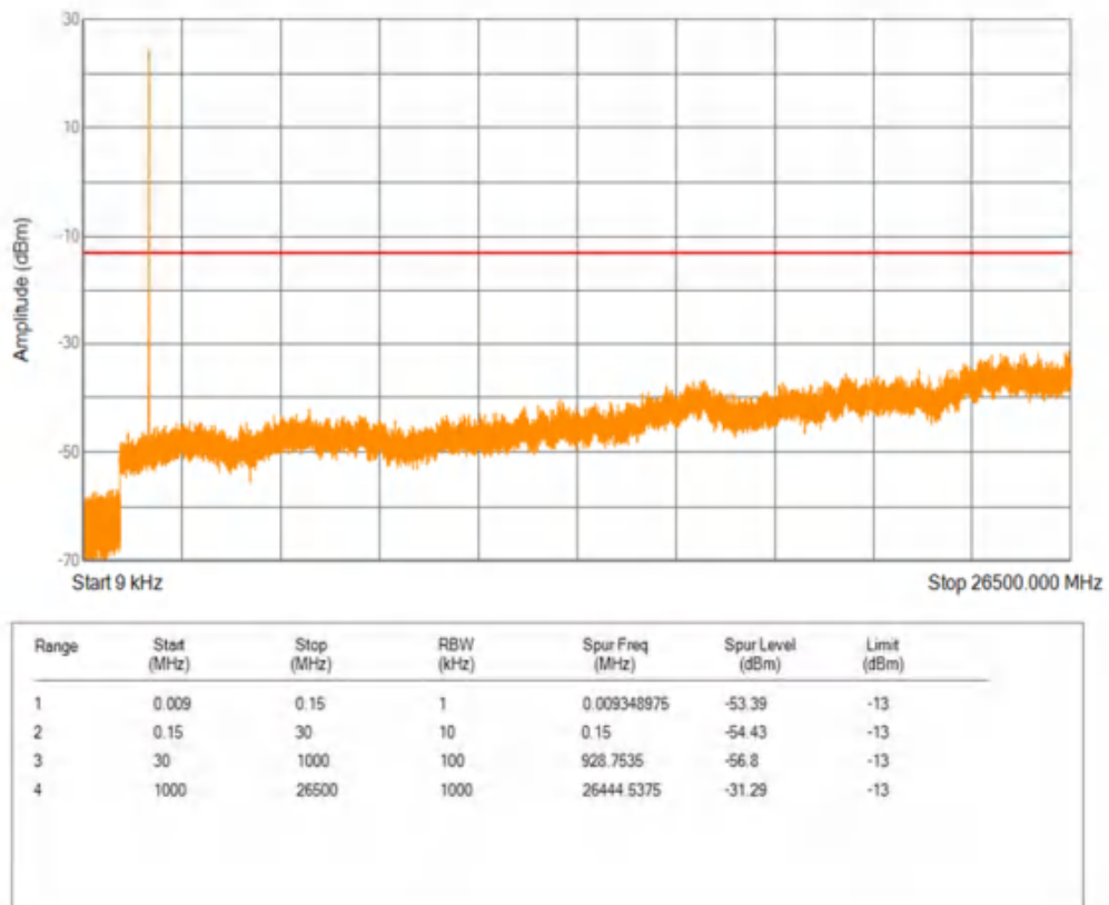
Band66 16QAM BW=5MHz Channel=131997 RB Size=1 Position=#0
