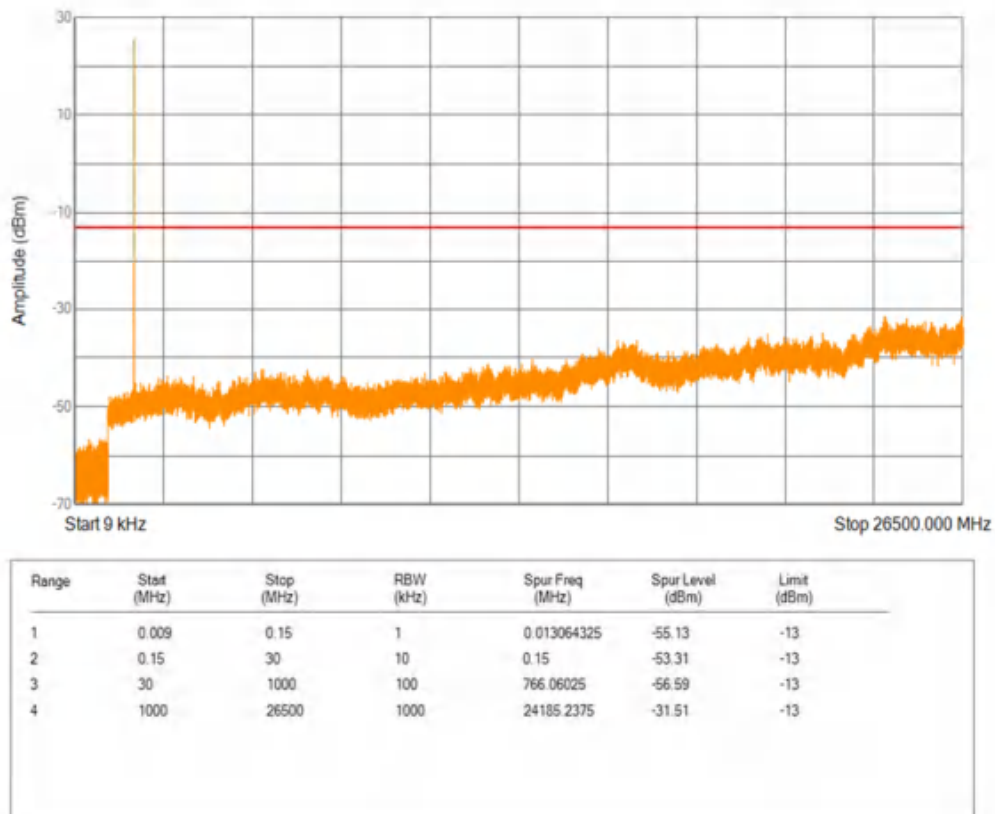
Band66 16QAM BW=10MHz Channel=132022 RB Size=1 Position=#0
