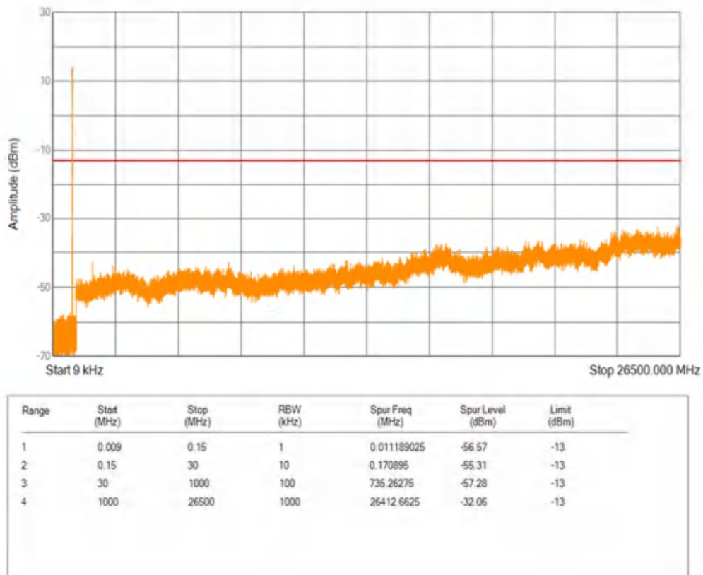
Band5 QPSK BW=1.4MHz Channel=20407 RB Size=1 Position=#0
