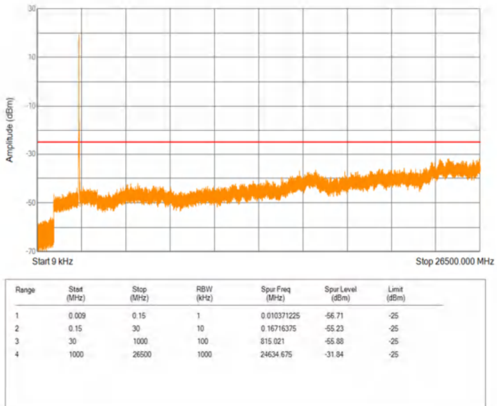
Band41 16QAM BW=20MHz Channel=39750 RB Size=1 Position=#0
