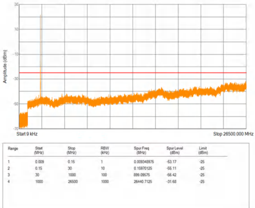
Band7 QPSK BW=5MHz Channel=21425 RB Size=1 Position=#0
