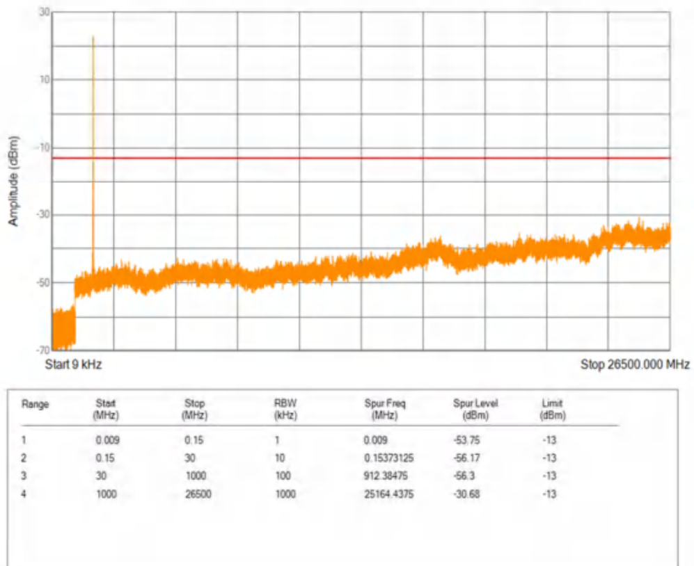
Band7 16QAM BW=10MHz Channel=20800 RB Size=1 Position=#0
