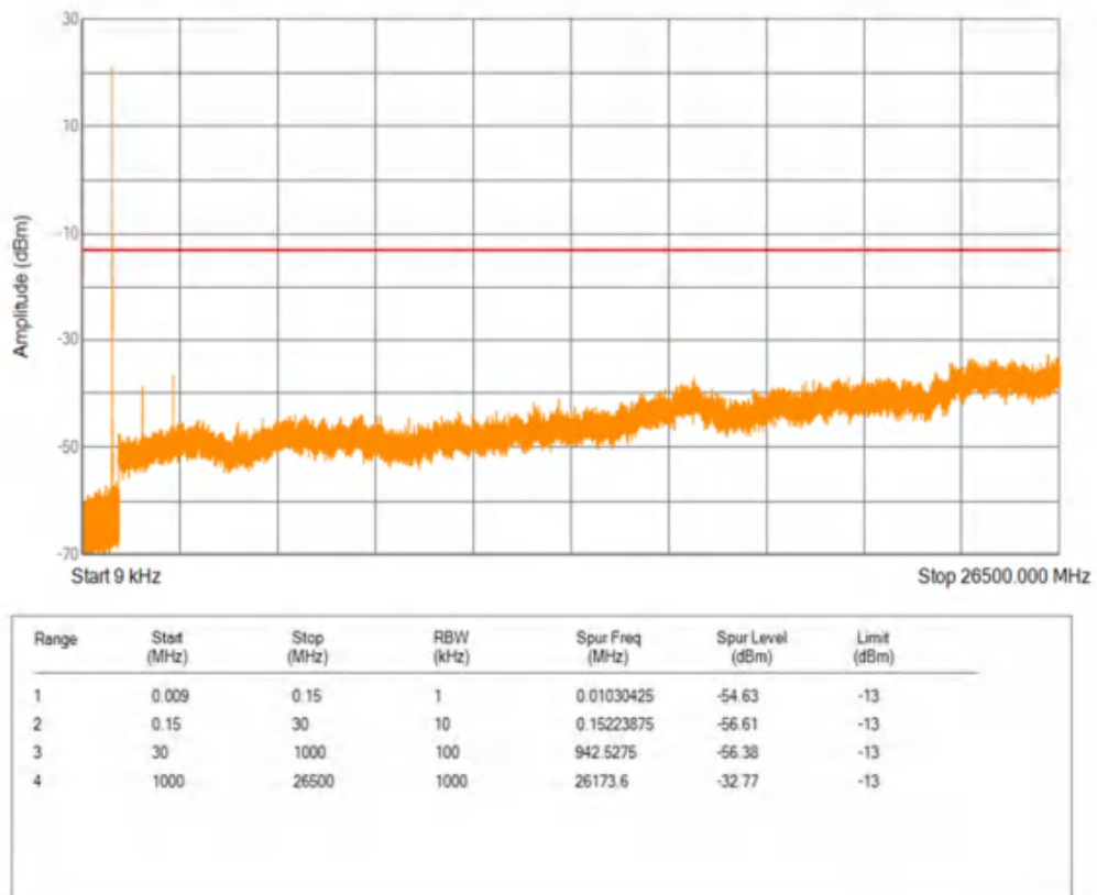
Band5 QPSK BW=1.4MHz Channel=20525 RB Size=1 Position=#0
