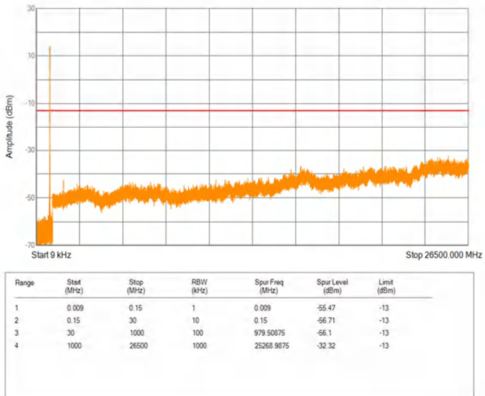
Band5 16QAM BW=5MHz Channel=20625 RB Size=1 Position=#0
