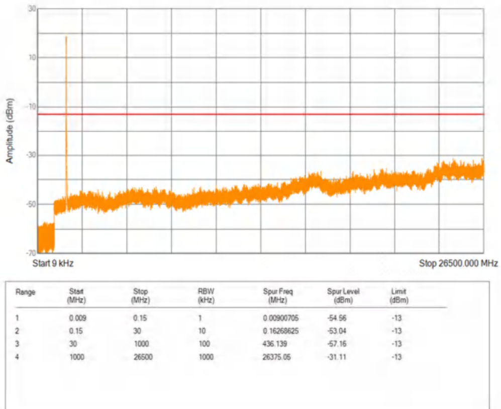
Band66 16QAM BW=15MHz Channel=132322 RB Size=1 Position=#0
