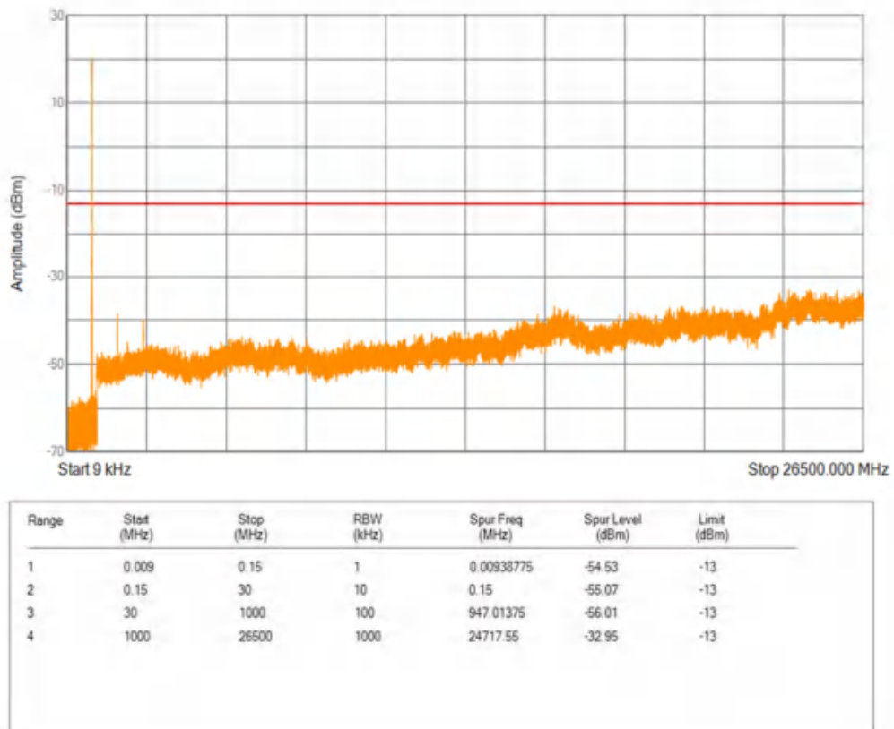
Band5 16QAM BW=10MHz Channel=20450 RB Size=1 Position=#0
