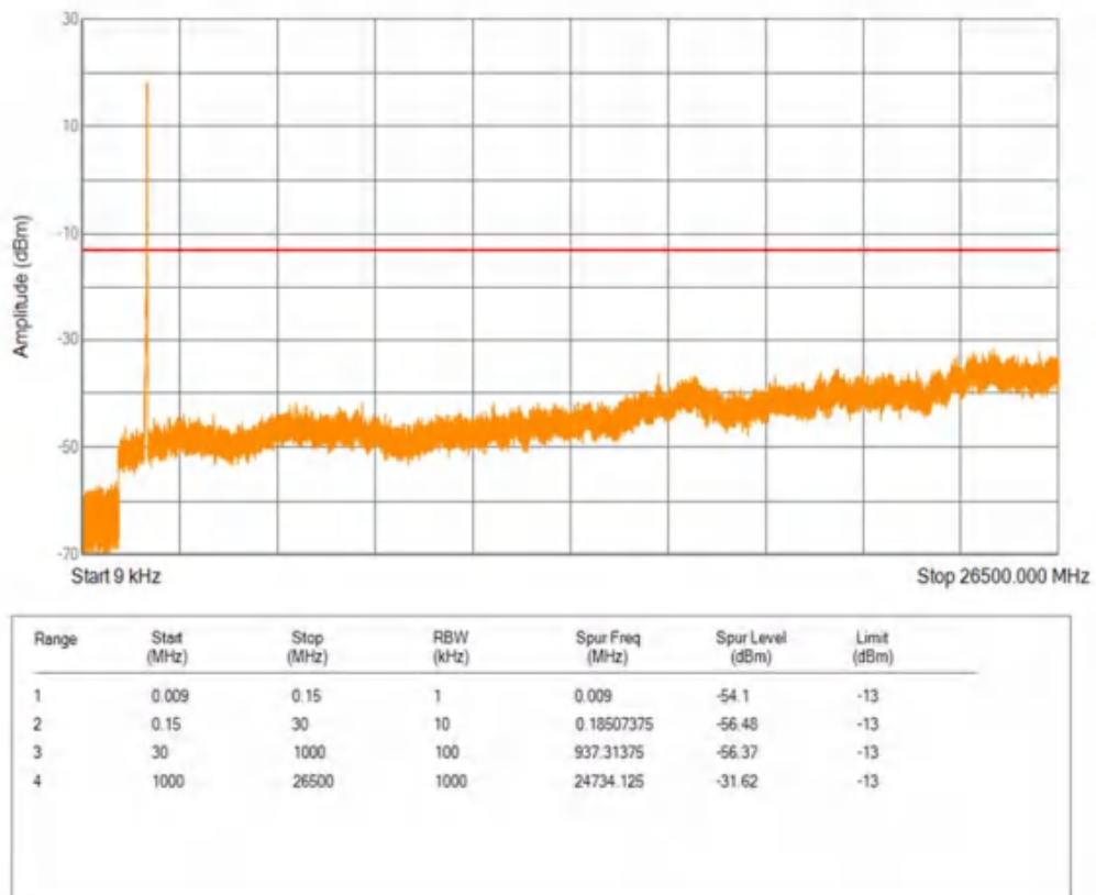
Band66 16QAM BW=3MHz Channel=131987 RB Size=1 Position=#0
