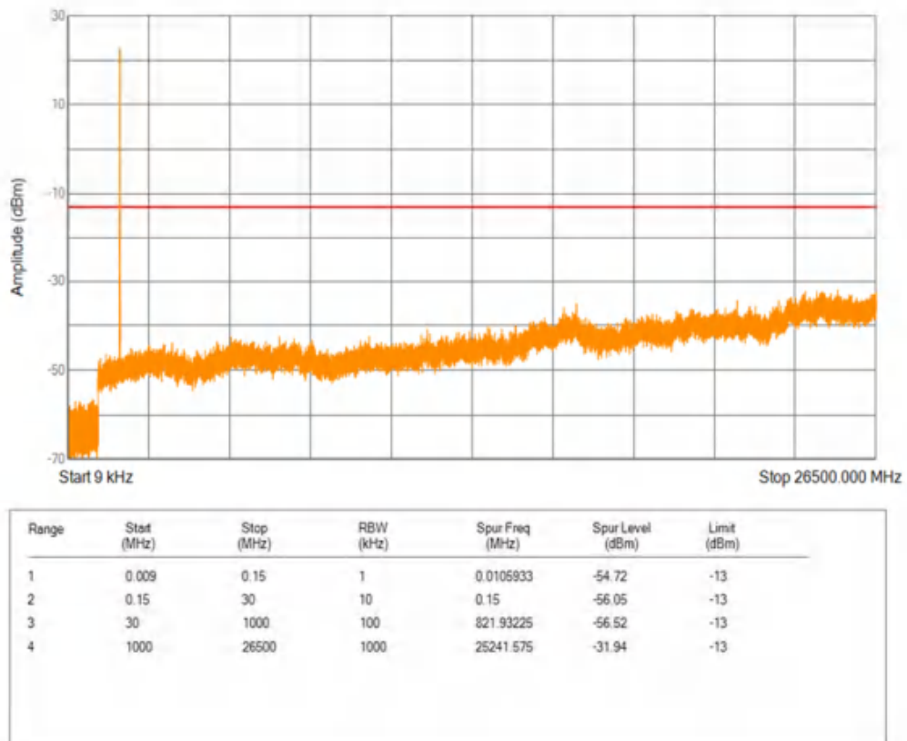
Band66 16QAM BW=5MHz Channel=132322 RB Size=1 Position=#0
