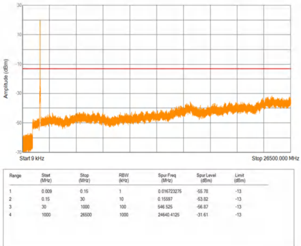
Band66 QPSK BW=20MHz Channel=132572 RB Size=1 Position=#0
