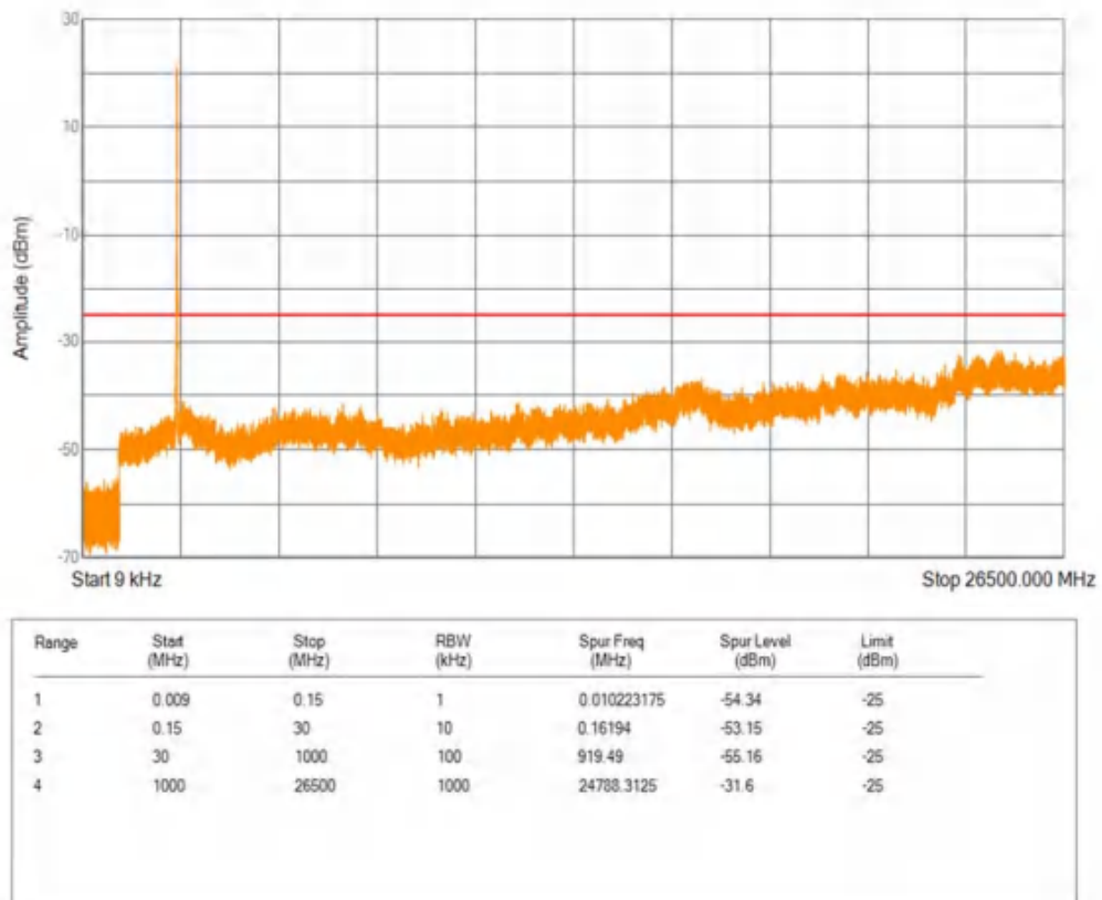
Band7 QPSK BW=20MHz Channel=20850 RB Size=1 Position=#0
