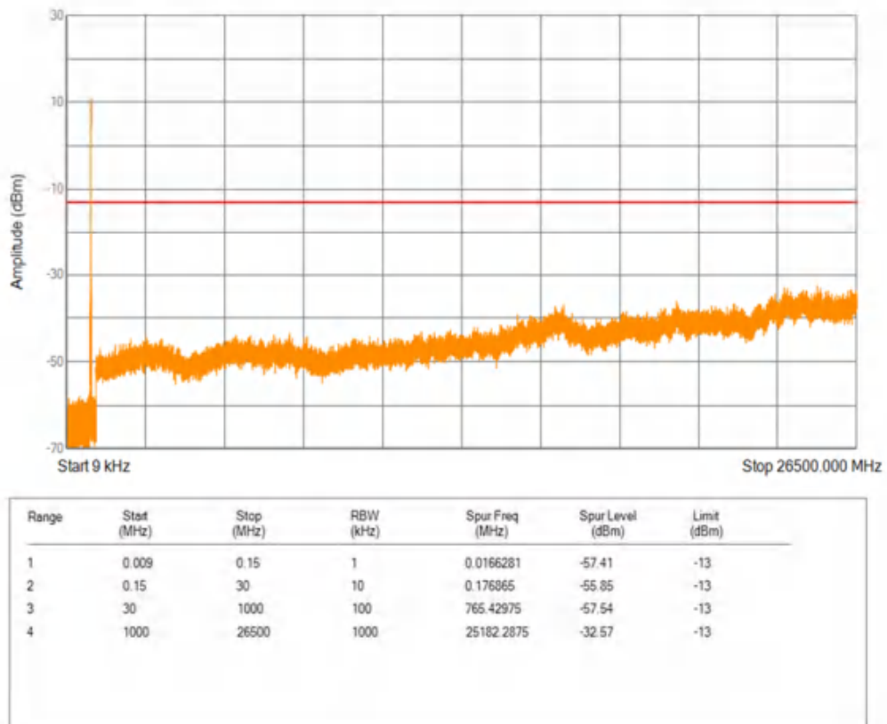
Band5 16QAM BW=10MHz Channel=20525 RB Size=1 Position=#0
