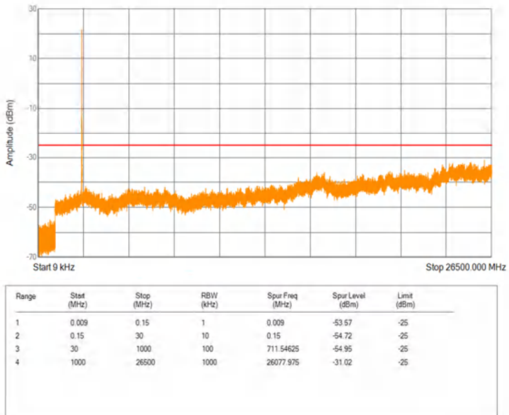
Band7 QPSK BW=15MHz Channel=20825 RB Size=1 Position=#0
