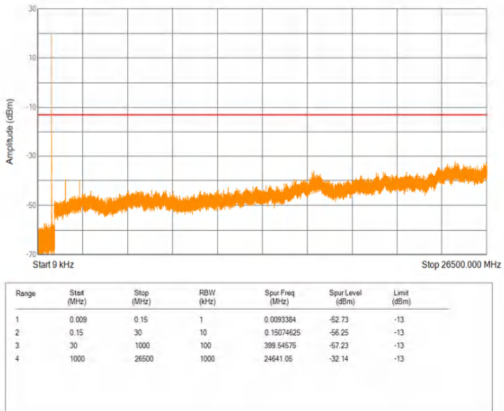
Band5 16QAM BW=1.4MHz Channel=20525 RB Size=1 Position=#0
