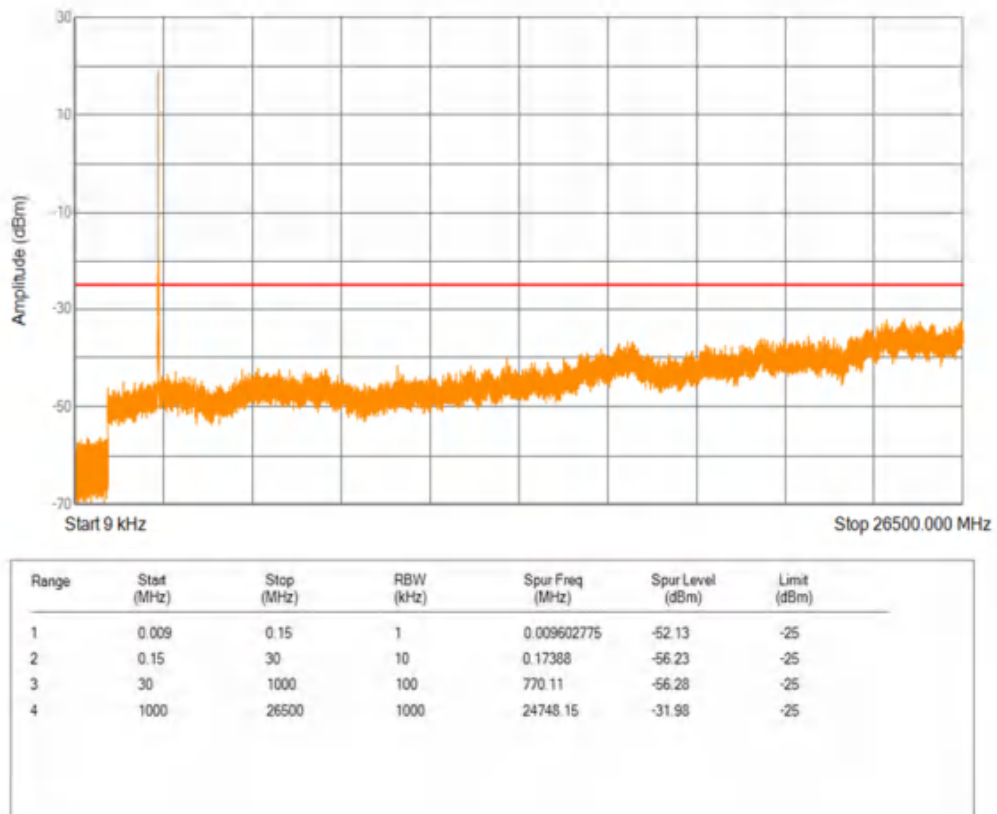
Band7 16QAM BW=10MHz Channel=21400 RB Size=1 Position=#0
