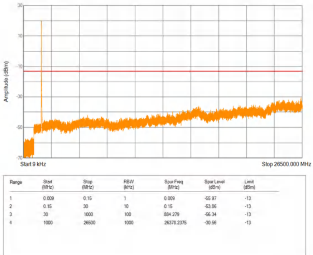
Band66 QPSK BW=15MHz Channel=132322 RB Size=1 Position=#0
