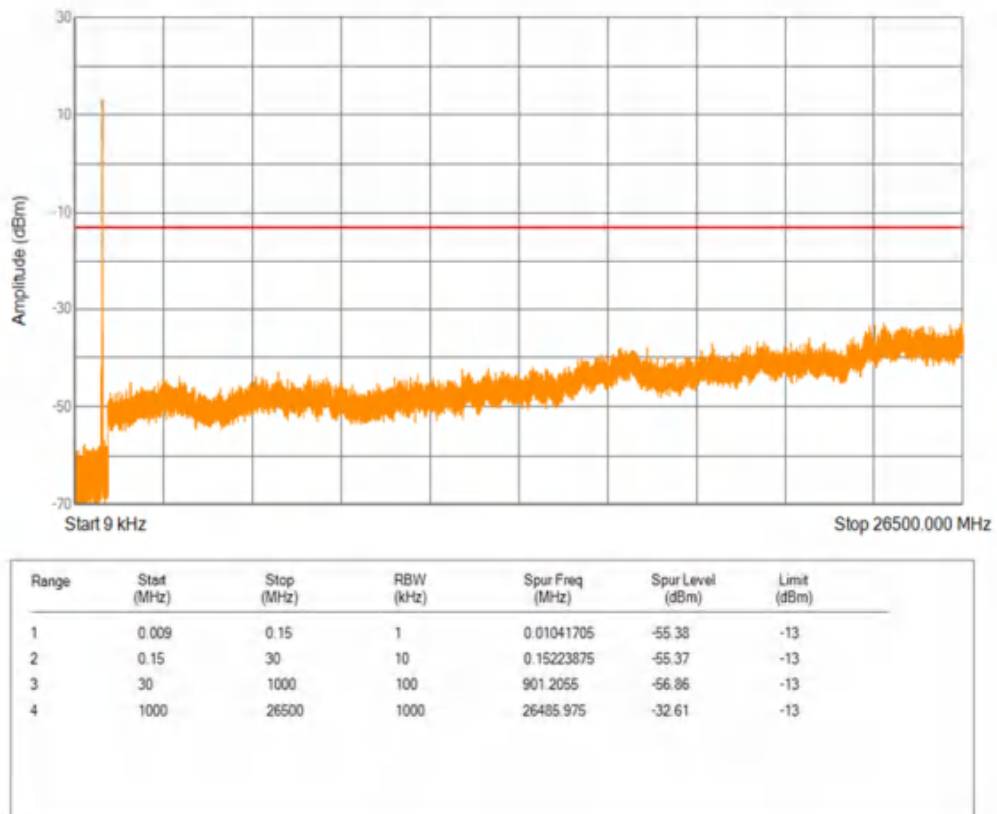
Band5 QPSK BW=10MHz Channel=20600 RB Size=1 Position=#0
