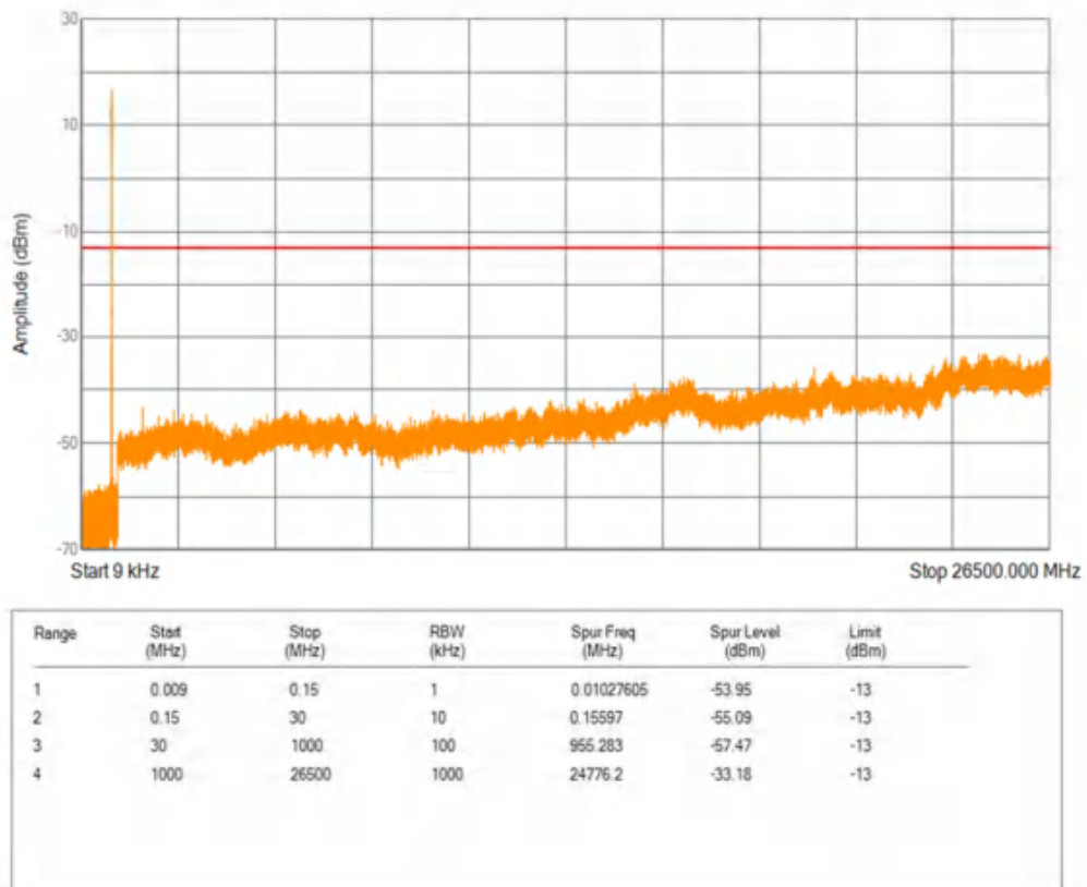
Band66 16QAM BW=1.4MHz Channel=131979 RB Size=1 Position=#0
