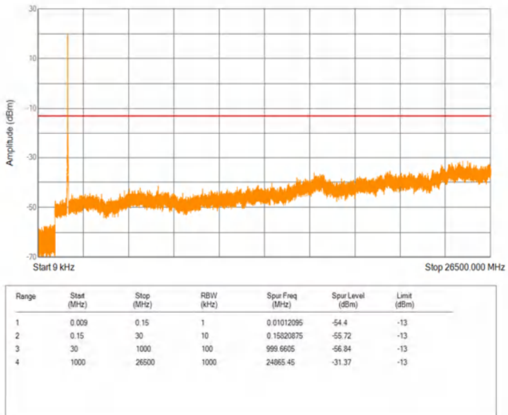
Band66 16QAM BW=15MHz Channel=132597 RB Size=1 Position=#0
