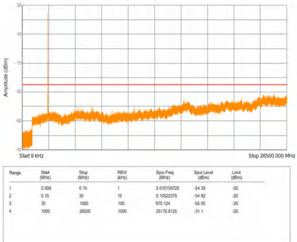
Band7 QPSK BW=10MHz Channel=20800 RB Size=1 Position=#0
