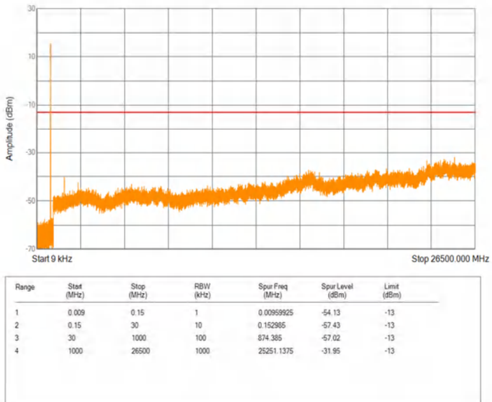
Band5 16QAM BW=3MHz Channel=20635 RB Size=1 Position=#0
