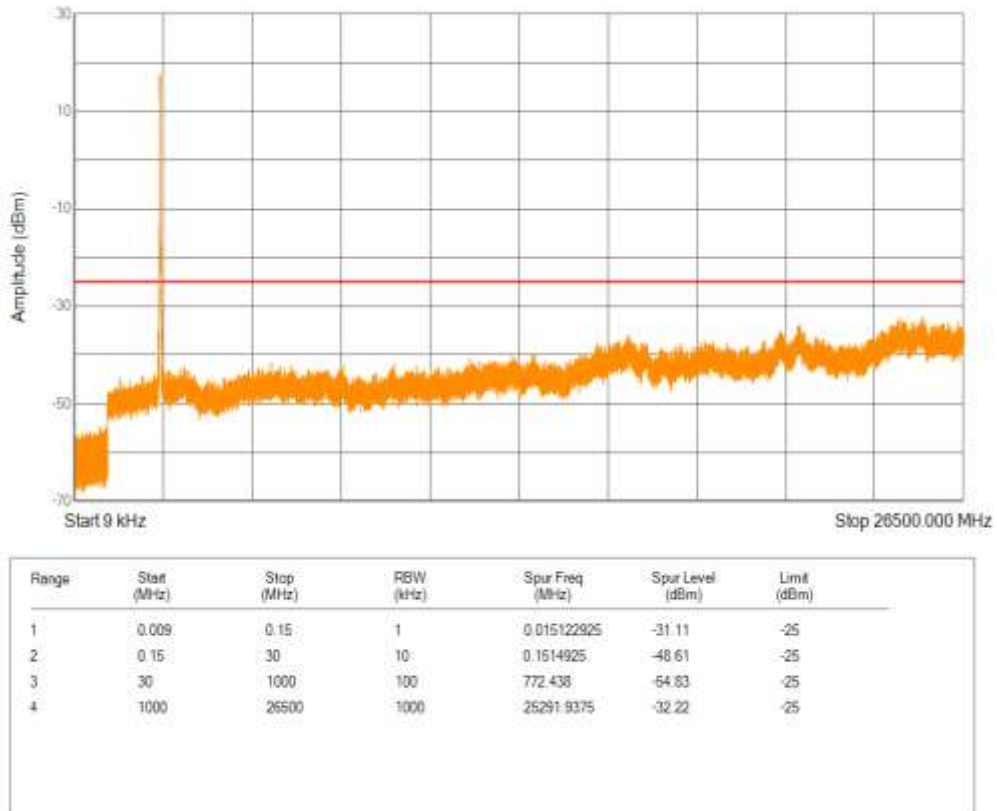
Band41(2555-2655) QPSK BW=20MHz Channel=40740 RB Size=100 Position=#0
