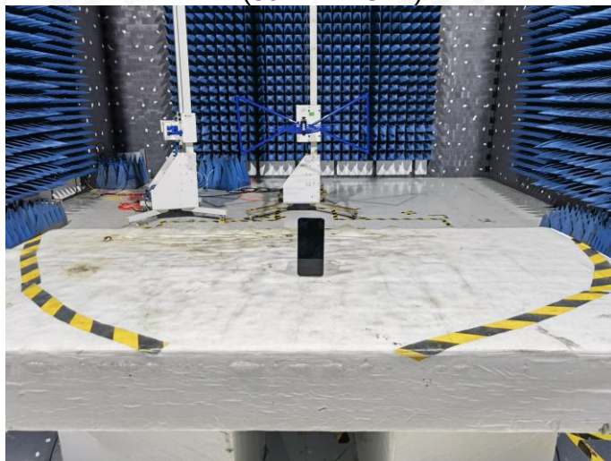
RE (30 MHz-1GHz)
